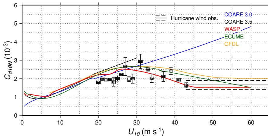
Figure 2. Neutral drag coefficient with respect to 10 m wind speed for different parameterizations (COARE3.0, Fairall et al. (2003); COARE3.5, (Edson et al., 2013); WASP; ECUME (Roehrig et al., 2020) and GFDL (Chen et al., 2020)) and summary of observations up to 60 \text{ m s}^{-1} .
