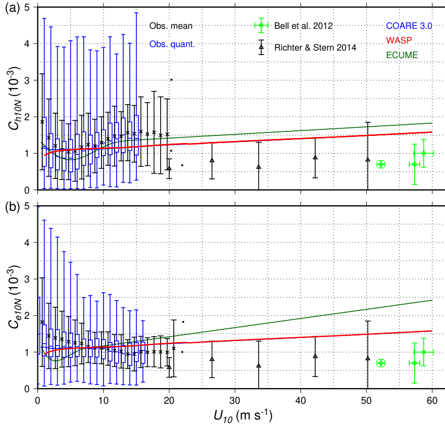
Figure 3. Neutral coefficient for sensible (a) and latent (b) heat fluxes at 10 m with respect to 10 m wind speed for different parameterizations (COARE3.0, (Fairall et al., 2003), blue line; WASP, red line; and ECUME, (Roehrig et al., 2020), dark green line) and in situ eddy covariance observations and estimates up to 60 \text{ m s}^{-1} (see text). Note that WASP and COARE3.0 are almost superimposed. Black and blue symbols as in Fig. 1.
