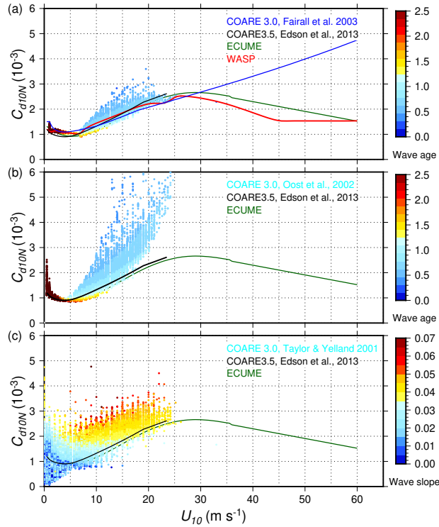
Figure 4. Neutral drag coefficient with respect to 10 m wind speed for the parameterizations implemented in SURFEX v8.1 (a) (COARE 3.0, (Fairall et al., 2003); COARE3.5, (Edson et al., 2013), ECUME (Roehrig et al., 2020), and WASP (present study)), COARE 3.0 with dependence on the wave age (b - color scale, (Oost et al., 2002)) and COARE 3.0 with dependence on the wave steepness (c - color scale, (Taylor and Yelland, 2001)). The surface data used to compute the drag coefficient with wave impact in (a, b, c) are the hourly observations of the LION moored Météo-France buoy (centre of the Gulf of Lion) between 2001 and 2014.
