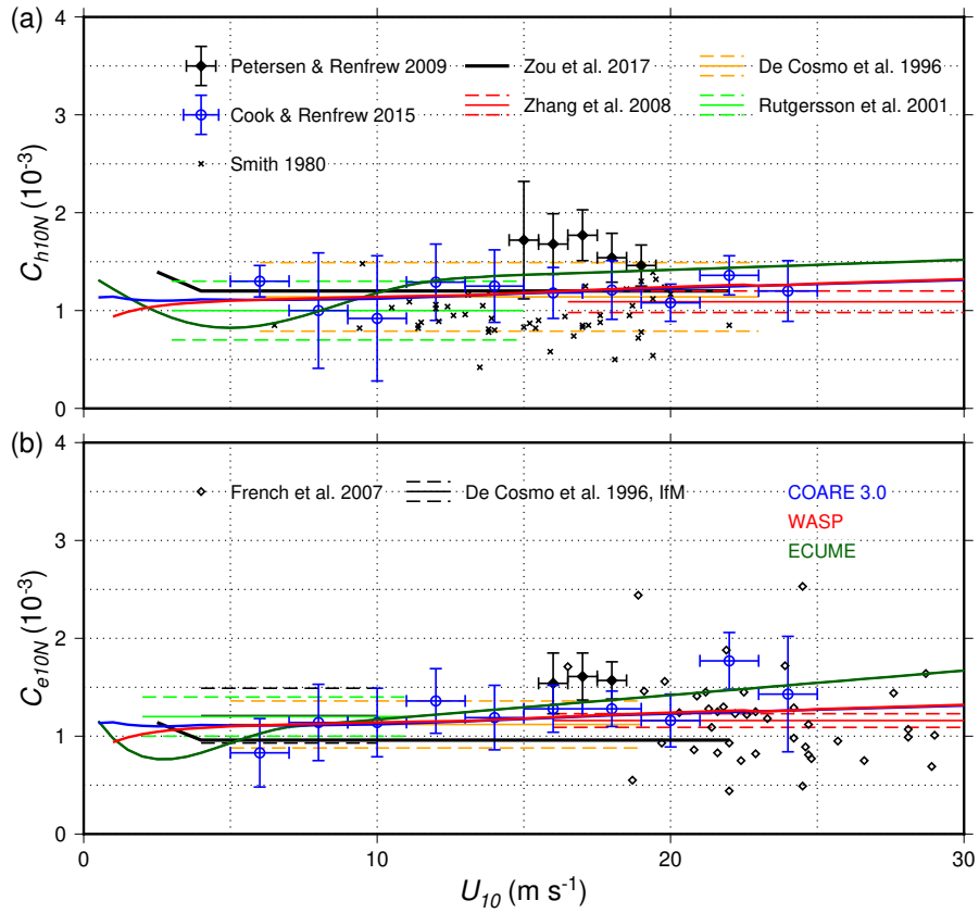
Figure B1. Sensible (a) and latent (b) heat transfer coefficients with respect to 10 m wind speed for different parameterizations (COARE3.0, (Fairall et al., 2003); ECUME (Roehrig et al., 2020) and WASP) in comparison with additional observations (see Table B2) up to 28 m s^{-1} .
