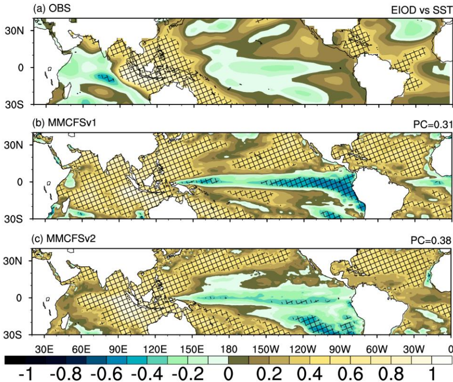
Figure 16: Correlation between SST over the eastern IOD box ( 10^{\circ} S to equator, 90-110^{\circ} E) and tropical SSTs anomalies 470 during JJAS. (a) Observations (ERSST), (b) MMCFSv1, and (c) MMCFSv2. The hatching shows statistically significant at 95 % confidence level.
