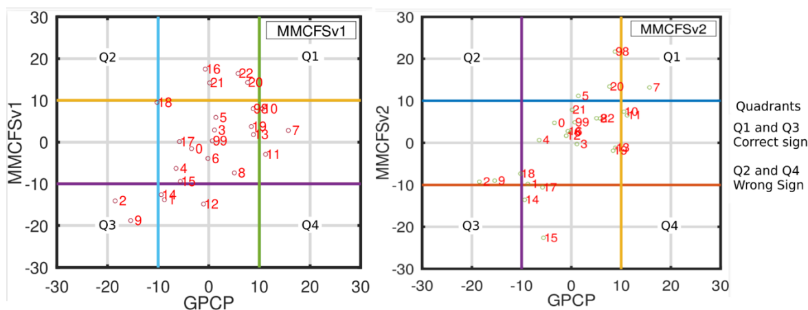
345 Figure 12. Scatter plot of ISMR anomaly (percentage) from GPCP (x-axis), and MMCFS (y-axis), left panel is MMCFSv1 and right panel is MMCFSv2.
