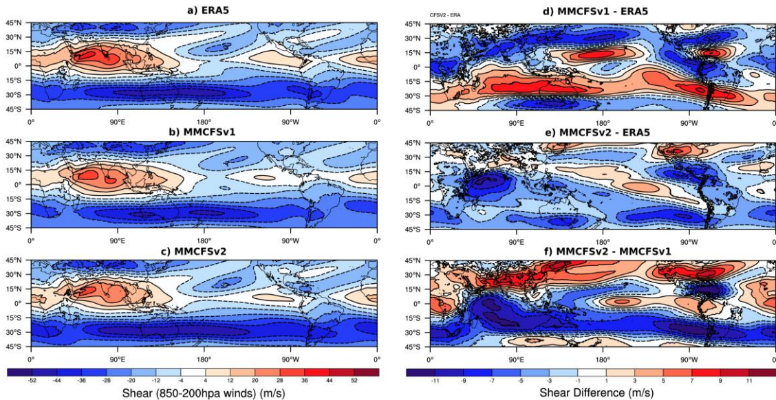
Figure 10: JJAS seasonal mean easterly wind shear (U850–U200, m/s) in (a) observations (ERA5) (b) MMCFSv1, and (c) MMCFSv2. Seasonal mean easterly wind shear biases (model-observation) in (d) MMCFSv1 (e) MMCFSv2. (f) Difference in simulated seasonal mean easterly wind shear between MMCFSv2 and MMCFSv1 hindcast runs. Dashed contours are used for negative values while solid contours are positive values.
