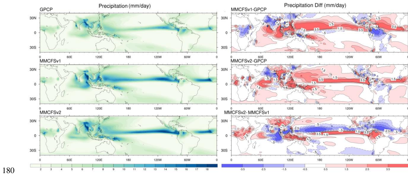
Figure 2: JJAS mean Rainfall (a) GPCP(b) MMCFSv1 (c) MMCFSv2, and bias (d) MMCFSv1-GPCP (e) MMCFSv2-GPCP, and (f) Difference between MMCFSv1 and MMCFSv2. Dashed contours are used for negative difference, while positive contours are solid.
