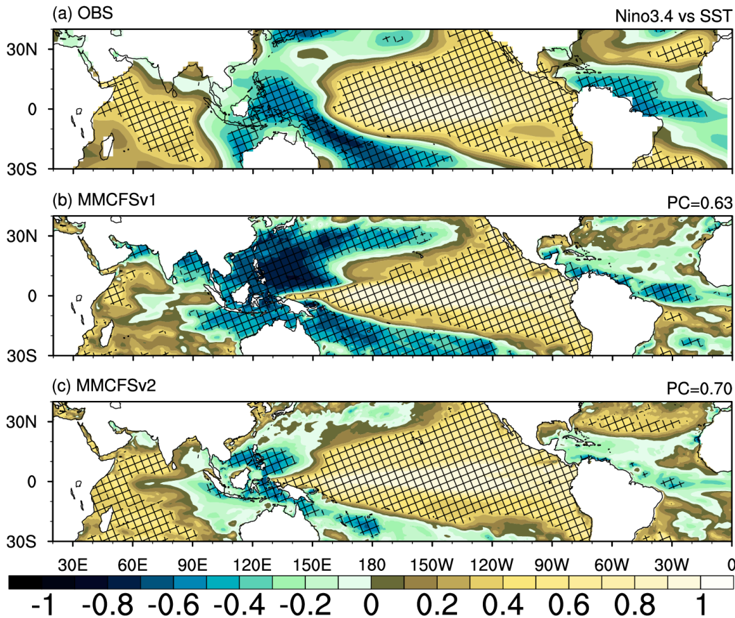
Figure 14: Correlation between JJAS Nino 3.4 (index) SST anomalies and Tropical SST anomalies in (a) Observations (ERSST), (b) MMCFSv1, and (c) MMCFSv2. The hatching shows statistical significance at 95 % confidence level.
