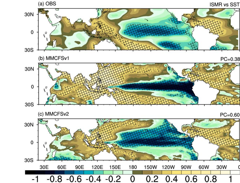
Figure 18: Correlation between ISMR and global SST anomalies. (a) Observations (ERSST), (b) MMCFSv1, (c) MMCFSv2. The hatching shows statistically significant at a 95% confidence level.
