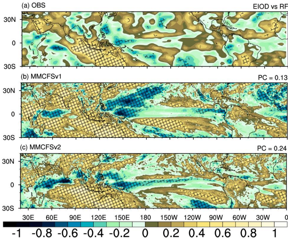
Figure 17: Correlation between the SST anomalies over the eastern equatorial Indian Ocean (index) and rainfall anomalies over the tropical regions. (a) Observations (GPCP), (b) MMCFSv1, and (c) MMCFSv2. The hatching shows statistical significance at 95 % confidence level.
