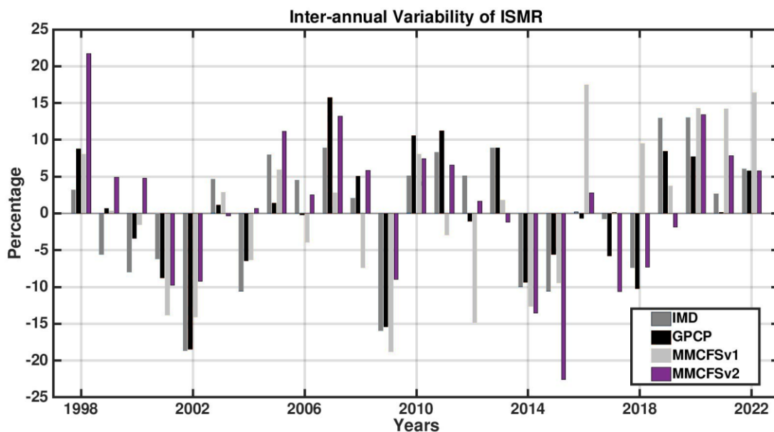
Figure 11: Interannual Variability of area averaged rainfall over Indian land mass from model hindcast (MMCFSv2, MMCFSv1) and different observational datasets (IMD and GPCP).
