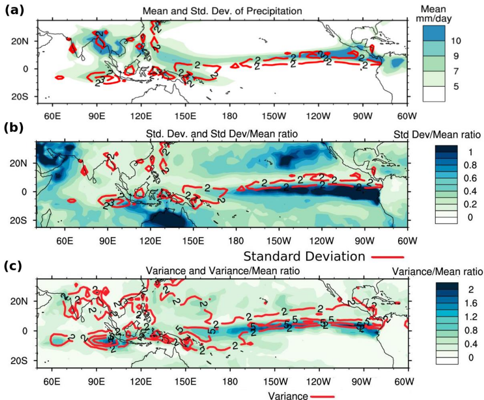
Figure 1: (a) JJAS climatological mean precipitation (shading) and standard deviation (contours) (b) Standard deviation (red contour) and standard deviation to mean ratio (shading) (c) Variance (red contour) and variance to mean ratio of precipitation (shading) from 41 years (1981-2021) of GPCP data.
