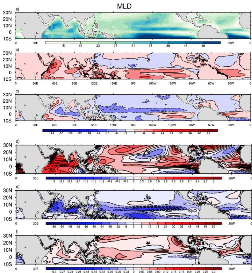
Figure 6. a) Mixed Layer Depth from C-GLORS, b) and c) Model bias of MLD from C-GLORS, d) SST difference between v2 and v1 ( v_2-v_1 ) e) MLD difference ( v_2-v_1 ) f) Qnet contribution to MLD. Dashed contours are used to highlight negative values.
