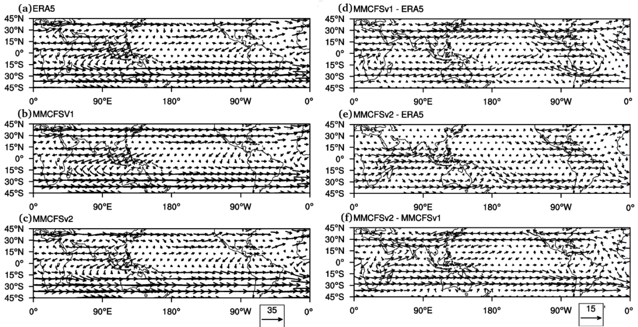
Figure 8: JJAS climatological mean winds (m/s) 200 hPa (a) ERA5 (b) MMCFSv1 (c) MMCFSv2, and bias (d) MMCFSv1-ERA5 (e) MMCFSv2-ERA5, and (f) Difference between MMCFSv2 and MMCFSv1.
