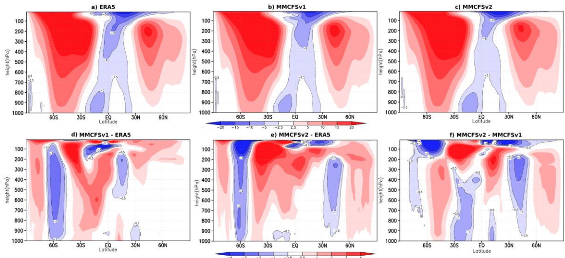
Figure 9: JJAS climatological zonal mean wind (m/s) (a) ERA5 (b) MMCFSv1 (c) MMCFSv2, bias (d) MMCFSv1-ERA5 (e) MMCFSv2-ERA5, and (f) Difference between MMCFSv1 and MMCFSv2. Negative contours are highlighted with contour lines.
