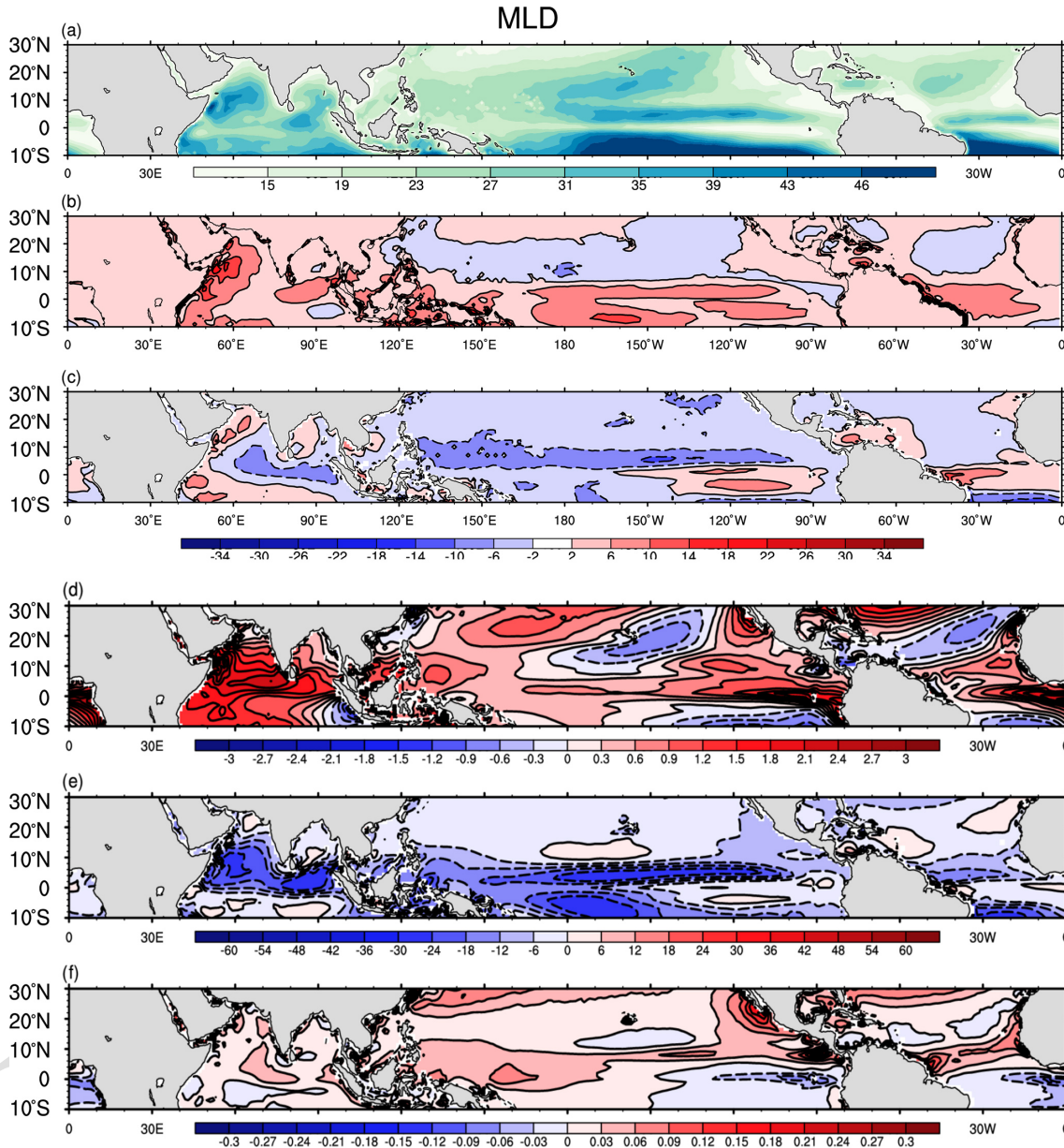
Figure 6. Panel (a) shows mixed layer depth from C-GLORS, and (b) and (c) show model bias of MLD from C-GLORS. Panel (d) shows the SST difference between v_2 and v_1 ( v_2 - v_1 ). Panel (e) shows the MLD difference ( v_2 - v_1 ) and (f) shows the Q_{net} contribution to MLD. Dashed contours highlight negative values.
