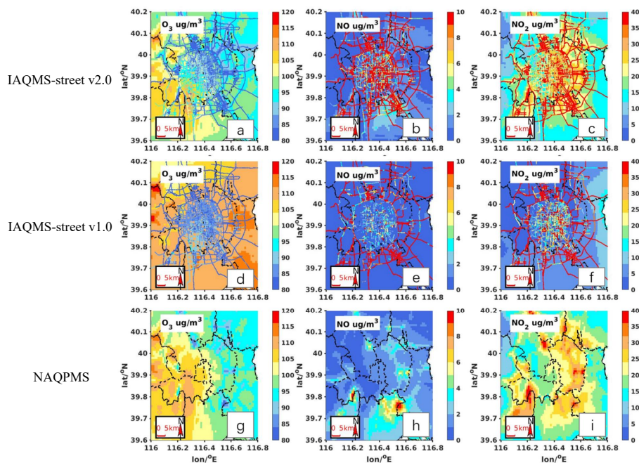
Figure 8. Spatial distribution of the monthly averaged O_3 , NO, and NO_2 concentrations (unit: \mu g/m^3 ) at the urban-street-network scale during August 2021 simulated by the IAQMS-street v2.0 (a–c), IAQMS-street v1.0 (d–f), and NAQPMS (g–i).
