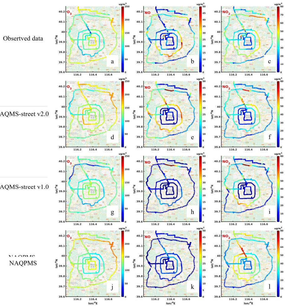
310 Figure 9. Horizontal distributions of the observed O 3 concentration (a), NO concentration (b), and NO 2 concentration (c)- at the street scale and simulation results by the two-way coupled model in IAQMS-street v2.0 (d-f), IAQMS-street v1.0 (g-i), and NAQPMS (j-l) (Imagery © 2022 Google, map data © 2022 Google).
