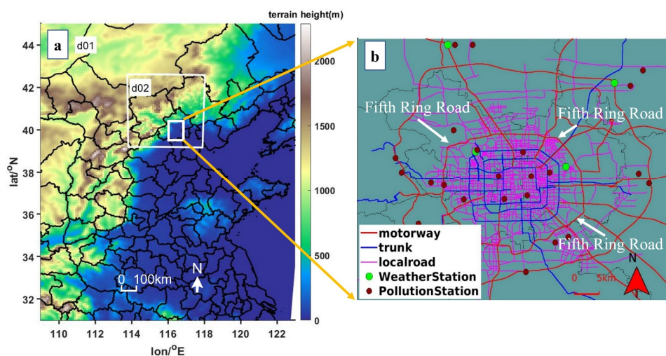
Figure 2. (a). Simulation domains at regional scale: the largest domain 1 (d01) covers the middle and east of China with a horizontal grid spacing of 9 km, an inner domain (d02) covers Beijing and surround areas with a horizontal grid spacing of 1 km. (b). The modelling area and street network in the street-scale model. Green and brown points indicate the locations of urban monitoring stations.
