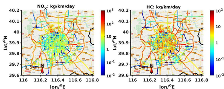
Figure 5. Horizontal distributions of the \text{NO}_x and HC emissions (unit: kg/km/day) at the street-network in Beijing urban and suburban area during August 2021 (Imagery © 2022 Google, map data © 2022 Google).
