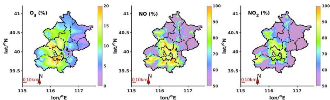
335 Figure 10. Contribution of local on-road vehicles to the O 3 , NO, and NO 2 distributions in Beijing.
