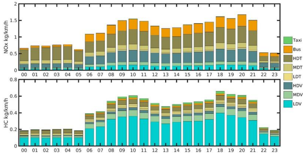
Figure 4. Diurnal variations of the contributions of road vehicles to the NO x emissions and Hydrocarbon (HC) emissions in Beijing during August 2021.
