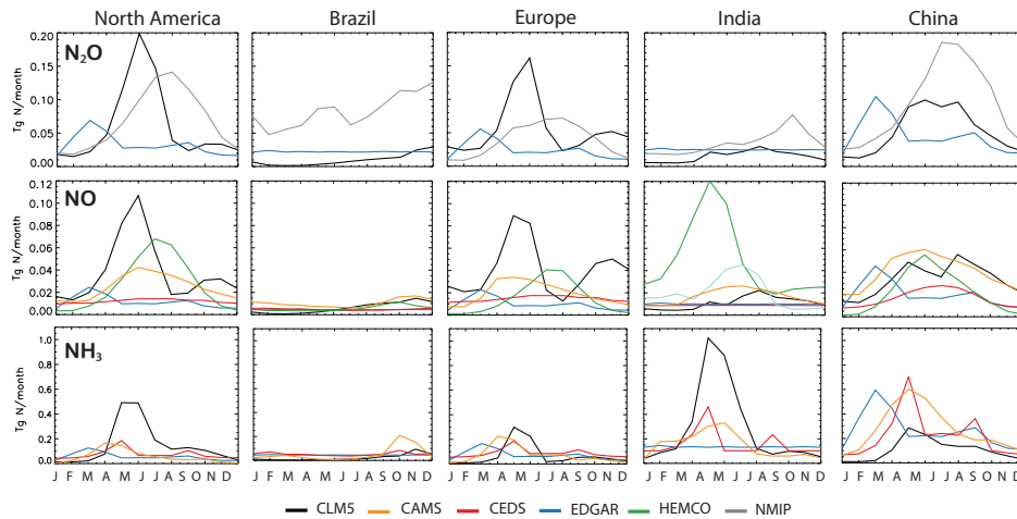
510 Figure 6: Monthly agriculture N 2 O, NO and NH 3 emissions in the main crop regions considered in the study (North America, Brazil, Europe, India, and China) estimated by CLM5, CAMS, CEDS, EDGAR, HEMCO and NMIP (Table 1). Soil NO emissions in HEMCO were weighted by cropland fraction; soil N 2 O in NMIP is the average of only two models that provided monthly output.
