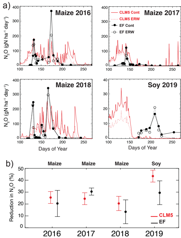
365 Figure 3: Soil N 2 O fluxes at the Energy Farm for the pilot study (maize; 2016) and the large field trials (rotation crops as maize, maize and soybean; 2017–2019). Shown is simulated (red) and observed (black) daily N 2 O fluxes (g N ha -1 day -1 ) at the control (solid lines or solid circles) and basalt-treated plots (dotted lines or open circles) (a) and reductions in N 2 O emissions (%) in the basalt-treated plots compared to the control plots for the simulated by CLM5 (red) and measured at the field experiments (black) (b). Error bars represent variability in the reduction (%) estimated using propagation of errors.
