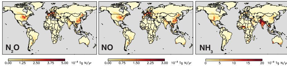
430 Figure 5: Simulated global soil agriculture N 2 O, NO and NH 3 emissions in CLM5 without basalt ('Control Run').
