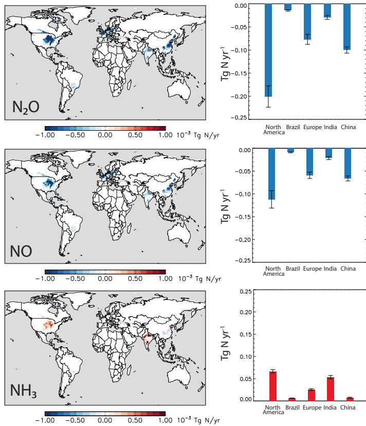
555 Figure 7: Changes in annual soil N 2 O, NO and NH 3 fluxes across the main five agriculture regions (North America, Brazil, Europe, India, and China) based on increases in soil pH resulting from basalt treatment required to sequester 2 Gt CO 2 yr -1 (Figure 2). Shown is the spatial distribution of changes in soil N 2 O, NO and NH 3 (Δ ERW-Control) and the summary of the regional changes (Tg N yr -1 ). Error bars indicate the standard deviation of the annual total changes.
