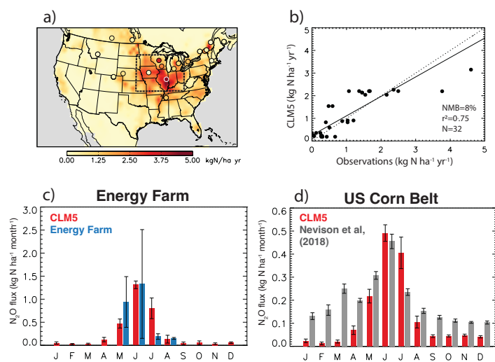
375 Figure 4: Soil N 2 O fluxes in U.S. with modelled and observed values at individual measurement sites (a), the scatter plot with modelled and observed values at the individual sites (b), seasonal variability of monthly soil N 2 O at the location of the Energy Farm (c) and across the US Corn Belt (d). Observations are means from published measurements, including the Energy Farm (2017-2019; Blanc-Betes et al., 2021) or averaged monthly fluxes from the Carbon Tracker- Lagrange regional inversion model (2008-2014; Nevison et al., 2018). The squared-correlation coefficient ( r^2 ), nominal 380 mean bias (NMB, %) and number of observations (N) are shown in the inset. Reduced major axis-regression lines (solid) for croplands and the 1:1 line (dashed) are also shown. The US Corn Belt is represented with a dashed box and location of Energy Farm (40.07 N, 88.2 W) with a white border circle in the CLM5 map. Error bars represent the standard deviation of the annual totals. ▲
