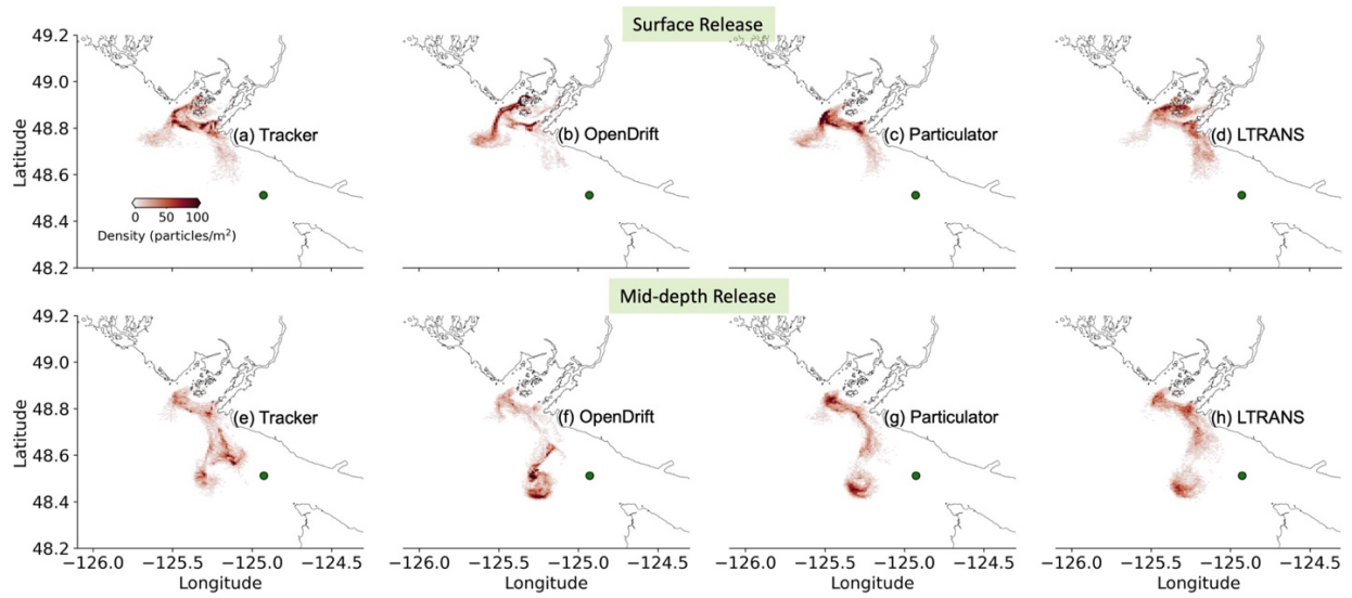
Figure 7: Vertical integral of particle densities for all four offline particle codes after 2 days of tracking using hydrodynamic outputs from the LiveOcean model. (a-d) particles were released from the free surface, (e-h) particles were released from the middle water column. Green dots represent particles release location.
