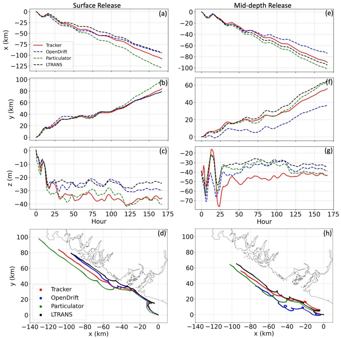
290 Figure 6: The centers of mass in x, y, and z directions for all four offline particle tracking codes simulated using hydrodynamic outputs from the LiveOcean model. (a-c) particles released from the free surface. (e-g) particles released from the middle water column. (d, h) centers of mass in x and y directions.
