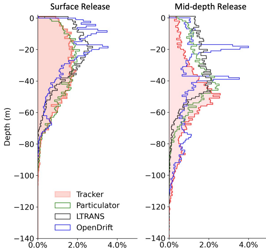
Figure 8: Histogram of vertical particle distribution for all four offline particle codes after 2 days of tracking using hydrodynamic outputs from the LiveOcean model. Left panel: particles released from the free surface; right panel: particles released from the middle water column.
