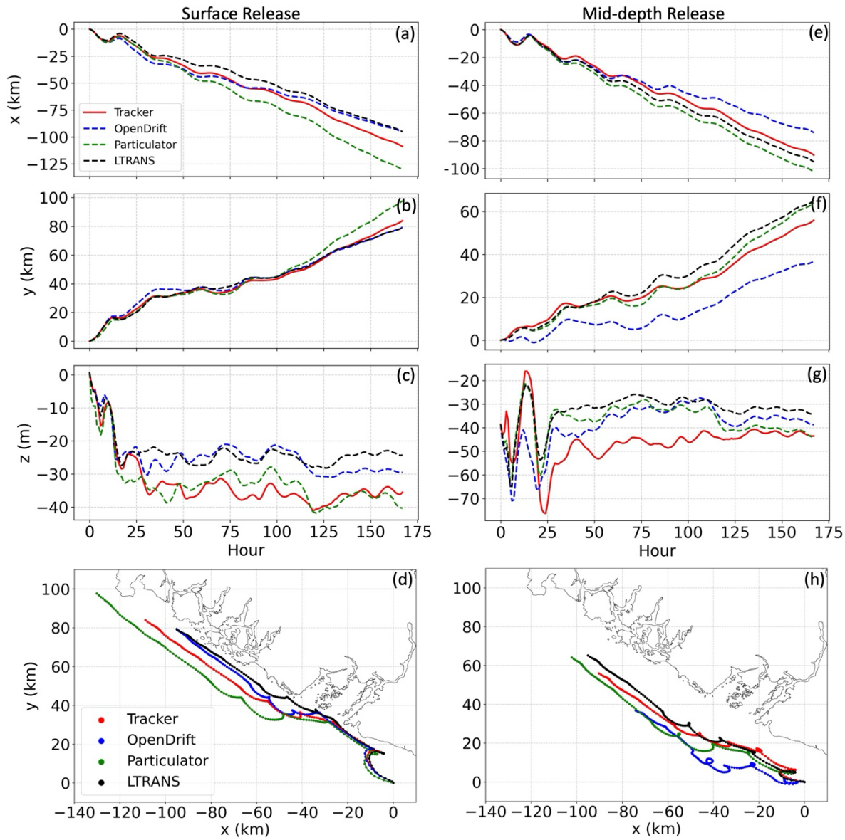
290 Figure 6: The centers of mass in x, y, and z directions for all four offline particle tracking codes simulated in the LiveOcean model. (a-c) particles released from the free surface. (e-g) particles released from the middle water column. (d, h) centers of mass in x and y directions.
