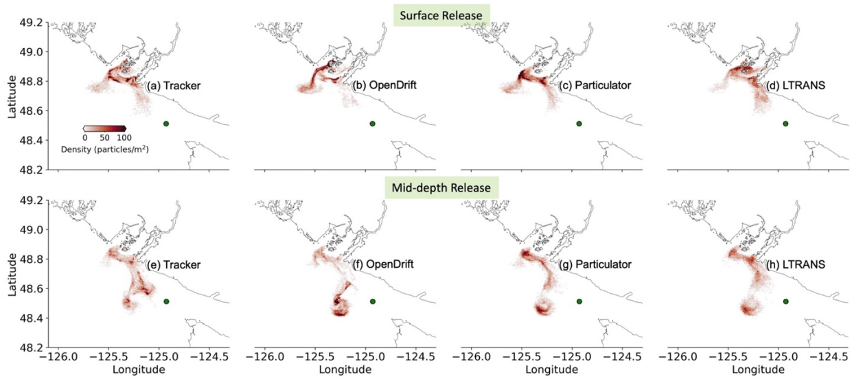
295 Figure 7: Vertical integral of particle densities for all four offline particle codes after 2 days of tracking in the LiveOcean model. (a-d) particles were released from the free surface, (e-h) particles were released from the middle water column. Green dots represent particle release location.
