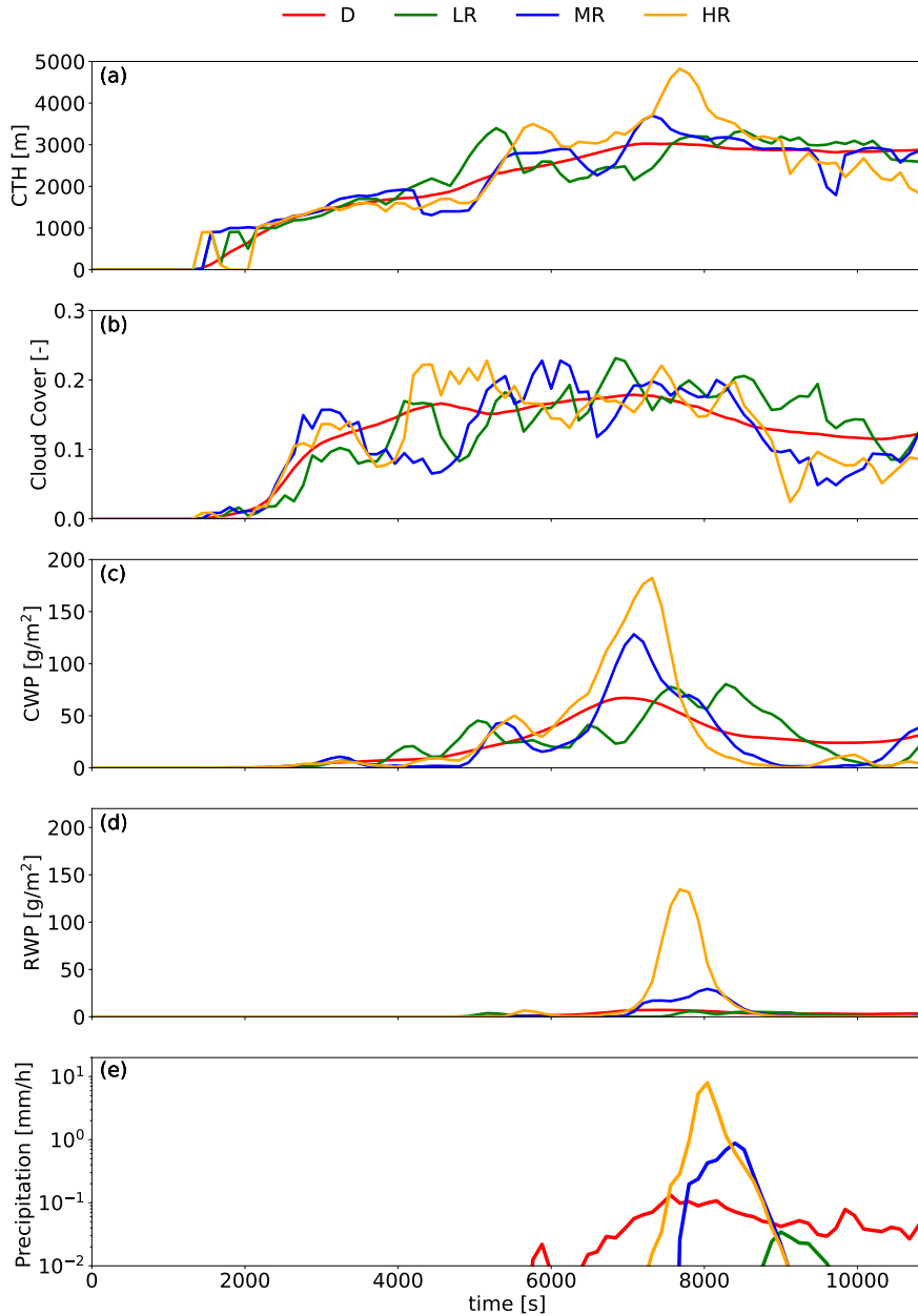
Figure 7. Time series of ensemble averages of cloud top height, cloud cover, cloud water path, rain water path and surface precipitation for D, LR, MR and HR scenarios with N_{\text{SD}}^{(\text{bin})} = 100 . Cloud top height is the vertical position of the topmost cloudy cell. Cloud cover is the fraction of columns with at least one cloudy cell. Cloudy cells are cells with cloud water mixing ratio greater than 10^{-5} . Cloud droplets are droplets with 0.5 \mu\text{m} \leq r_w \leq 25 \mu\text{m} . Rain drops are droplets with 25 \mu\text{m} \leq r_w . Surface precipitation, CWP and RWP are domain averages divided by CC in order to obtain values representative of the cloudy area.
