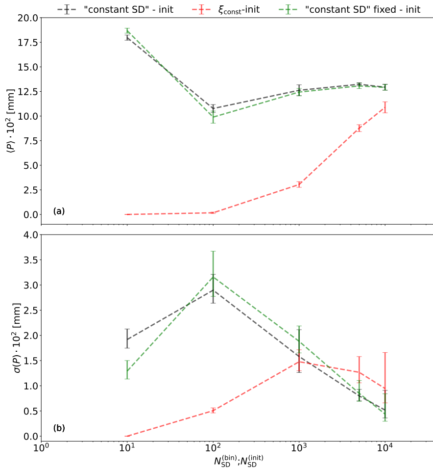
Figure 14. Mean \langle P \rangle and standard deviation \sigma(P) of accumulated precipitation against the number of SDs for HR simulations with three SD initialization methods. Horizontal axis is N_{\text{SD}}^{(\text{bin})} in "constant SD"-init and N_{\text{SD}}^{(\text{init})} in \xi_{\text{const}}\text{-init} . In "constant SD" fixed-init we have N_{\text{SD}}^{(\text{init})} = N_{\text{SD}}^{(\text{bin})} . Error bars represent the 95% confidence interval.
