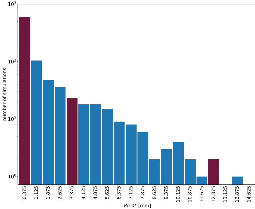
Figure 6. Frequency histogram of accumulated surface precipitation ( P ) from the ensemble of dynamic simulations with N_{\text{SD}}^{(\text{bin})} = 10^2 . Horizontal axis is bin center. Bin width is 7.5 \cdot 10^{-3} mm. The vertical axis is the number of simulations with P within a bin. The bins in burgundy show the expected rain amount for LR, MR and HR velocity fields (left to right).
