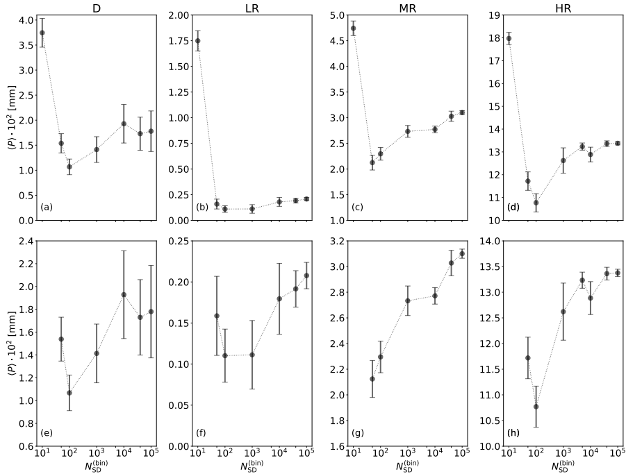
Figure 11. Ensemble mean of precipitation against number of super-droplets for four scenarios: D, LR, MR and HR. In (e-h) the same results are shown as in (a-d), but without N_{SD}^{(bin)} = 10 . Error bars show the 95% confidence interval.
