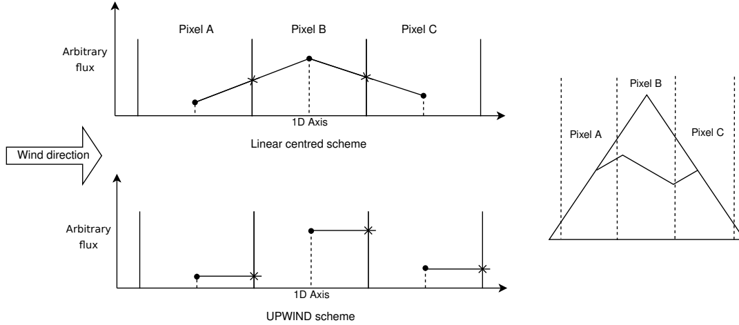
Figure 3. Illustration of the differences between the upwind scheme and a more classic linear scheme for a 1D ideal case. Dots represent the flux estimated for each pixel by Eq 23. Crosses (X) represent the flux value crossing the pixel face. In the linear scheme, the flux value leaving the pixel is the linear interpolation between the two-pixel cell center values. The flux crossing the pixel face can be very different from the cell center computed value. The border flux being linearly interpolated, the border value can be unrealistic. This behaviour can cause interpolation to move erosion out of the expected zone (usually summits, the windiest zone). In the upwind scheme, the flux value crossing the pixel is identical to the cell-centred computed value.
