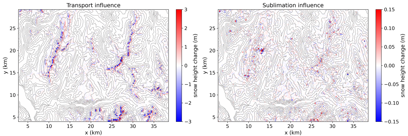
Figure 12. (a) Snow depth difference (m) between TRANS and CTRL simulation on 16 March 2018, which corresponds approximately to the end of accumulation season. (b) Snow depth difference (m) between TRANS+SUBL and TRANS simulations.
