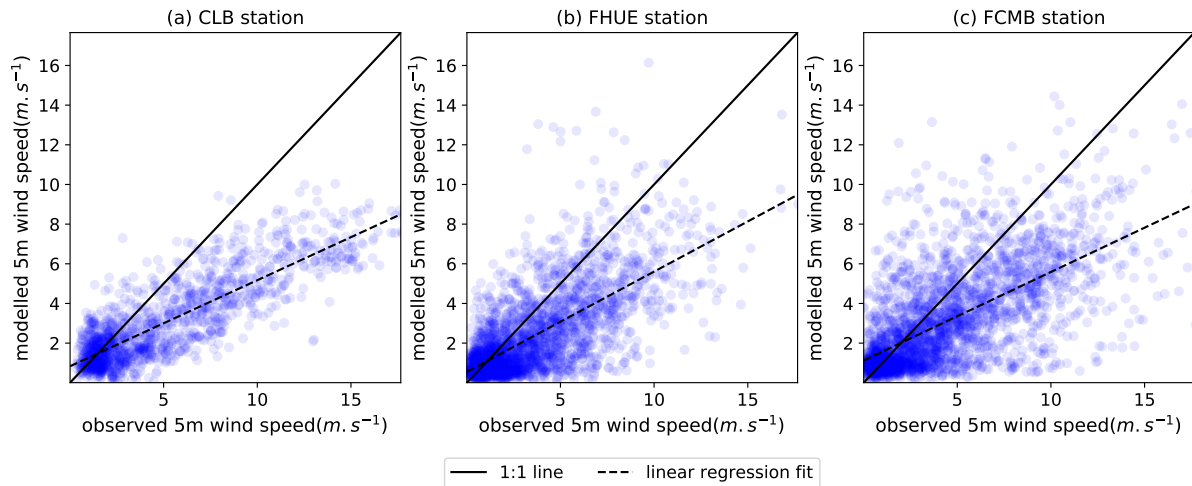
Figure 10. Comparison between observed wind at Col du Lac Blanc and at Huez and Chambon ISAW station and the 250m resolution DEVINE-modelled wind used as a forcing in the closest simulation points. Linear regression line fitting the modelled wind as a function of the observed ones are presented. The presented points are the ones used for blowing snow occurrence evaluation in Fig. 9. Wind observed data were filtered using the same algorithm as Le Toumelin et al. (2022)
