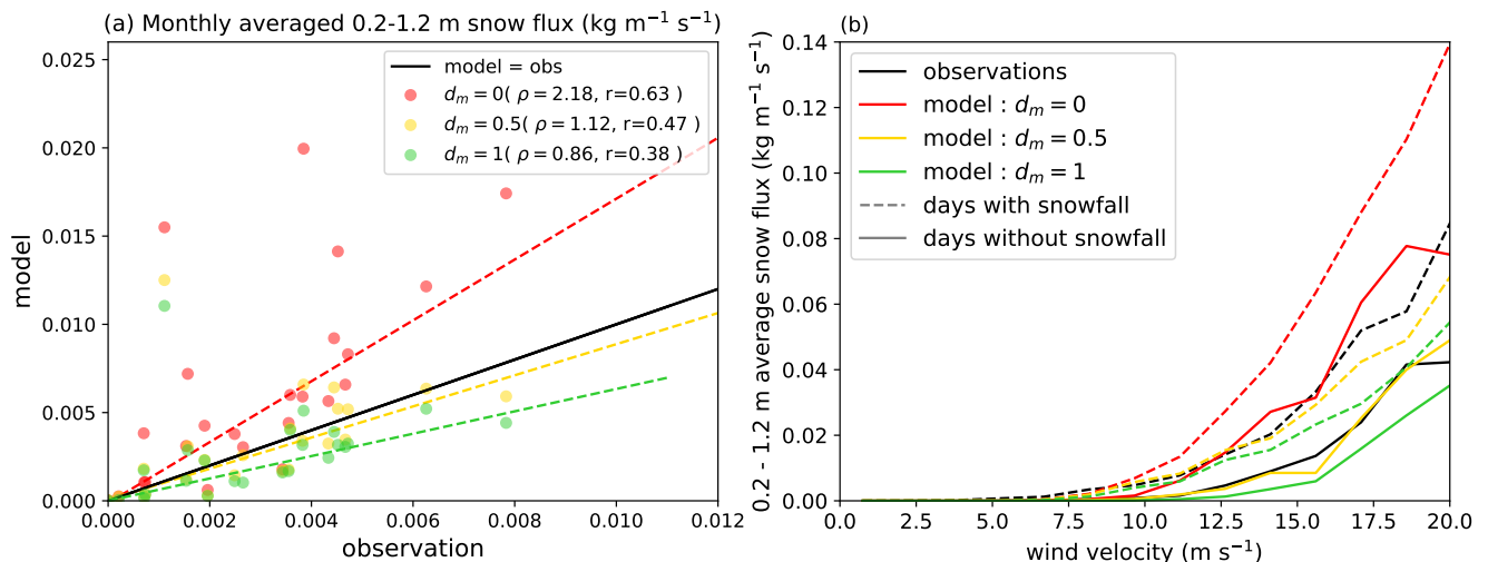
Figure 11. (a) Simulated monthly-averaged Q_{t,int} at Col du Lac Blanc as a function of SPC-observed fluxes, for 3 different values of d_m . The 1:1 line representing equality between the model and observations is drawn in black. The dashed lines are Theil Sen regression fits (Wilcox, 1998) of each model configuration. Ratio model-observation of total cumulated fluxes ( \rho ) and correlation coefficient ( r ) are indicated in the legend. (b) Observed and modelled Q_{t,int} (with the same model configuration as (a)) averaged by 5m-wind velocity intervals, as a function of the interval mean wind friction velocity. Dashed lines are computed from the data for days with snowfall and plain lines with the data for days without snowfall.
