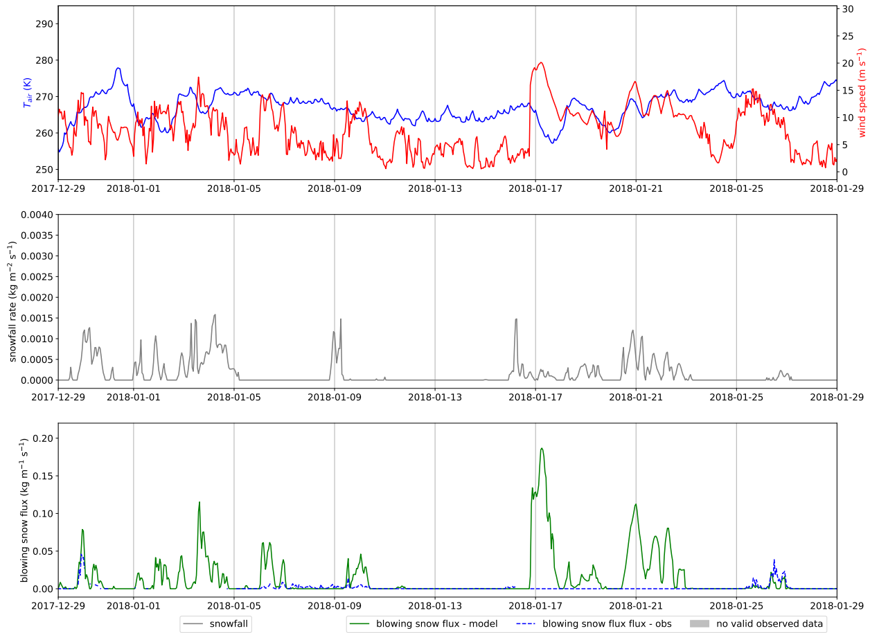
Figure A1. Modelled and SPC-measured 0.2 -1.2 m blowing snow flux during January 2018. SAFRAN-modelled air temperature and solid precipitations, as well as measured wind speed are also represented. This month is a clear outlier in the comparison between observed and modelled fluxes presented in Fig. 11. Here we see that, during the two main modelled events of the month (17 January and 21 January), no flux is detected by the SPC, despite high wind ( 15\text{-}20\text{ m s}^{-1} ), negative temperatures in the previous weeks, preventing the formation of an ice crust, and co-occurring heavy snowfall, which should bring continuously transportable snow. It seems to indicate either an undetected SPC deficiency or big errors in the forcing fields during this month, rather than a model failure.
