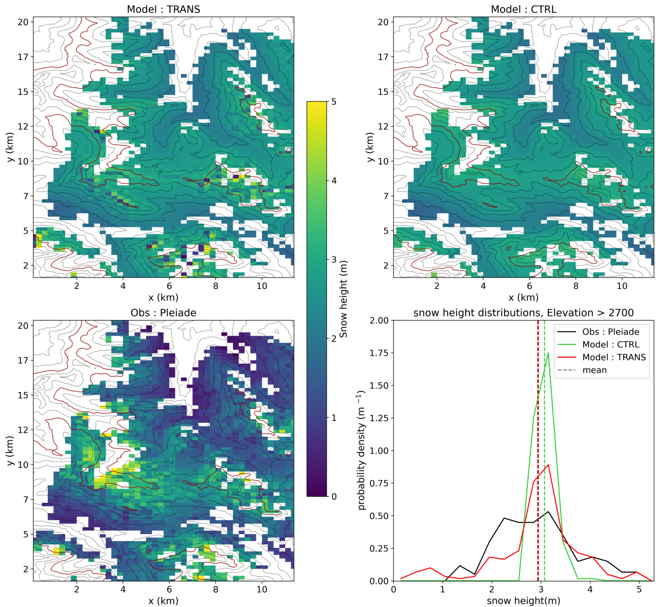
Figure 13. (a) Simulated snow depth map on 16 March 2018 10:00 computed with the TRANS configuration (snow transport activated) on the region covered by Pleiades image. White pixels are those which are not included in the analysis for reasons described Sect. 4.3 (b) Simulated snow depth map with the CTRL configuration (snow transport deactivated). (c) Observed snow depth map with Stereo Pleiades imagery, resampled at 250 m resolution. (d) Probability density distributions of snow depth simulated with TRANS and CTRL configurations, and observed with Pleiades. Mean snow depth are represented as dashed lines (Note Pleiades and TRANS mean snow depths are superposed). Only pixels above 2700 meters are considered. 2700 m isoline is highlighted in red in the subfigures a, b and c.
