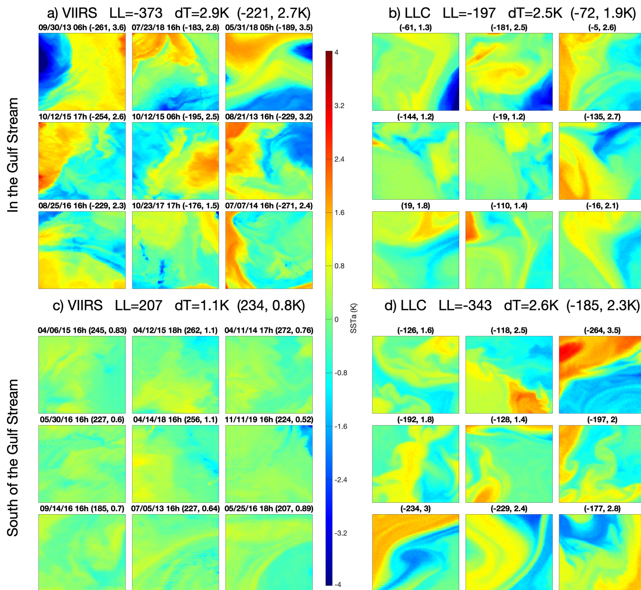
Figure 17. (a) Gallery for VIIRS cutouts in red rectangle of Fig. 16c. (b) Same for LLC4320 cutouts in red rectangle of Fig. 16d. (c) VIIRS cutouts in white rectangle of Fig. 16c. (d) LLC4320 cutouts in white rectangle of Fig. 16d. Dates, times, LL and dT as in Fig. 13.
