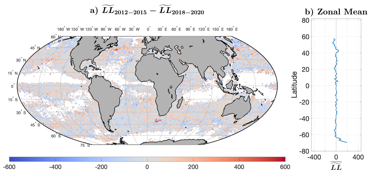
Figure A3. (a) \overline{LL}_{2012-2015} - \overline{LL}_{2018-2020} . White areas - less than 5 cutouts in the corresponding HEALPix cell in 2012–2015 and/or 2017–2020. The same color palette is used in this figure as in Fig. 5 to facilitate comparison as well as to emphasize the significant differences in \overline{LL}_{VIIRS} - \overline{LL}_{LLC} . (b) Zonal mean of a.
