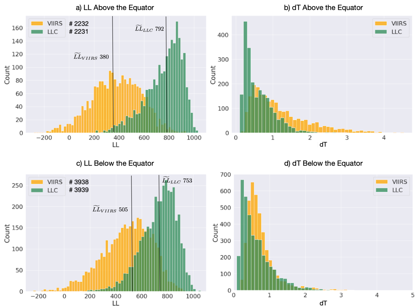
Figure 12. (a) Histograms of LL for all VIIRS (yellow) and LLC4320 (green) cutouts above the Equator in the focus area. (b) Histograms of dT for the same region as (a). (c) As for (a) except below the Equator. (d) As for (b) except below the Equator. The median values of the distributions are indicated for (a) and (c), as are the number of cutouts contributing to each. The number of cutouts apply to the corresponding dT frames.
