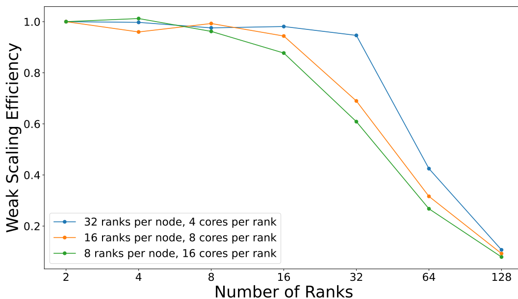
Figure 7. Weak scaling parallel efficiency for the tsunami model test case with different set ups of ranks per node and cores per rank on ARCHER2. A drop off in performance can be seen when moving from single to multi-node runs.
