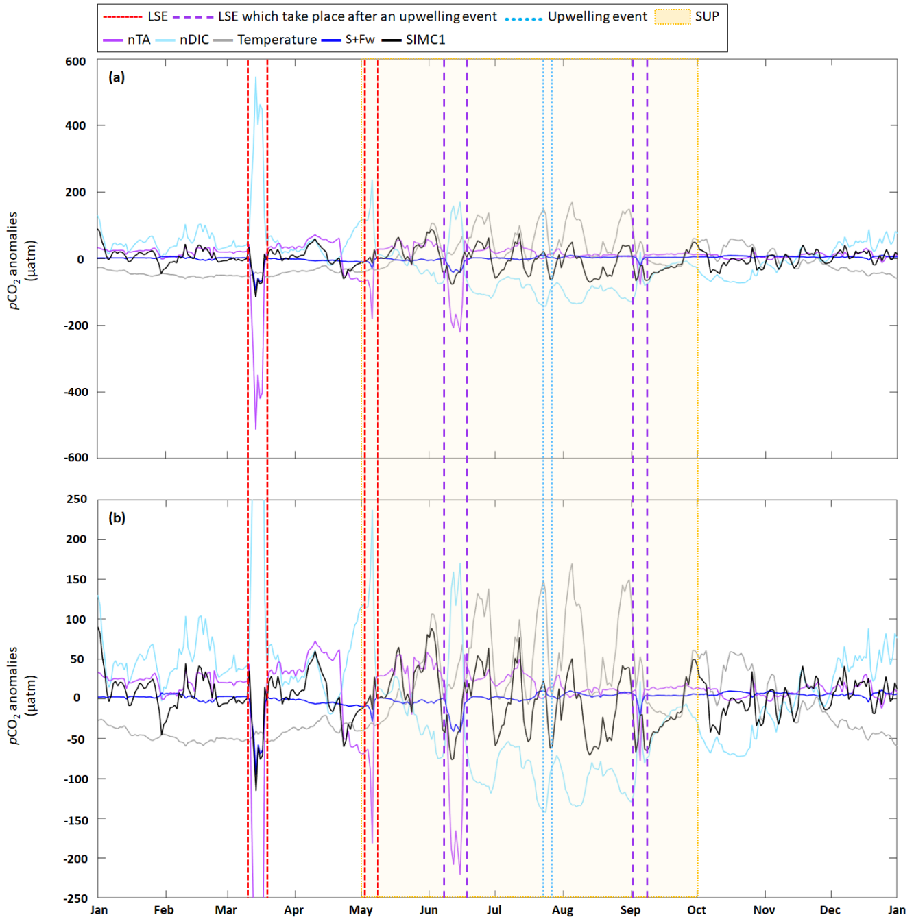
820 Figure D1. Time series for 2017 of daily average (a) p\text{CO}_2 anomalies generated by DIC, TA, S+Fw and temperature based on the approach in Lovenduski et al. (2007) (Note: the dark blue line is sometimes obscured by the black line, especially in March), (b) enlargement of the panel a between -250 and 250 \mu\text{atm} . LSE and an upwelling event have been highlighted. The summer upwelling period (SUP) is indicated by yellow shading.
