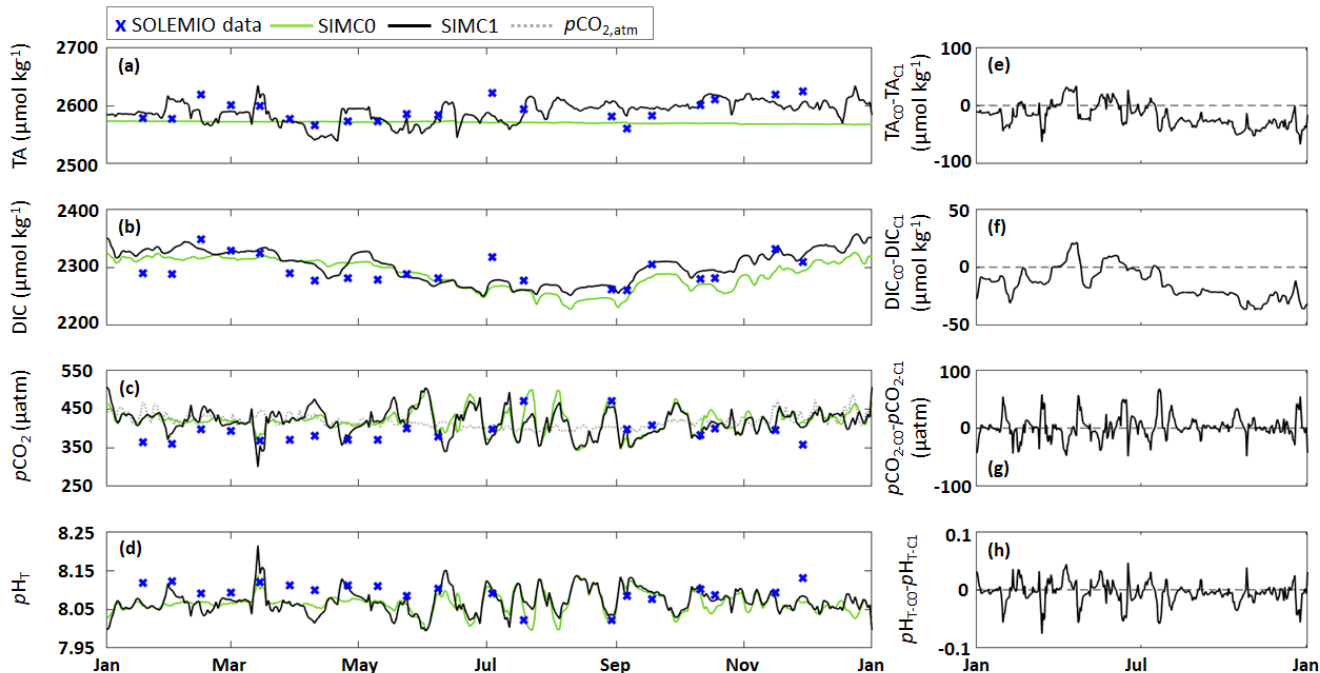
Figure 3. (a-d) Comparison of model outputs from the SIMC0 (autochthonous formulation) and SIMC1 (allochthonous 315 formulation), model runs showing daily averages of (a) TA, (b) DIC, (c) seawater p\text{CO}_2 and CAV atmospheric p\text{CO}_2 and (d) \text{pH}_T . (e-h) Differences between SIMC0 and SIMC1 outputs for each variable (VARC0 – VARC1).
