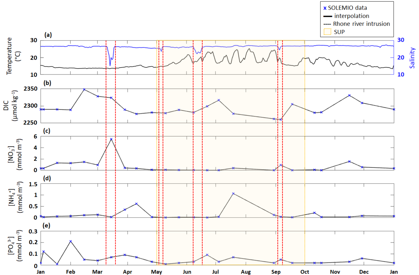
830 Figure E1. Time series of surface (a) temperature (PLANIER measurements) and salinity (CARRY measurements) and interpolated (b) DIC, (c) \text{NO}_3^- , (d) \text{NH}_4^+ and (e) \text{PO}_4^{3-} concentration at SOLEMIO station. SOLEMIO data are represented by blue markers. Rhone River intrusions studied here are indicated by the red dotted lines and the SUP is shaded in yellow.
