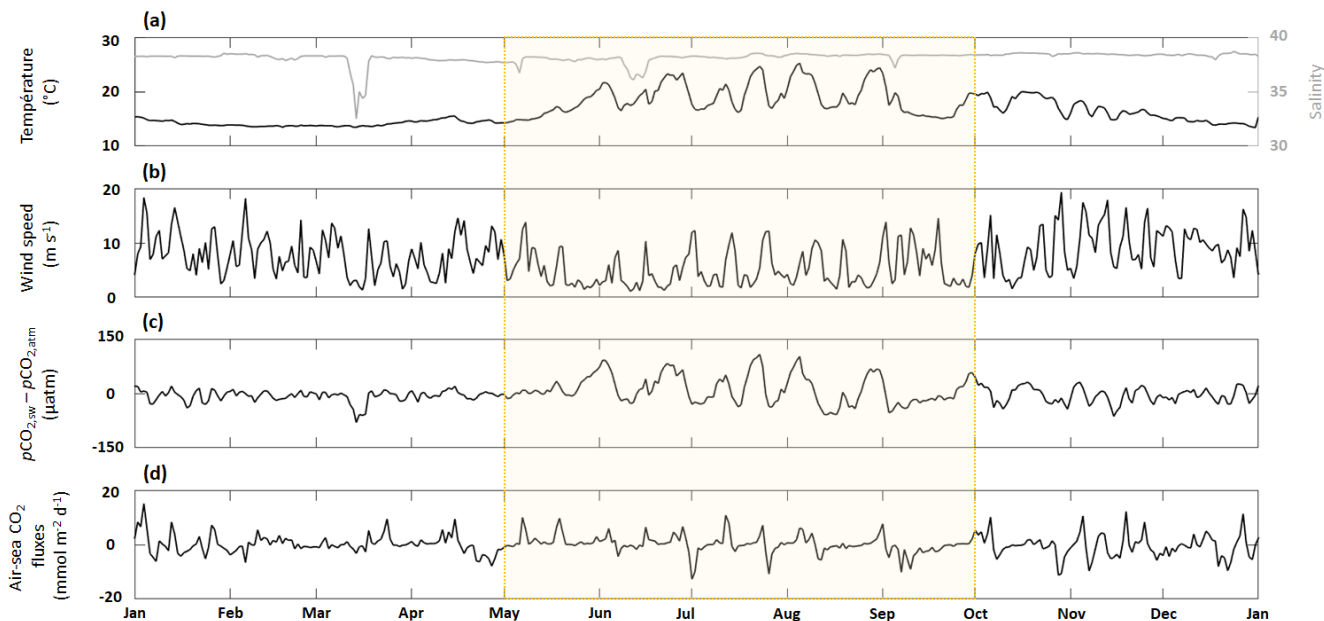
Figure 5. Time series of (a, e) in situ daily average sea surface temperature (black line) and salinity (grey line) (b, f) SIMC1 daily average wind speed (c, g) the difference between SIMC1 daily average seawater p\text{CO}_2 and in situ daily average atmospheric p\text{CO}_2 (d, h) SIMC1 daily average air-sea \text{CO}_2 fluxes (aeration process). The summer upwelling period (from 1 May to 1 October) is highlighted in yellow.
