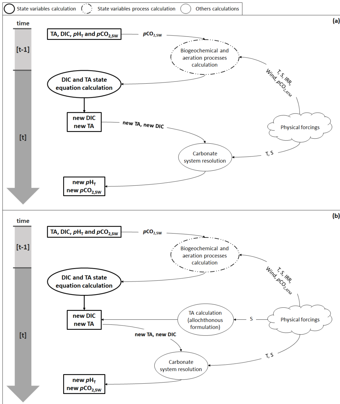
270 Figure 3. Flow diagram illustrating the steps needed to calculate pH_T and pCO_2 (a) using the autochthonous formulation (Eq. 4) and (b) with the allochthonous formulation (Eq. 5 and 6). Physical forcings include temperature (T), salinity (S), solar irradiance (IRR), wind speed (Wind) and atmospheric pCO_2 ( pCO_{2,ATM} ).
