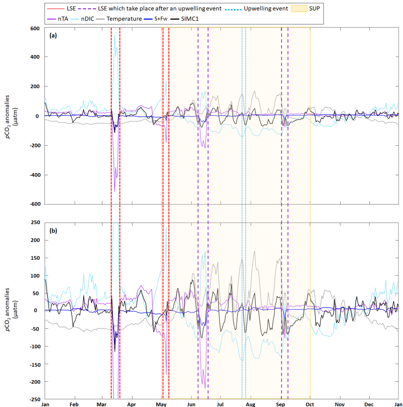
825 Figure D1. Time series for 2017 of daily average (a) pCO 2 anomalies generated by DIC, TA, S+Fw and temperature based on the approach in Lovenduski et al. (2007) (Note: the dark blue line is sometimes obscured by the black line, especially in March), (b) enlargement of the panel a between -250 and 250 μatm. LSE and an upwelling event have been highlighted. The summer upwelling period (SUP) is indicated by yellow shading.
