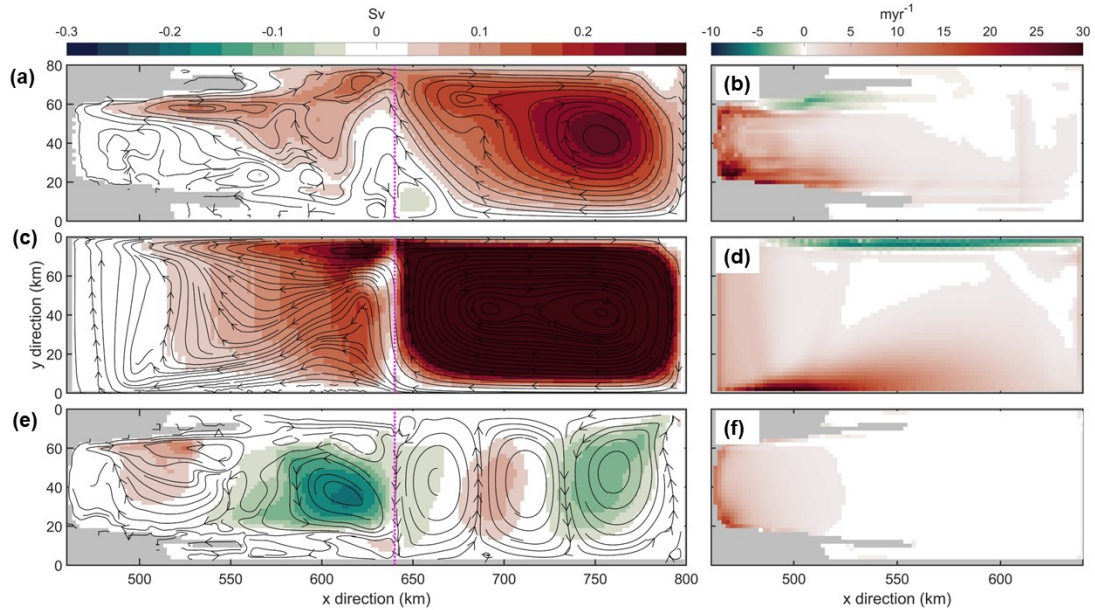
Figure 3. Panels (a), (c), and (e) show plane views of the quasi-steady state barotropic streamfunction from the simulations restored to the MEAN profiles for the FVCOM-ISMOP+ (FI_C2M), FVCOM-Wedge (FW_C2M), and ROMS-ISOMIP+ (RI_C2M) configurations, respectively. The black lines and arrows indicate the barotropic flow, while the magenta dashed line mark the ice front. Panels (b), (d), and (f) display spatial distribution of melt rates from the simulations FI_C2M, FW_C2M, and RI_C2M, respectively.
