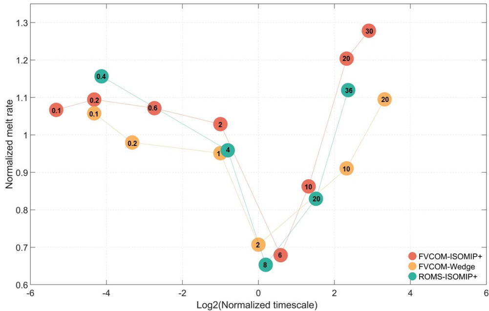
Figure 6. Normalized melt rates plotted against normalized timescales from all the simulations across the FVCOM-ISOMIP+, FVCOM-Wedge, and ROMS-ISOMIP+ model configurations. The period of oscillating profiles used in each simulation is denoted by the black text within the colored circles.
