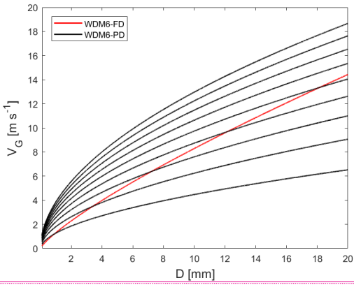
Figure 1: V_G ( m s^{-1} ) as a function of D_G (mm) with various \rho_G between 100 and 900 ( kg m^{-3} ), utilizing a_G and b_G values from Table 2. The V_G - D_G relationship in the original WDM6 scheme (WDM6-FD) is shown by a red line.
