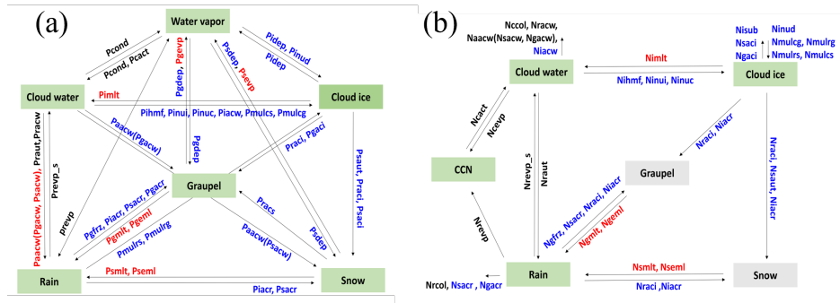
Figure A1. Flowcharts of microphysical processes for predicting (a) mass mixing ratio ( S_{q_x} ) and (b) number concentration ( S_{N_x} ) of hydrometeors in WDM6 scheme. The number concentrations of hydrometeors in the green boxes are predicted only (e.g., cloud water, cloud ice, rain, and cloud condensation nuclei (CCN)). Microphysical terms drawn with red (blue) are activated when the temperature is above (below) 0^\circ\text{C} . Terms drawn in black are activated regardless of temperature.
