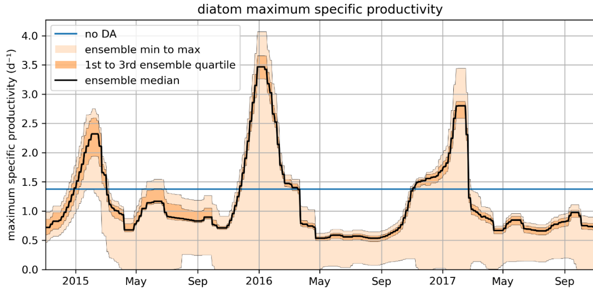
500 Figure 10. The November 2014 – October 2017 time series for the diat-MSP parameter, showing the median value, the ensemble spread and the region between the two quartiles around the median. The figure also shows the (constant) parameter value in the non-assimilated case (blue line).
