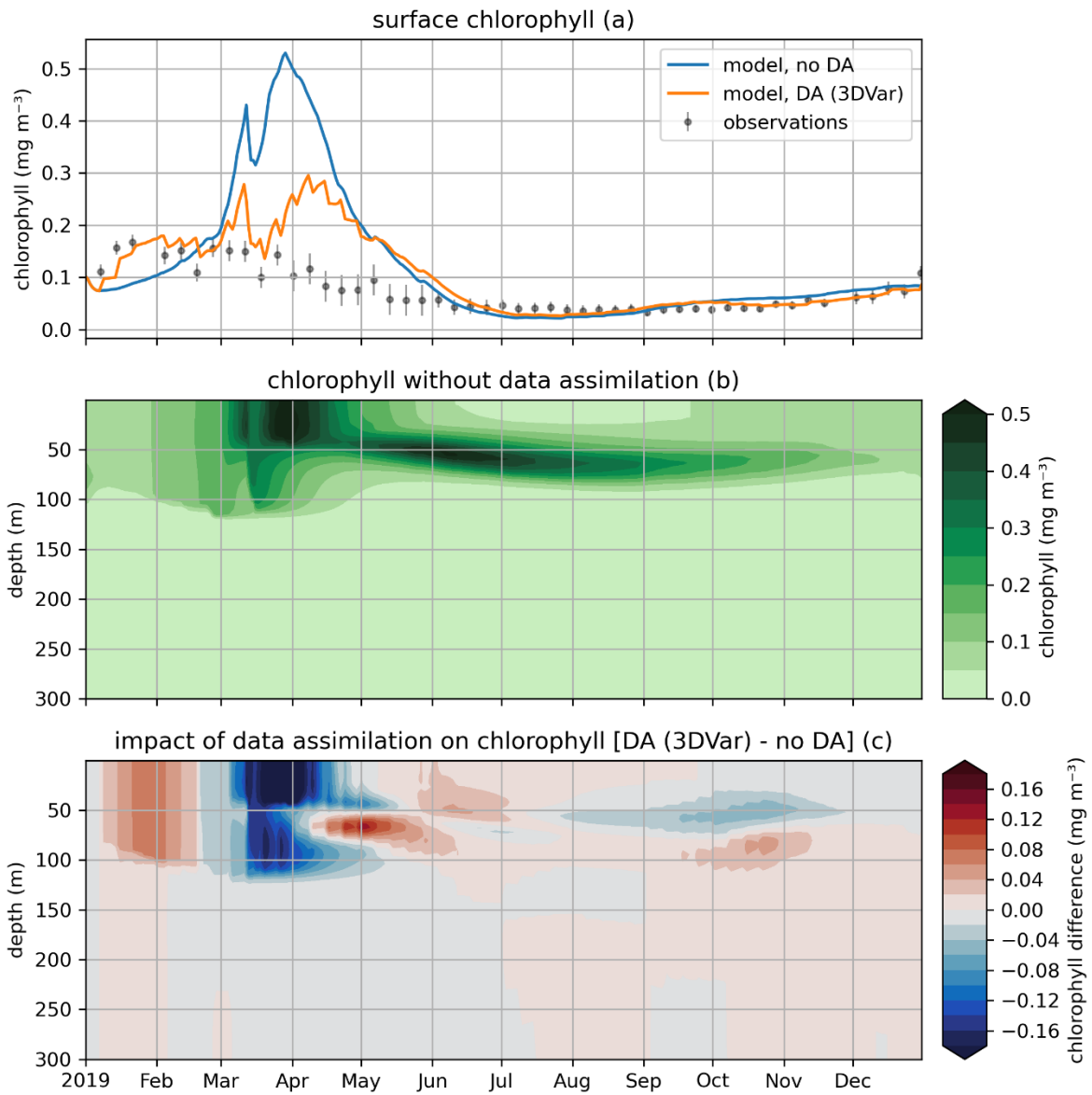
425 Figure 8. Modelled and observed chlorophyll in a free model run (“no DA”) and in the experiment where remotely sensed surface chlorophyll were assimilated (“DA (3DVar)”). The top panel (a) shows surface chlorophyll (modelled and observed), the middle panel (b) shows the chlorophyll throughout the water column in the free run, and the bottom panel (c) shows the difference in chlorophyll between the variational assimilation experiment and the free run.
