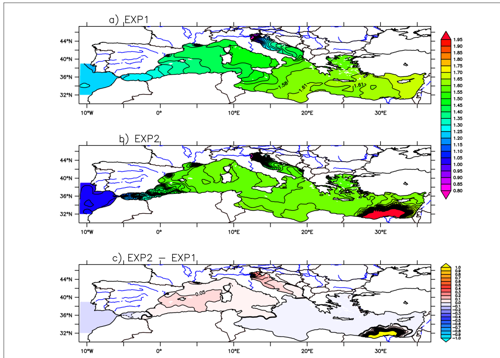
Figure E1. a) EXP1: we use the same approach as described in our submitted paper, i.e., ^{18}R_{river} = ^{18}R_{precip} \times ^{18}R_{runoff} . b) EXP2: we added the ^{18}O_{river} simulated by the old version of LMDZiso at a lower resolution R96x71. ^{18}R_{river} = ^{18}R_{riverLMDZiso} \times ^{18}R_{runoff} . c) the difference EXP2 - EXP1
