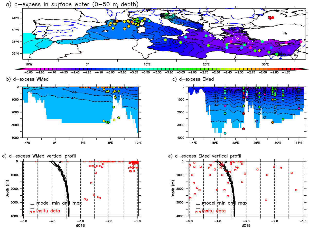
Figure 8. Horizontal map of d-excess in the surface water defined as deuterium excess ( d\text{-excess} = \delta D_w - 8 \cdot \delta^{18}O_w , Dansgaard (1964)). Color-filled dots represent in-situ observations from (Gat et al., 1996; Reverdin et al., 2022). Both model and in-situ data use the same color scale.
