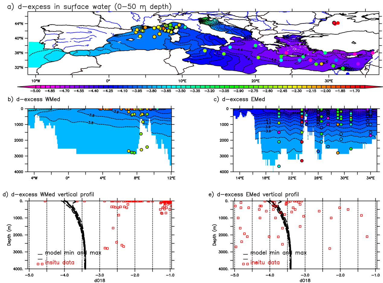
Figure 8. Horizontal map of d-excess in the surface water defined as deuterium excess ( d\text{-excess} = \delta D_w - 8 * \delta^{18}O_w , Dansgaard (1964)). Color-filled dots represent in-situ observations from (Gat et al., 1996). Both model and in-situ data use the same color scale.
