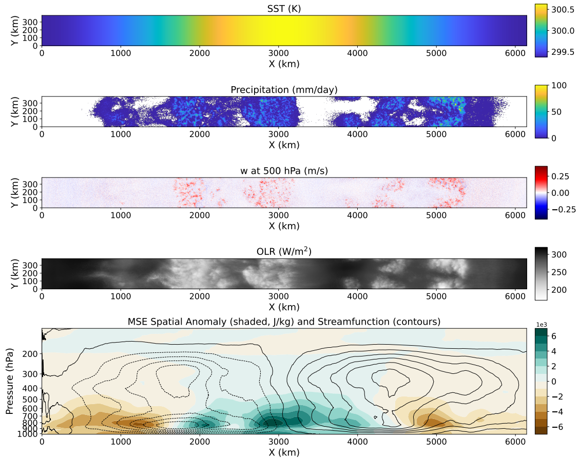
Figure 2. Daily-mean SST (K), precipitation ( \text{mm d}^{-1} ), vertical motion at 500 hPa ( \text{m s}^{-1} ), and outgoing longwave radiation (OLR; \text{W m}^{-2} ) at day 150, and moist static energy (MSE; \text{J kg}^{-1} ) anomaly from the spatial mean and streamfunction averaged over days 100 - 200 in the MW_300dT1p25 simulation with SAM. Streamfunction is calculated by integrating y -averaged \rho w across the x -axis of the simulation, with contours every 500 \text{ kg m}^{-1} \text{ s}^{-1} .
