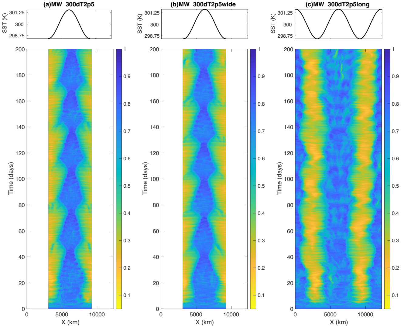
Figure 12. Hovmöller diagrams of y-averaged column relative humidity in the MW_300dT2p5 simulation with SAM for (a) the standard domain size, (b) a domain that is twice as wide in the y-dimension, (c) a domain that is twice as long in the x-dimension. Note that these SAM simulations, used to test the domain size, were performed with SST(x) = \langle SST \rangle + \frac{\Delta SST}{2} \cos\left(\frac{2\pi}{L_x} \left(x + \frac{L_x}{2}\right)\right) with \lambda = 6000 km and L_x = 6144 km, rather than Equation 1 and \lambda = L_x as required for RCEMIP-II. The top panel shows the SST pattern.
