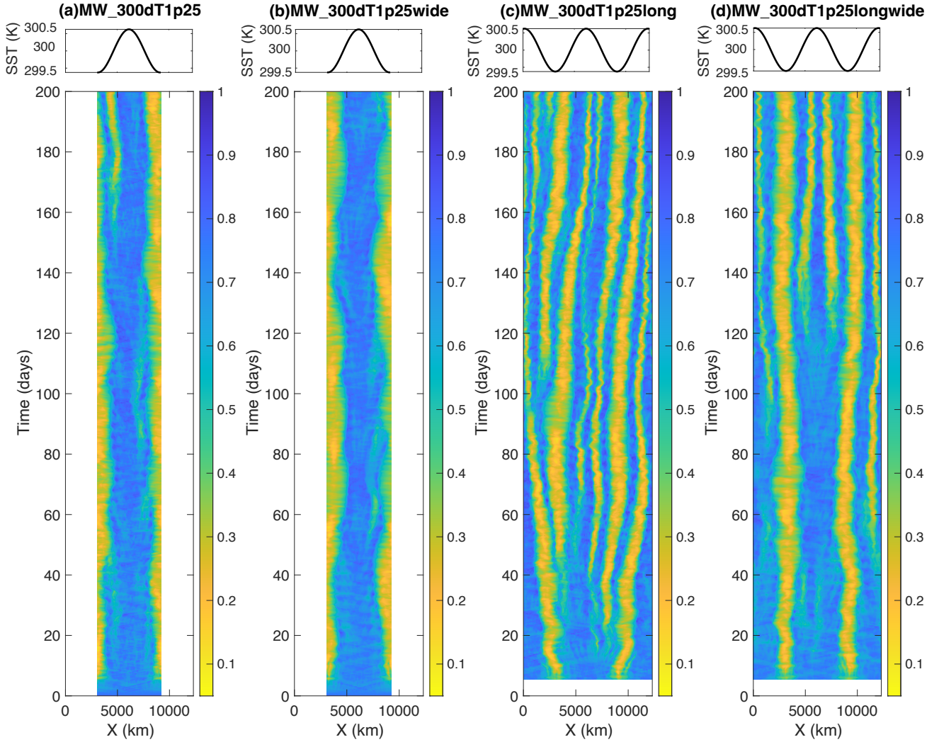
Figure 11. Hovmöller diagrams of y-averaged column relative humidity in the MW_300dT1p25 simulation with SAM for (a) the standard domain size, (b) a domain that is twice as wide in the y-dimension, (c) a domain that is twice as long in the x-dimension, and (d) a domain that is twice as wide and twice as long. Note that these SAM simulations, used to test the domain size, were performed with SST(x) = \langle SST \rangle + \frac{\Delta SST}{2} \cos\left(\frac{2\pi}{L_x}\left(x + \frac{L_x}{2}\right)\right) with \lambda = 6000 km and L_x = 6144 km, rather than Equation 1 and \lambda = L_x as required for RCEMIP-II. The top panel shows the SST pattern. Note that the output for the first five simulation days in panels (c) and (d) was corrupted and thus is not plotted.
