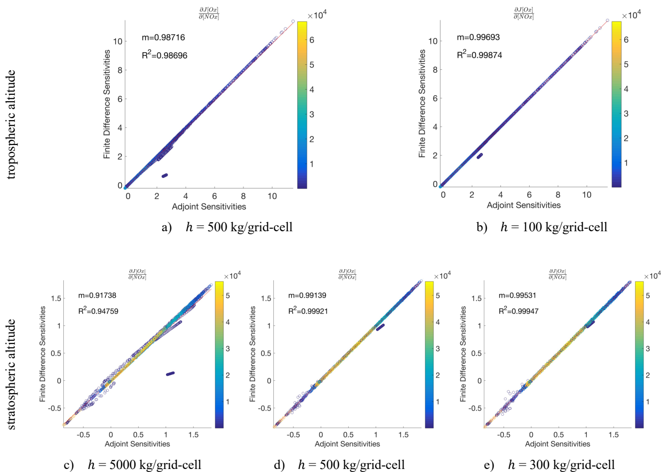
Figure 4: Adjoint model evaluation after a single chemistry time-step (1 hour) with disabled transport and convection processes for different \text{NO}_x perturbation sizes, h . Top row (panels a, b) displays the evaluation at a tropospheric model layer (4 km) and bottom row (panels c, d, e) at a stratospheric model layer (21 km). The adjoint gradients compared to finite difference gradients, with the corresponding linear regression slope, m , and coefficient of determination, R^2 , for all N column models tested simultaneously ( N=46 \times 72 ). Each point on the parity plot is coloured according to the \text{NO}_x mass in the grid-cell.
