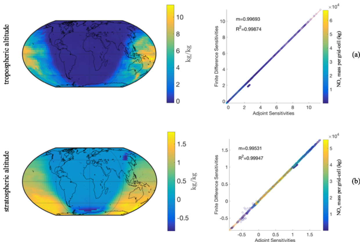
5 Figure 3 Adjoint model evaluation after a single chemistry time-step (1 hour) with disabled transport and convection processes. In the left column the adjoint sensitivities depict changes in O_3 mass for NO_x perturbations in the same grid-cell. In the right column are the adjoint gradients compared to finite difference gradients, with the corresponding linear regression slope, m , and coefficient of determination, R^2 , for all N column models tested simultaneously ( N=46 \times 72 ). Each point on the parity plot is coloured according to the NO_x mass in the grid-cell. Top row (a) shows a tropospheric model layer (4 km) and bottom row (b) shows a stratospheric model layer (21 km).
