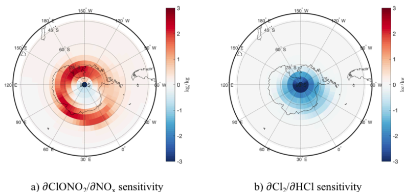
5 Figure 7: Antarctic chlorine activation (a) and deactivation (b) adjoint sensitivities for a two-week September simulation at a stratospheric vertical model layer (~21 km).
