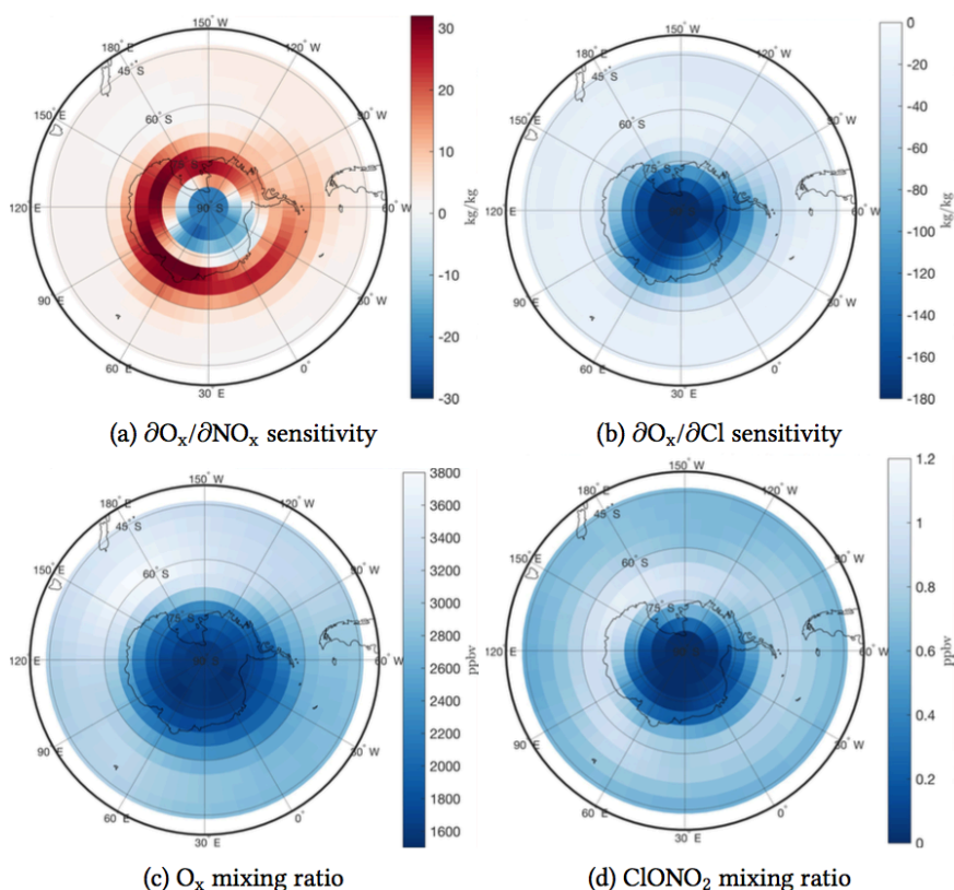
Figure 6 Stereographic plots of \partial O_x / \partial NO_x and \partial O_x / \partial Cl sensitivities in kg/kg and O_x and ClONO_2 mixing ratios in ppbv for a two-week September simulation at a stratospheric vertical model layer (~21 km).
