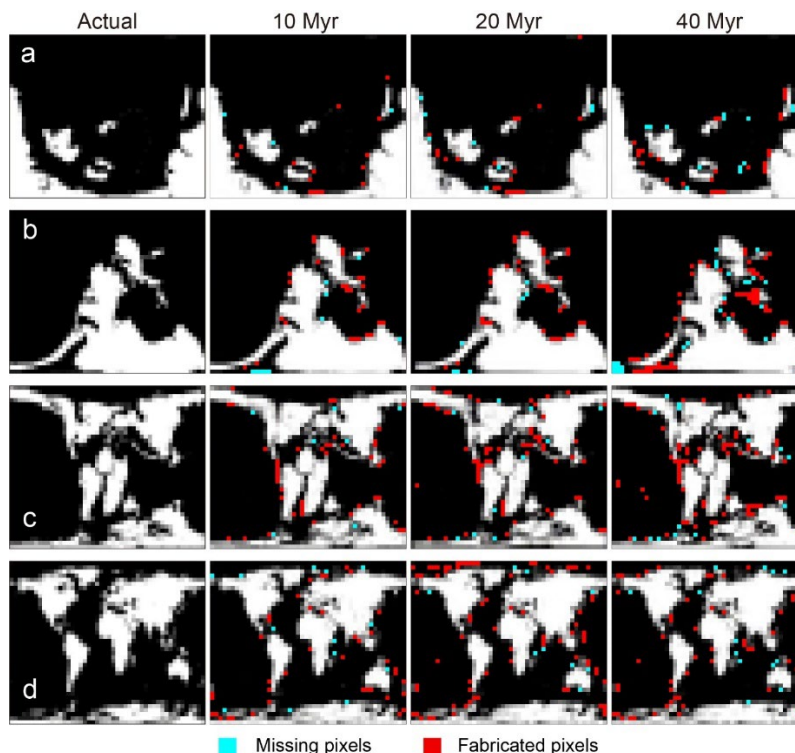
245 Figure 4. Comparative visualization of actual PaleoDEM and model-predicted frames at selected time intervals. This figure illustrates the comparative visualizations at (a) 535 Ma, (b) 315 Ma, (c) 105 Ma, and (d) 25 Ma. The grey pixels represent areas impacted by nearest-neighbour downsampling in the paleogeographic maps. The missing pixels indicate areas present in the original frames but absent in the model-predicted frames; the fabricated pixels show areas absent in the original frames but present in the model-predicted frames.
