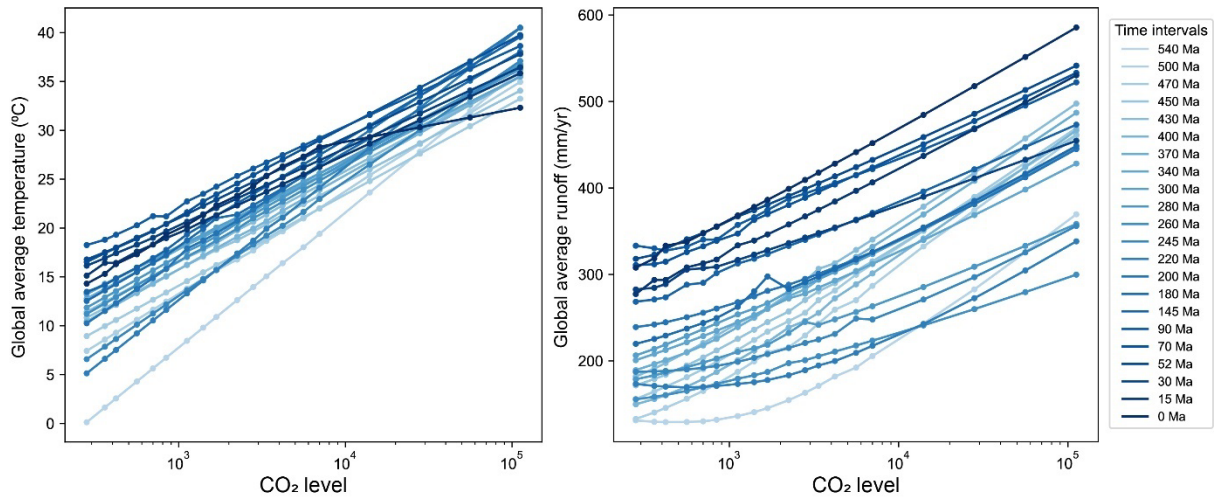
290 Figure 6. Global average surface air temperature and average continental runoff over CO 2 levels in the FOAM dataset. The representation is color-coded with a descending blue gradient, where light blue represents more ancient conditions, and dark blue denotes more recent scenarios. Note that the 0 Ma curve is built from only one CO 2 level (preindustrial), with an arbitrary increase in temperature and runoff applied when CO 2 levels change.
