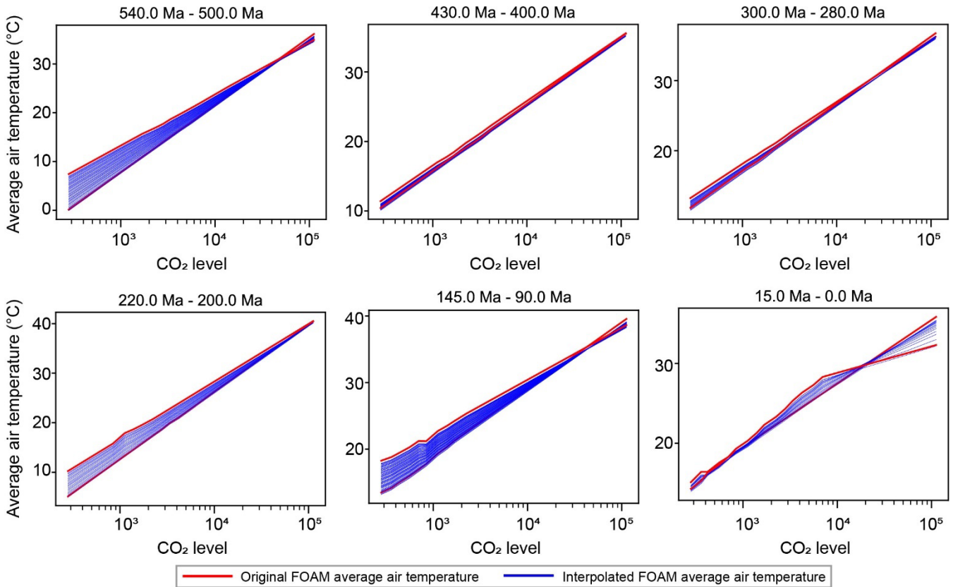
310 Figure 7. Trends in global temperature changes corresponding to varying CO 2 levels. Each subplot features one of the 21 distinct time intervals between members of the FOAM dataset. Within each subplot, the red lines delineate the keyframe average temperature variations and the blue lines show the Deep Learning-interpolated average temperature at each 1 Myr. See Fig. A1 for the full 21 subplots.
