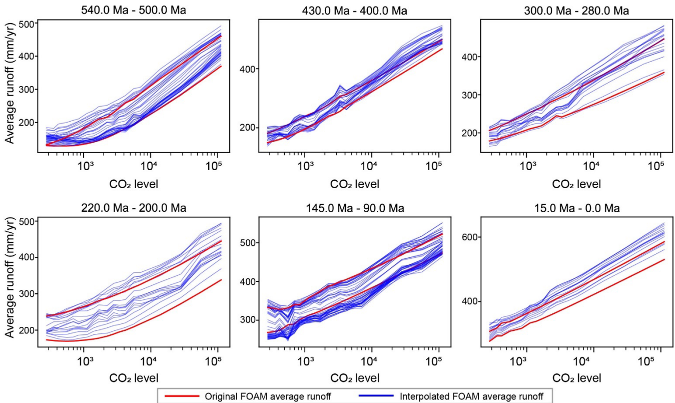
315 Figure 8. Trends in runoff changes corresponding to varying CO 2 levels. As with Fig. 7, the subplots represent the runoff changes between the original runoff outputs from the FOAM dataset. The red lines are original average runoff in the FOAM dataset, and blue lines are Deep Learning interpolated data. See Fig. A2 for the full 21 subplots.
