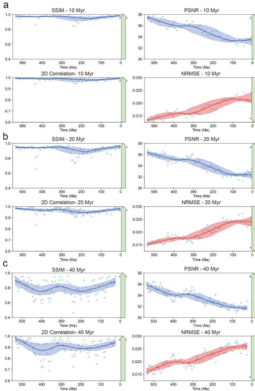
210 Figure 2. Comparative Evaluation of Performance Utilizing (a) 10 Ma, (b) 20 Ma, and (c) 40 Ma Intervals within the PaleoDEM Dataset. The blue line represents the LOWESS (Locally Weighted Scatterplot Smoothing) fitting curve with a fraction of 0.4, serving as an indicator of the central trend. The light blue shaded bands illustrate the confidence interval, derived from a 1000-resampling bootstrap method, providing a measure of the precision and uncertainty of the estimated fit. The NRMSE is represented in red colour because it signifies error, thus its trend is converse to the other three metrics. The green arrows indicate the direction of better performance. See text for detailed discussions.
