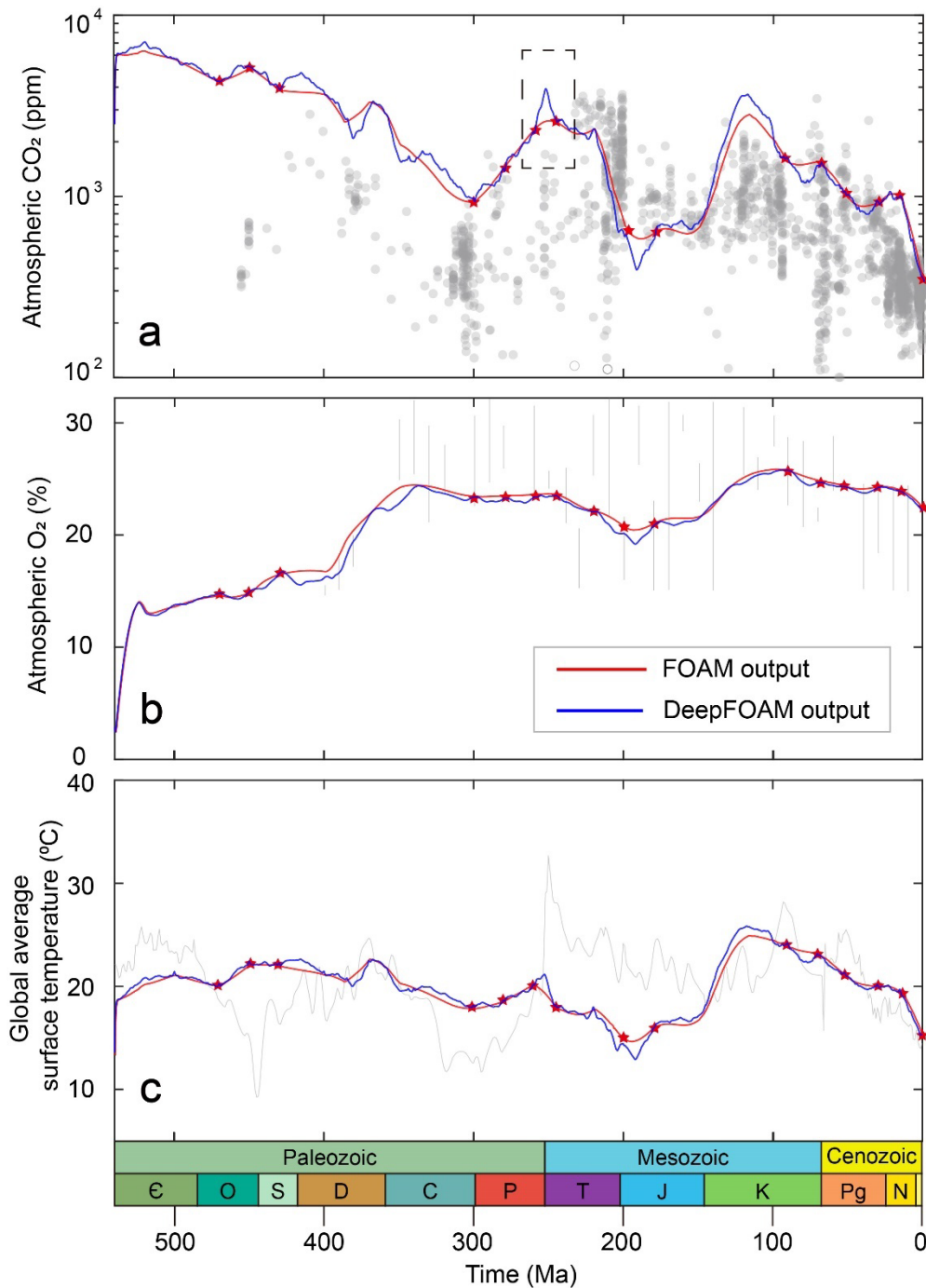
350 Figure 9. Phanerozoic output comparisons between the SCION-FOAM and SCION-DeepFOAM. (a) atmospheric CO 2 concentration (proxy data represented by scatter symbols; sources: Foster et al., 2017; Witkowski et al., 2018), (b) atmospheric O 2 concentration (proxy data represented by vertical lines; sources: Glasspool and Scott, 2010; Lenton et al., 2016), and (c) global average surface temperature (proxy data represented in gray; source: Scotese et al., 2021). The red stars on the diagram represent the time intervals of 20 Myrs or less in the FOAM dataset. The dashed box in Fig. 9a marks the significant CO 2 increase at 253Ma.
