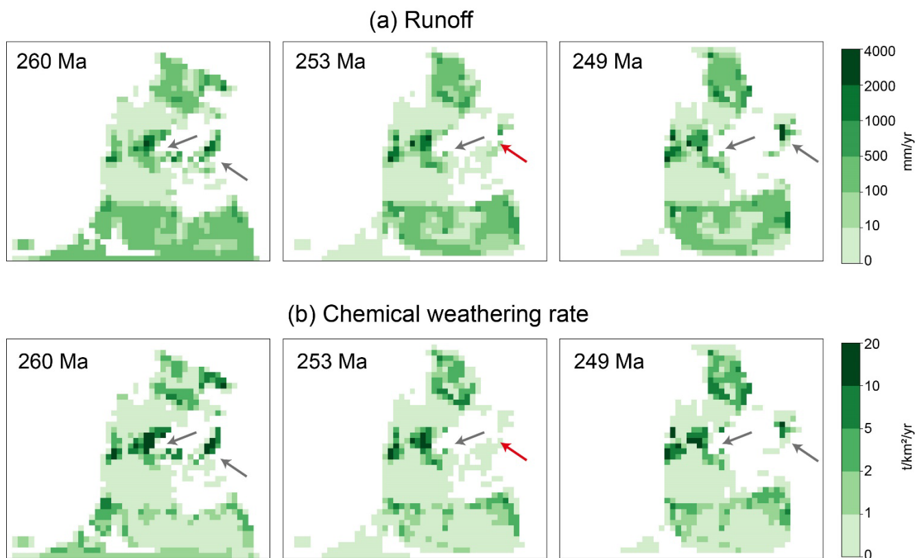
355 Figure 10. Runoff (a) and chemical weathering rates (b) for 260 Ma, 253 Ma, and 249 Ma. During the 260–245 Ma period, the low-latitude regions surrounding the Paleo-Tethys Ocean exhibit high runoff and corresponding high weathering (highlighted by grey arrows). These characteristics are derived from the FOAM dataset. However, during the 253 Ma interval, the Deep Learning method predicts reduced runoff and corresponding decreased weathering. This reduction is primarily attributed to the lowered runoff in eastern low-latitude plates, such as North and/or South China (marked by the red arrow).
