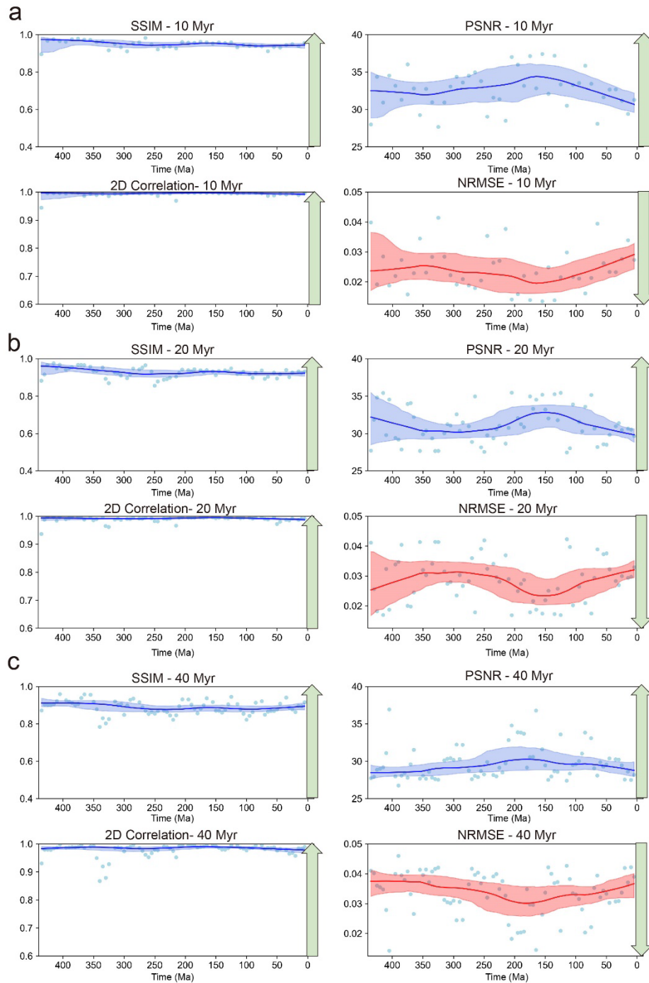
265 Figure 5. Comparative evaluation of performance utilizing (a) 10 Myr, (b) 20 Myr, and (c) 40 Myr intervals within the SAT Dataset. See Figure 2 for detailed explanations of the image symbols.
