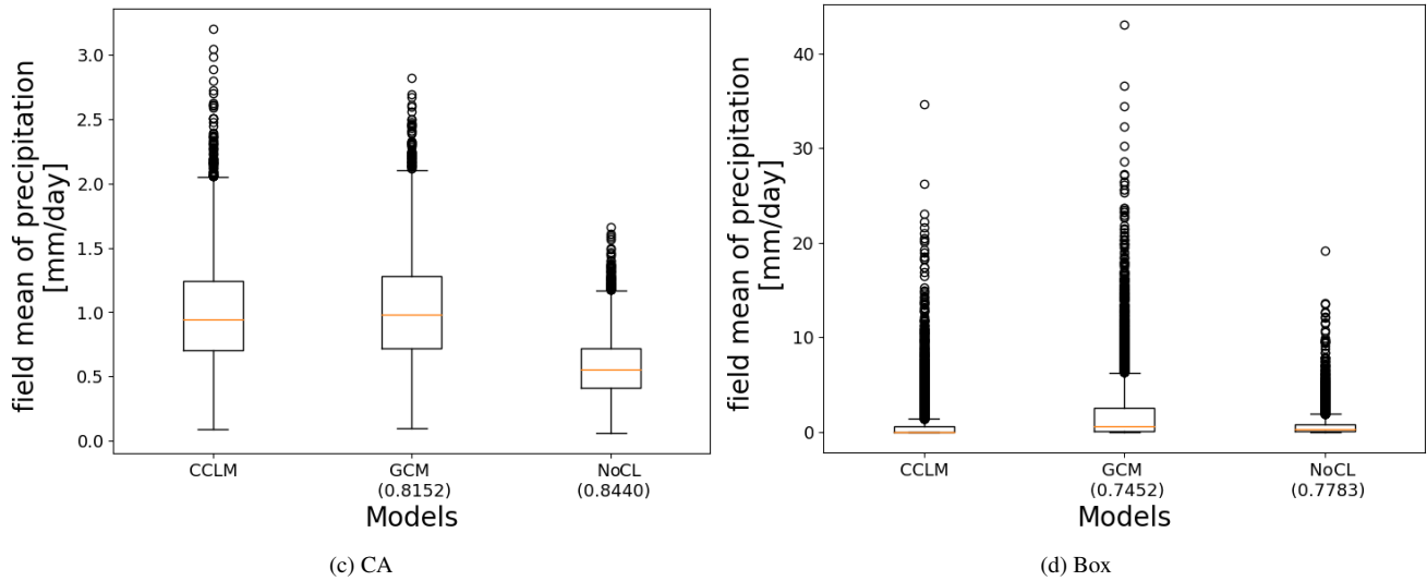
Figure 10. a) Mean absolute error (MAE) between the GCM(EC-Earth3-Veg) and the RCM (CCLM). GCM is remapped bilinearly to the 0.25 \times 0.25 grid. b) Added value (AV) or MAE reduction ( \text{MAE}(\text{EC-Earth3-Veg}, \text{CCLM}) - \text{MAE}(\text{CNN}, \text{CCLM}) ) for unconstrained method. c) and d) boxplots of averaged daily precipitation over the CA domain and the black box shown in a and b over North of Iran. Numbers in the parenthesis indicate the correlation coefficients of each model with respect to CCLM.
