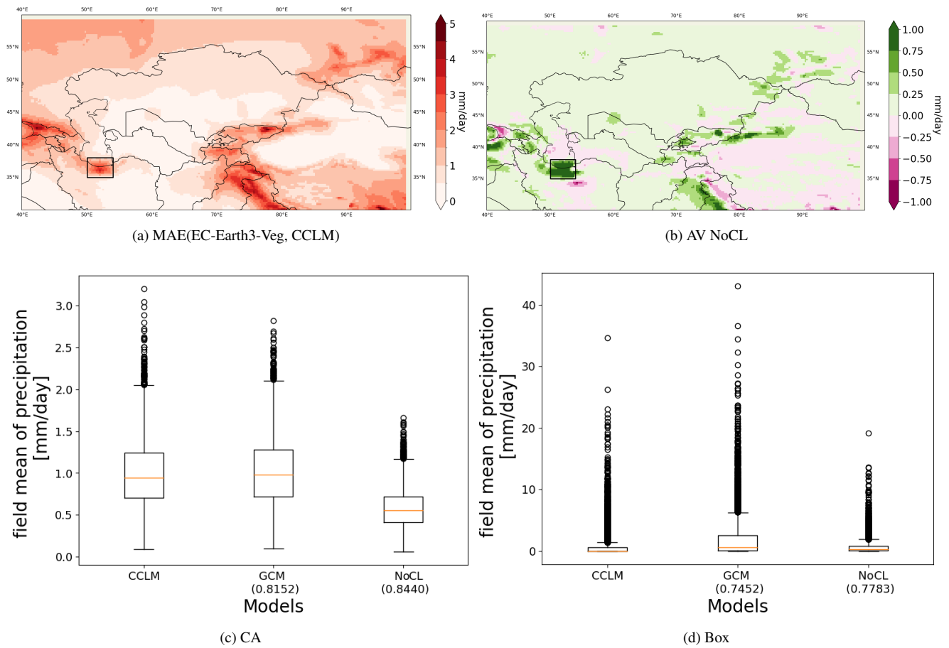
Figure 10. a) MAE of GCM (EC-Earth3-Veg) vs CCLM run. GCM is remapped bilinearly to the 0.25 \times 0.25 grid. b) Added value (AV) or MAE reduction ( \text{MAE}(\text{EC-Earth3-Veg}, \text{CCLM}) - \text{MAE}(\text{CNN}, \text{CCLM}) ) for unconstrained method. c) and d) boxplots of averaged daily precipitation over the CA domain and the black box shown in a and b over North of Iran. Numbers in the parenthesis indicate the correlation coefficients of each model with respect to CCLM.
