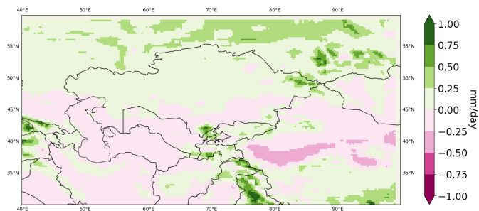
Figure 11. Added value (AV) or MAE reduction ( MAE(EC-MPI-ESM1-2HR, CCLM) - MAE(CNN, CCLM) ) for an unconstrained method that was not trained but applied to the SSP370 scenario.
