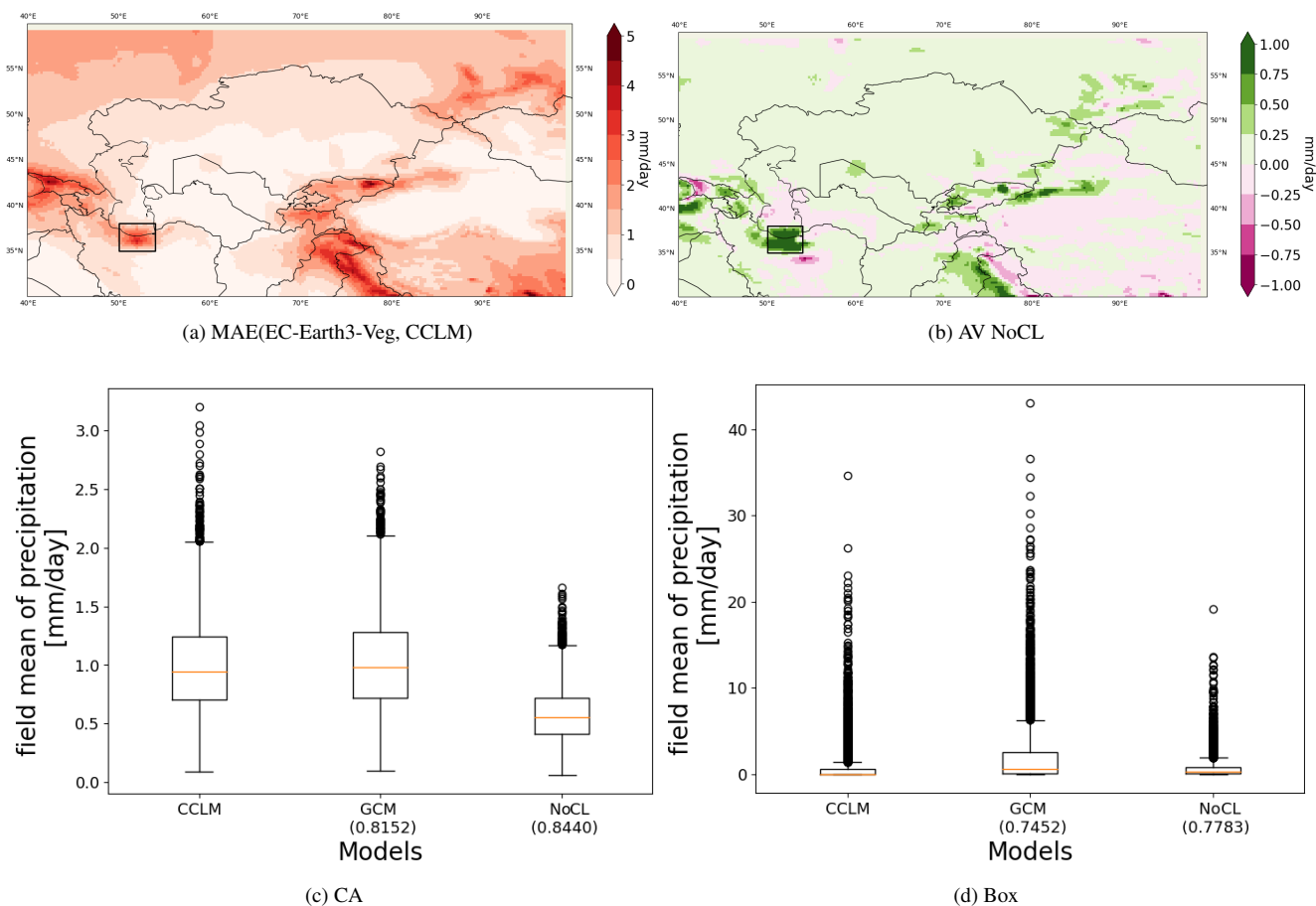
Figure 10. a) Mean absolute error (MAE of ) between the GCM(EC-Earth3-Veg) vs and the RCM (CCLM run ). GCM is remapped bilinearly to the 0.25 \times 0.25 grid. b) Added value (AV) or MAE reduction ( MAE(EC-Earth3-Veg, CCLM) - MAE(CNN, CCLM) ) for unconstrained method. c) and d) boxplots of averaged daily precipitation over the CA domain and the black box shown in a and b over North of Iran. Numbers in the parenthesis indicate the correlation coefficients of each model with respect to CCLM.
