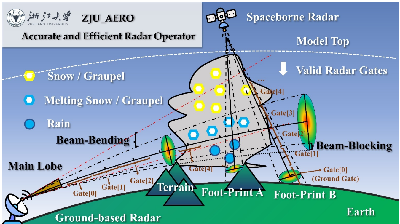
Figure 1: A conceptual graph illustrating the types of simulations that the Accurate and Efficient Radar Operator designed by Zhejiang University (ZJU-AERO) can accommodate. This graph visualizes the beam-bending and beam-blocking effects, which are taken into considerations by many radar operators designed for ground-based radars. For these radars, the sampling volume within the main lobe of the radar antenna patterns increases with the range of detection, as indicated by the area between the two dashed-
