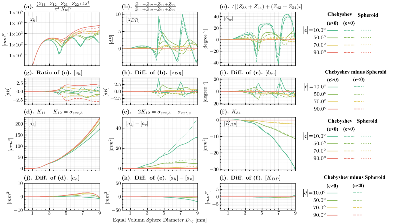
505 Figure 8: The SSP factors of intrinsic radar variables (indicated in the upper left corner) for the Chebyshev model and the spheroid raindrop models against the equal-volume-diameter of the liquid particles at the Ka band (35.5 GHz) and 283 K. Lines with different colours display the SSP factors for different elevation angles of the radar beam. Results of positive elevation angles for spheroids are indicated by solid lines while those of negative elevation angles are indicated by dashed lines. Since the results of spheroids have xy-plane reflectance symmetry, the negative and positive results are merged as dotted lines. The flatter auxiliary panels (g)–(l) (the second and the fourth rows) below the major panels (a)–(f) (the first and third rows) display the corresponding differences (or ratios) of optical properties between the Chebyshev model and the spheroid models, respectively. The first column shows horizontal polarization SSP factors ( [z_h] and [a_h] ) mentioned in Figure 6 and Figure 7, the second column shows SSP factors contributing to observed differential reflectivity ( [z_{DR}] and [a_h] - [a_v] ), and the third column shows the SSP factors contributing to the observed total phase shift ( [\delta_{hv}] and [K_{DP}] ).
