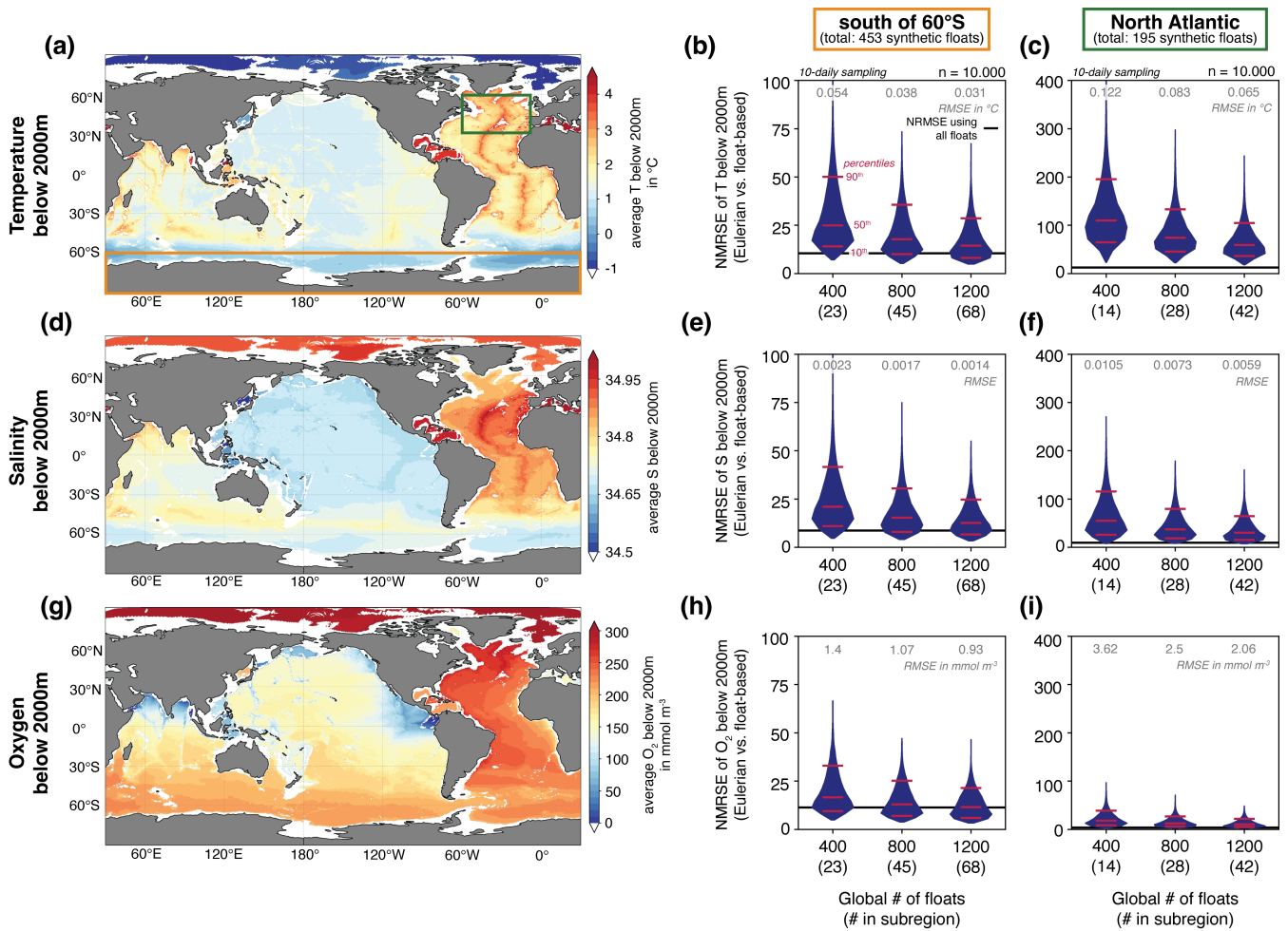
Figure 7. Case study "Deep ocean": (a) Temperature in °C below 2000 m and averaged over 2012-2017. (b) Violin plots of the normalized root mean square error (NRMSE) of the monthly temperature time series for the area south of 60°S (orange box in panel a) between the full Eulerian output and a float-based estimate using 10-day sampling and subsets of all synthetic floats corresponding to different global target float densities (x axis). The subsampling is repeated 10,000 times. The red horizontal lines denote the 90 th , 50 th , and 10 th percentile (from top to bottom). The black horizontal line corresponds to the NRMSE using all synthetic floats in the area. The RMSE is normalized by the area-weighted standard deviation of monthly mean temperature values of all grid cells in the area. The unnormalized RMSE is denoted in grey. (c) Same as (b) but for the North Atlantic between 30-60°N and 10-60°W (green box in panel a). (d)-(f) and (g)-(i) Same as (a)-(c) but for (d)-(f) salinity and (g)-(i) oxygen in mmol m -3 , respectively.
