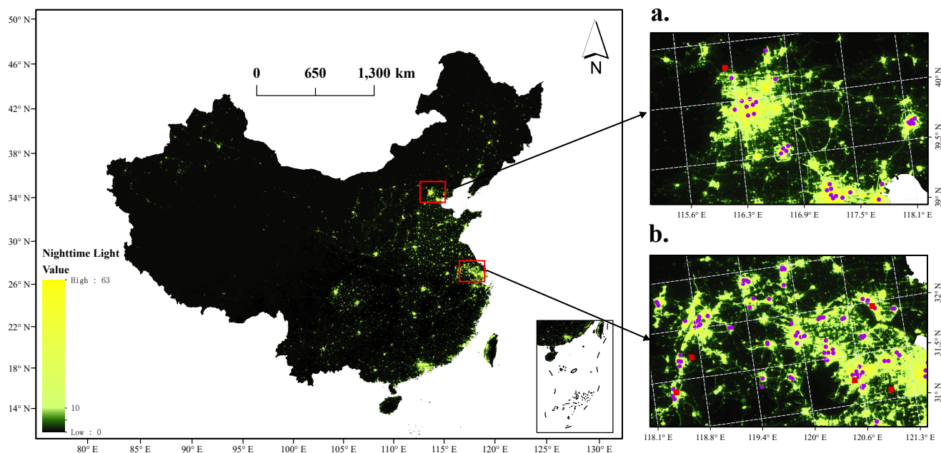
Figure 1. The left subplot shows the nighttime lights in the study area derived from V2.1 annual global VIIRS nighttime lights, with data averaged for the year 2020. The intensity of color corresponds to the level of urbanization, where brighter colors indicate higher urbanization levels. Subplots a and b display regions with significant local urbanization in NCP and YRD, respectively. In these subplots, purple dots and red rectangles are used to represent urban monitoring stations and rural monitoring stations, respectively.
