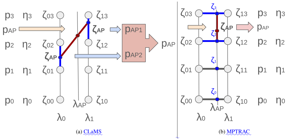
Figure 1. Concept of the interpolation illustrated in two dimensions for (a) CLaMS and (b) MPTRAC. Small circles indicate grid points, where the zeta and pressure values are given. Blue lines indicate the direction of the first interpolation and red lines indicate the direction of the second interpolation.
