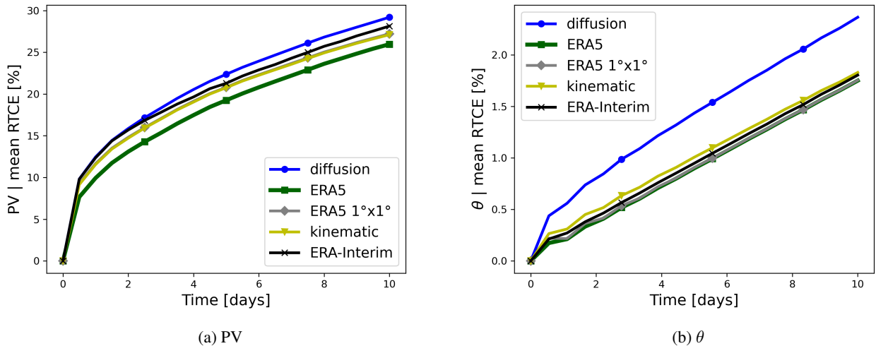
Figure 13. Evolution of the mean RTCE of a) PV and b) theta for different scenarios within a 10 days period. All scenarios are driven with MPTRAC. See the scenarios in Table 1 between MPTRAC-default and MPTRAC-def-erai for further details. The starting date is 06/01/2016. Only air parcels with an initial altitude above 360 K are considered.
