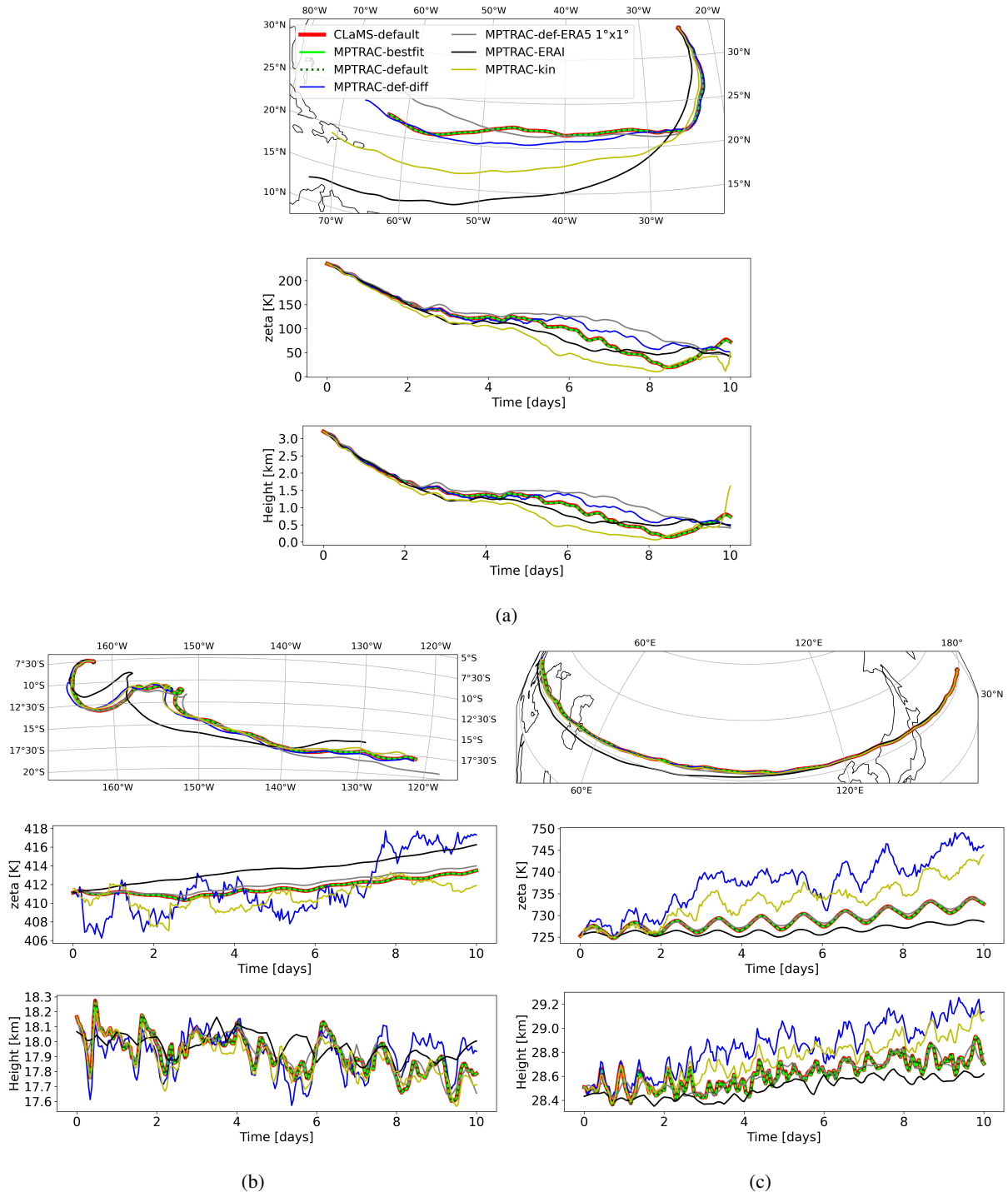
Figure 4. Selection Examples of trajectories calculated 10 days forward from 1 July 2016. Calculation results for different Different scenarios for in three examples layers are shown: The (a) Example for the troposphere, (b) example for the UTLS and (c) example for the lower stratosphere. For each trajectory the horizontal transport is shown in the upper panel. The vertical transport in the zeta coordinates and in log-pressure height is depicted below.
