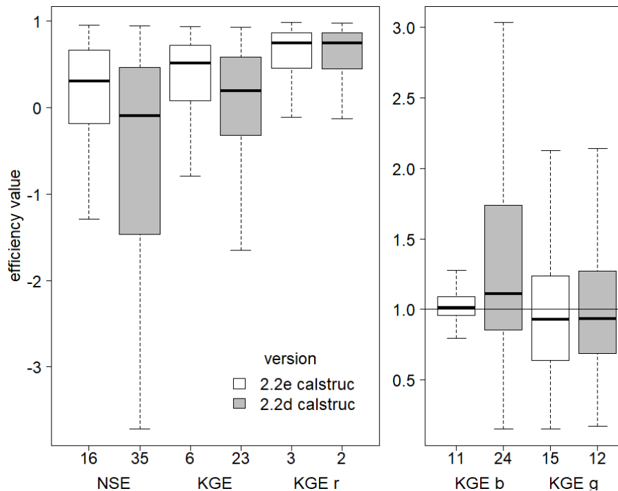
Figure 12. Efficiency metrics for monthly streamflow of the 230 gauging stations that differ between the streamflow data basis used for calibrating WaterGAP v2.2d and the new data basis used for v2.2e., with NSE , KGE and its components. All monthly observations available have been used to compute the metrics. Outliers (outside 1.5× inter-quartile range) are excluded but the number of stations that are defined as outliers is indicated at x-axis.
