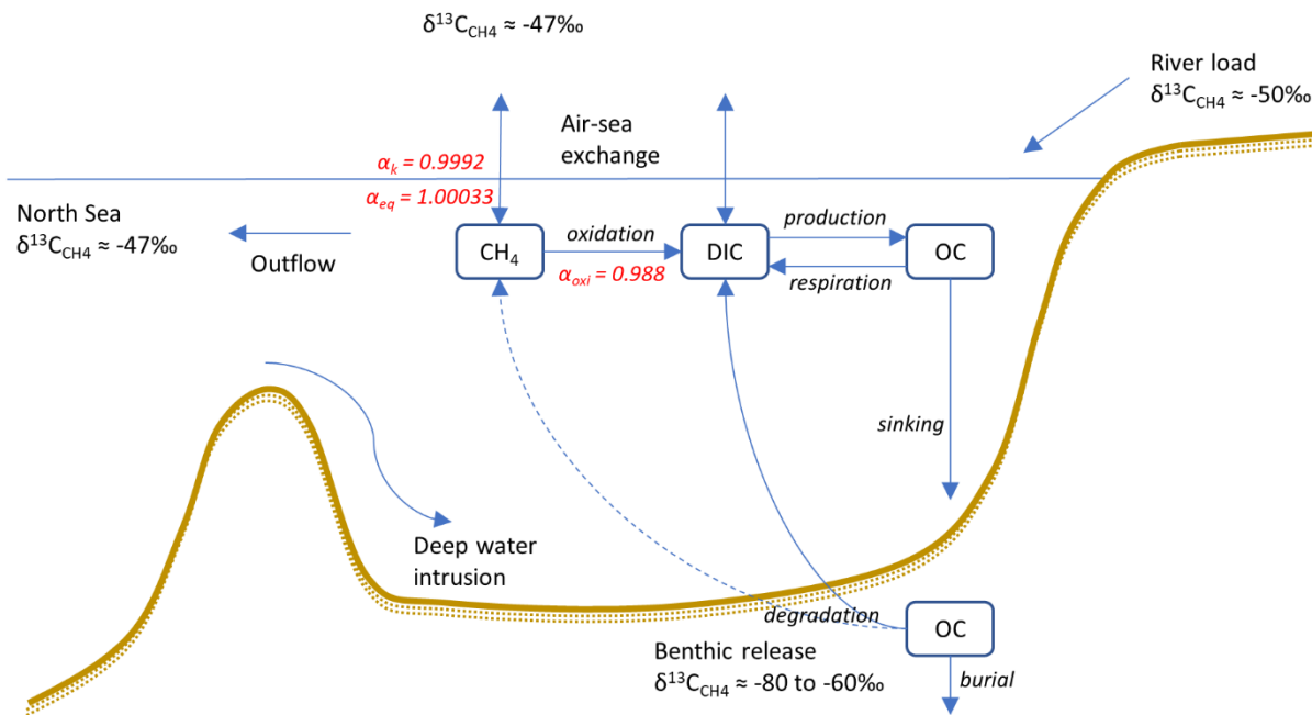
Figure 1: Conceptual sketch illustrating the processes involved in CH 4 cycling, including \delta^{13}C_{CH_4} values of end-members as well as \alpha values of transformation processes (see Sect. 2.3). The benthic release (dashed arrow) is not explicitly modeled, instead a preset calibrated value is used (see Sect. 2.3.5).
