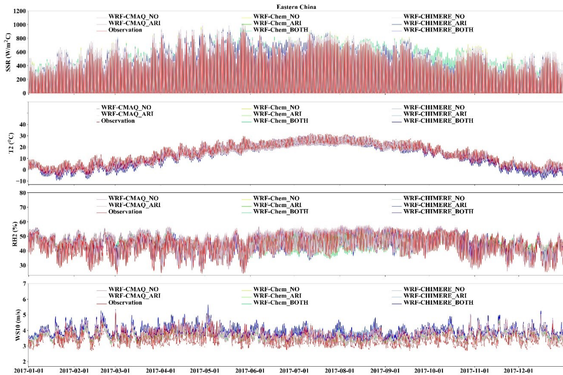
Figure 3. Time series of the observed and simulated hourly SSR, T2, RH2, and WS10 by coupled WRF-CMAQ, WRF-Chem, and WRF-CHIMERE with/without aerosol feedbacks over ECR in 2017.
