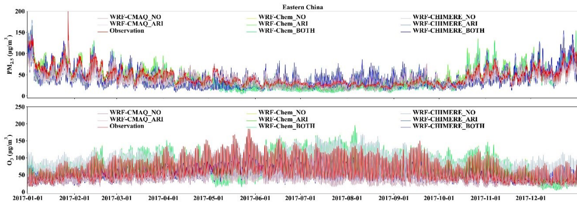
Figure 6. Time series of the observed and simulated hourly PM 2.5 and O 3 concentrations by WRF-CMAQ, WRF-Chem, and WRF-CHIMERE with/without aerosol feedbacks over ECR in 2017.
