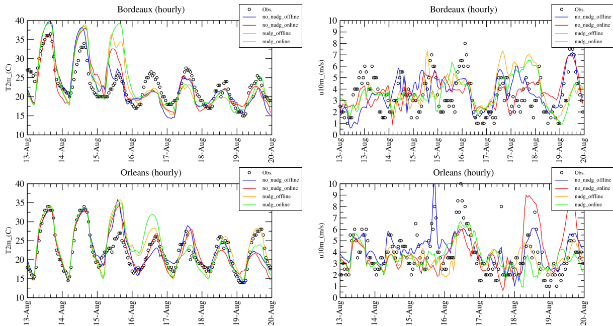
Figure 4. Time series of hourly 2m temperature ( ^{\circ}\text{C} ) and 10m wind speed ( \text{m}\cdot\text{s}^{-1} ) for the stations of Bordeaux and Orléans and for the period 13 to 20 August 2022.
