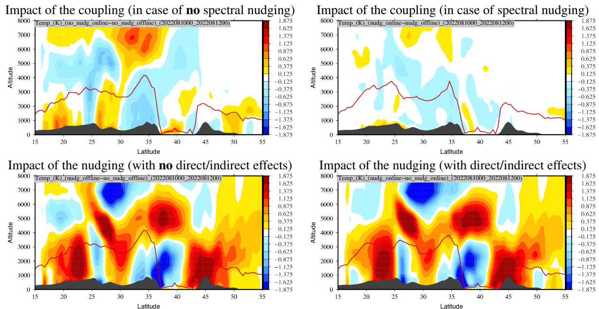
Figure 10. Vertical cross-section of differences of temperature ( ^{\circ}\text{C} ) between spectral nudging or not, coupling or not, and time averaged over the period 10 st :12 st August 2022. The red line represents the boundary layer height (m) of the simulation (a) if the difference is (a)-(b).
