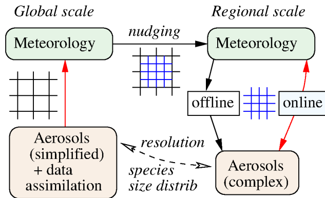
Figure 1. The paradox of the regional model nudged by a global model using other. The global model performs a meteorological simulation, generally including aerosol climatology to take into account the direct and indirect effects of aerosols. If the simulation is a reanalysis, there may also be data assimilation, such as optical thickness estimated from satellite observations. But the overall simulation will have included aerosols in the meteorological calculation. This global simulation will serve as a forcing for the regional simulation. The regional meteorological model will serve as a forcing tool, or will be coupled to the chemistry-transport model calculating aerosols. Aerosols are also taken into account, but at a different resolution. The black grid is the global model and the blue grid the regional model. The dotted arrow indicates that aerosols may not be the same species or have the same size distribution, depending on the chemistry-transport and climatology models used.
