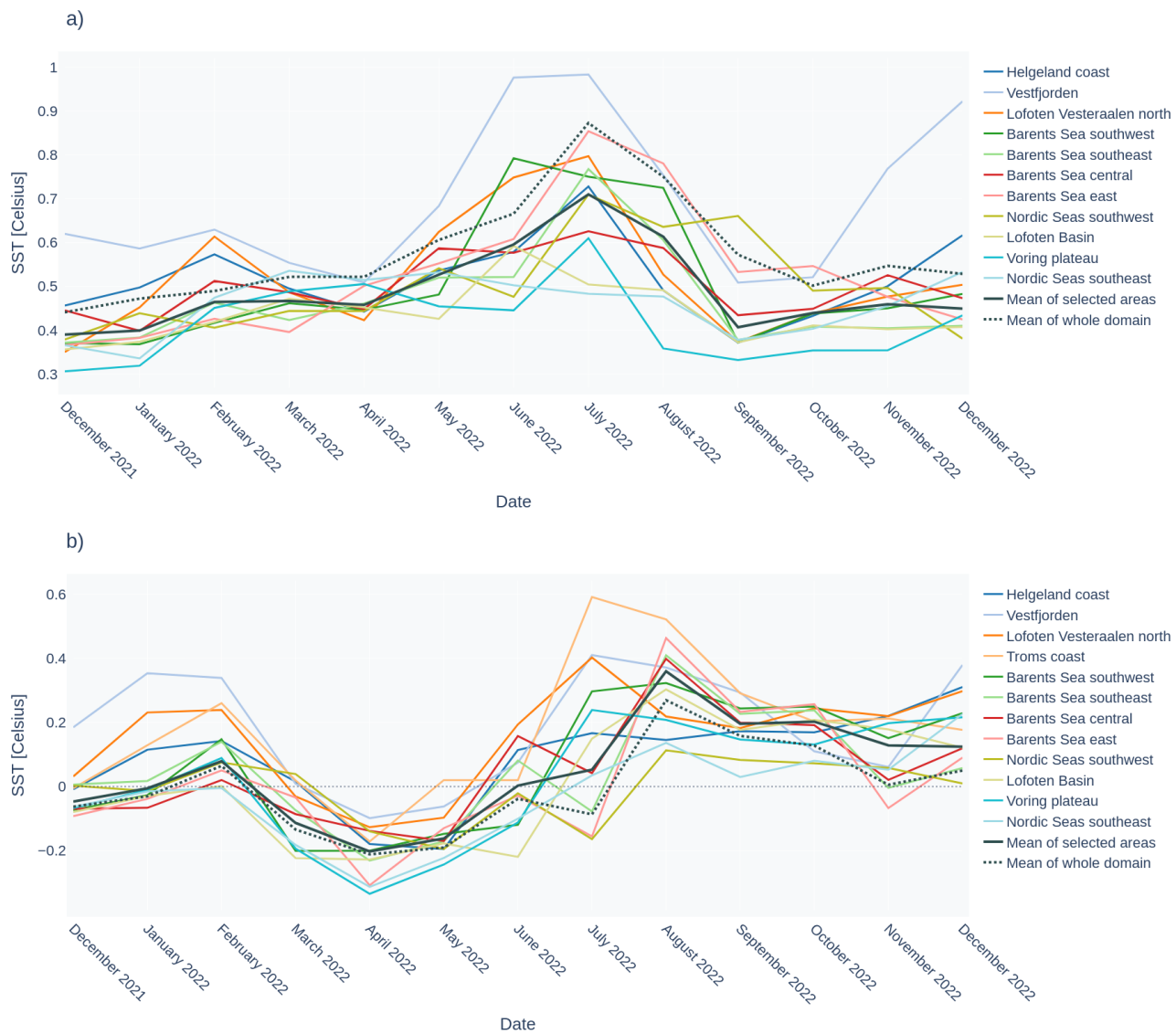
Figure 10. Time evolution of (a) RMSE and (b) ME for SST, separated for various regions in the model domain as defined by the colours in Fig. 5. For each available swath, Sentinel-3 SLSTR observations are compared with the model value that is closest to the satellite retrieval time in the 0-24 hours forecast range. Monthly averages of available data are shown.
