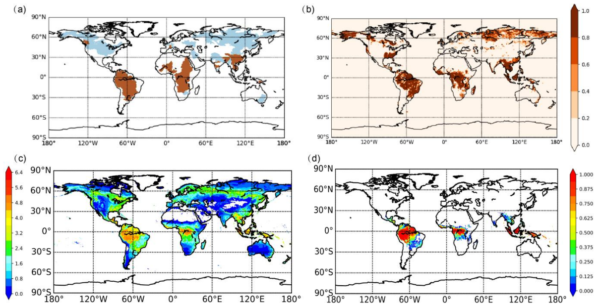
Figure S6 Distribution of overestimated river basins, leached soil, LAI, PFT. (a) is the simulation 30 results of weathering flux for river basins, where the brown color represents overestimation and the blue color represents underestimation. The data for this figure is derived from the runoff data provided by R_Park, the topographic data from s2 , and the adjusted erosion by observation data; (b) is the distribution of leached soil from Harmonized World Soil Database, and the values represent the percentage of each grid that contains that type of soil; (c) and (d) present vegetation 35 data from CESM (Community Earth System Model), specifically the Leaf Area Index (LAI) and tropical evergreen tree coverage, respectively.
