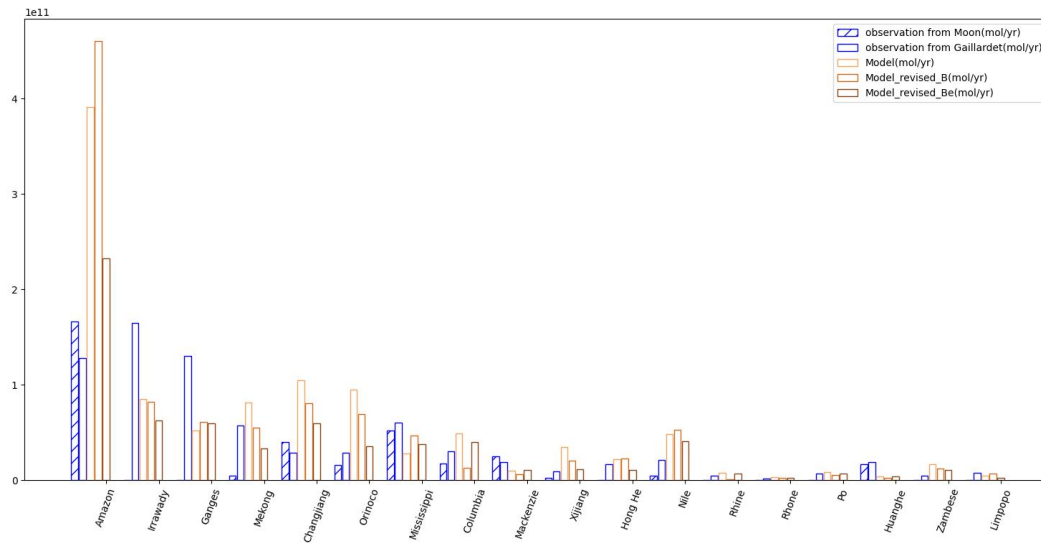
Figure S8 Histogram of silicate weathering fluxes for 18 river basins for which erosion rate from cosmogenic nuclide analysis was provided in (Wittmann et al., 2020). The blue hollow bars represent the observations from Gaillardet and bars with inclined lines represent the observations from Moon. Three different hollow bars in oranges represent the Park20 model result, revised by
