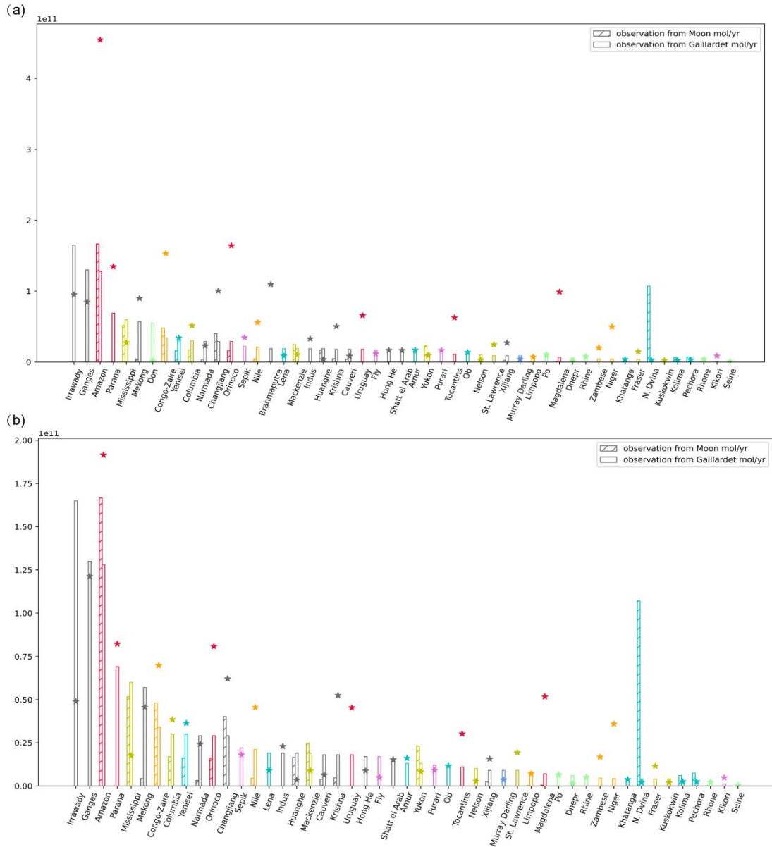
Figure S12 A comparison of the weathering flux across 51 basins as determined by the original Park20 model (a), revised model (b) and observational data. Observational results are shown as bar charts, sourced from studies by Gaillardet and Moon. The horizontal axis is arranged in descending order based on the observed river weathering flux, and rivers that are closely ranked may have small differences between (a) and (b). The simulated weathering flux is represented by pentagrams. Distinct colors differentiate the various regions as can be seen from Fig. 3b.
