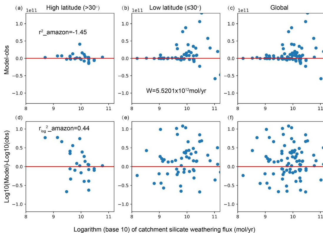
Figure S1 The difference between model calculated and observed silicate weathering fluxes for 81 large rivers over the world for model calculated with parameters provided in (Maffre et al., 2022). The upper and lower panels show model-obs and log(model)-log(obs), respectively. The left, middle and right panels show rivers in the mid- to high latitudes (more than half its river
