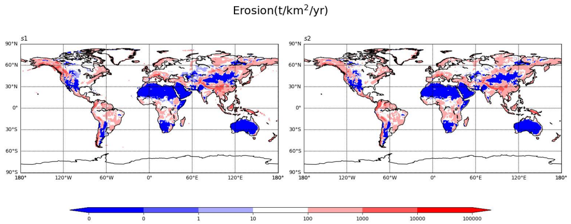
Figure S4 The distribution of erosion rate for the two slope datasets with runoff from Park
