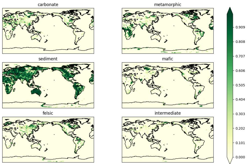
Figure S5 Distribution of lithologies modified from (Hartmann and Moosdorf, 2012).
