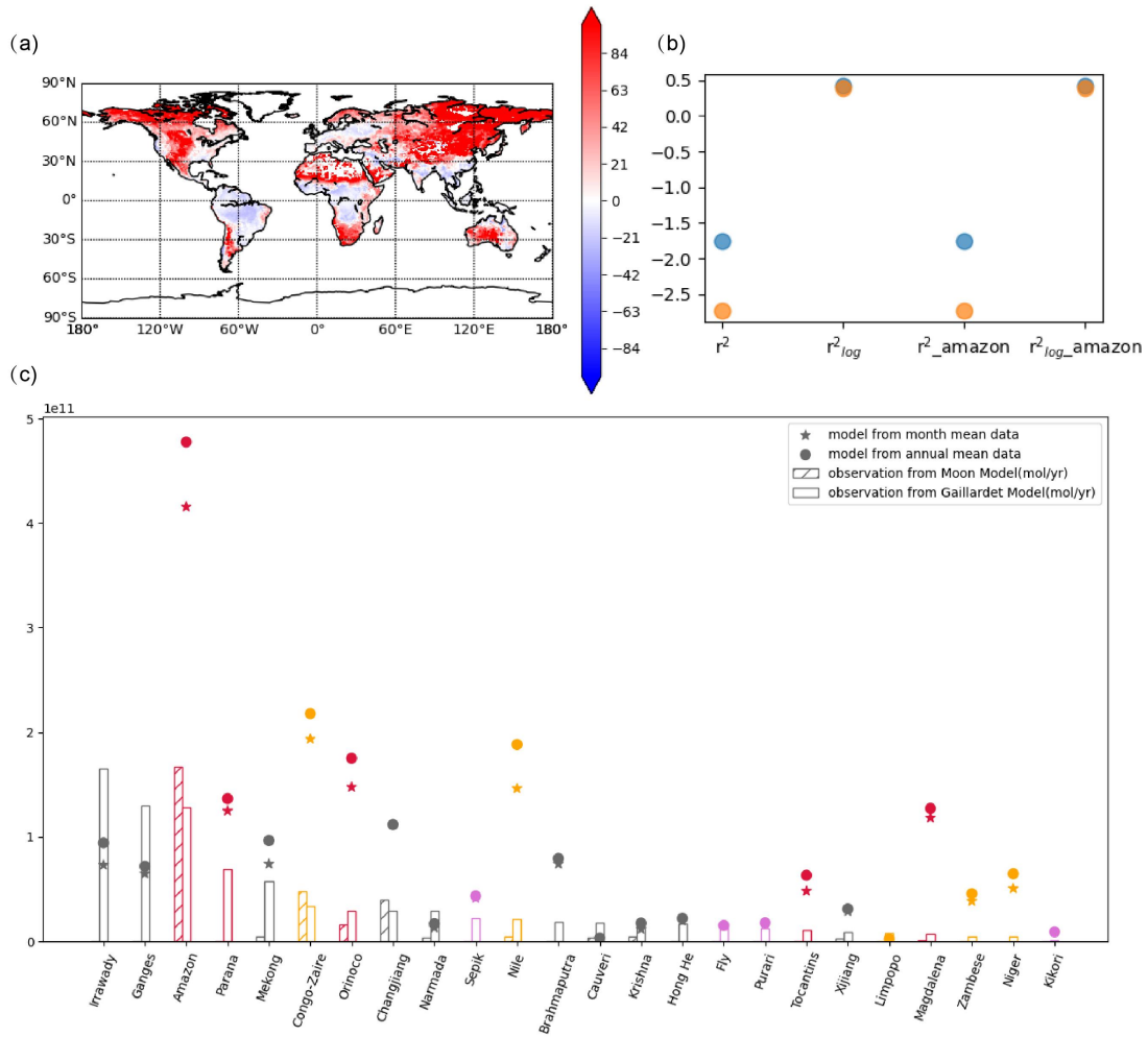
Figure S7 (a) is the percent of changes in silicate weathering flux with seasonal effect, and the negative numbers refer to the reduction of monthly average weathering fluxes compared to the annual mean weathering fluxes. (b) show scatter plots of r^2 or r_{log}^2 calculated, where x axis represents different metrics; blue points mean the result calculated by monthly mean climate data and orange mean the annual mean climate data. (c) is the histogram of silicate weathering fluxes for 24 large low-mid latitude river basins and the comparison between different data sources, month mean data and annual mean data respectively.
