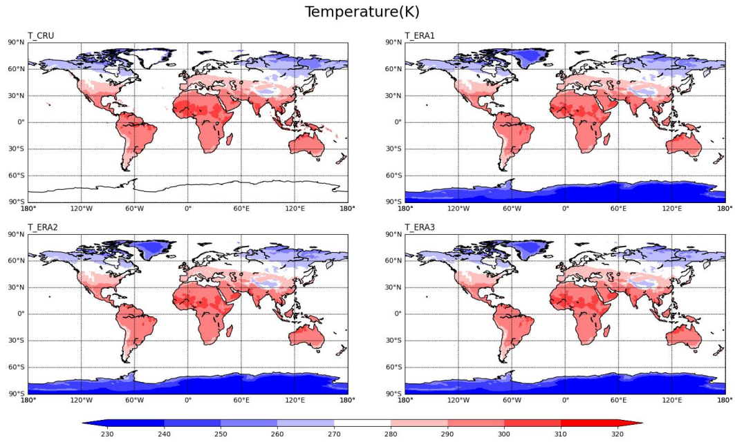
20 Figure S2 The distribution of temperature for the four datasets.
