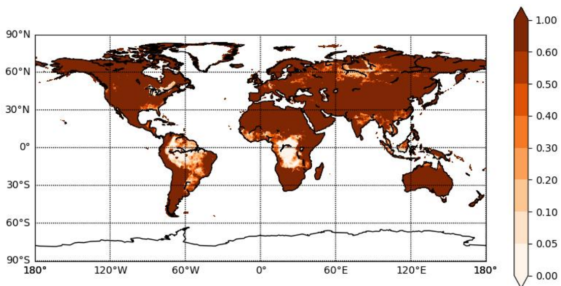
Figure S9 The concentration ratio of topsoil x_s from the Park20 model with R_Park runoff data, s2 slope data and erosion rate revised by TSS data.
