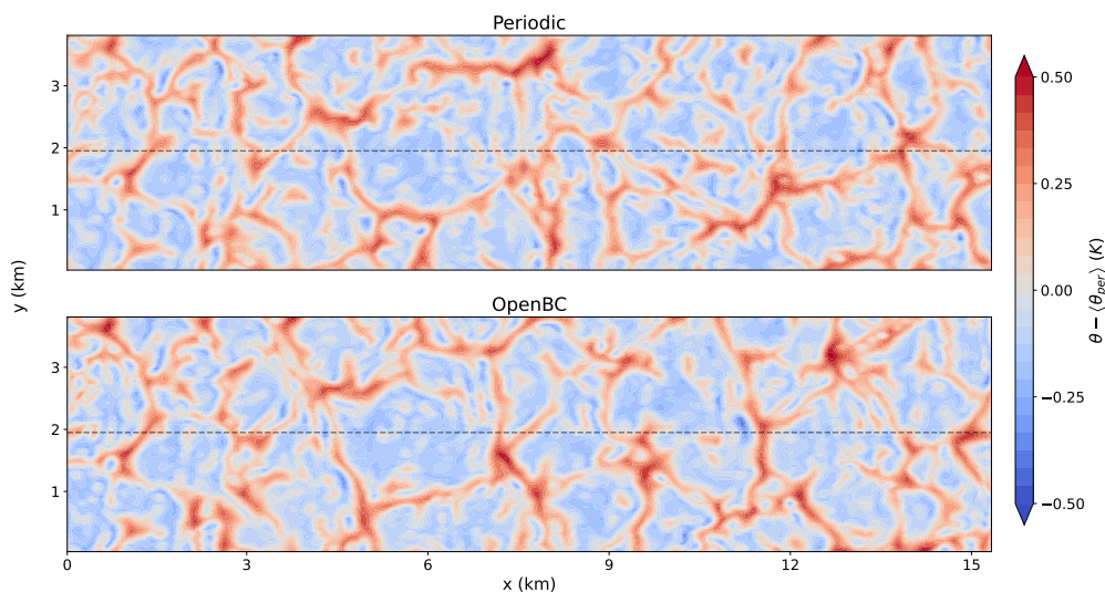
Figure 5. Horizontal cross-section of the potential temperature perturbation with respect to the periodic slab average at a height of 110m for the periodic simulation (top) and open boundary simulation (bottom). The dotted line shows the location of the xz cross-section shown in Fig. 6.
