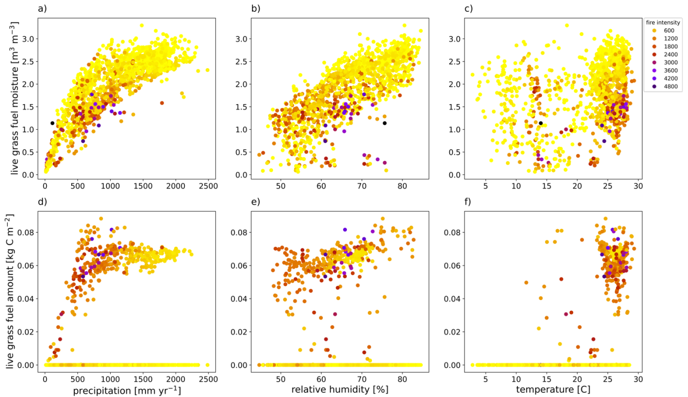
425 Figure 5. Association of fire intensity (colors; kW m -1 ) for live grass fuel moisture (m 3 m -3 ) with (a) precipitation, (b) relative humidity, and (c) temperature, and for live grass fuel amount (kgC m -2 ) with (d) precipitation, (e) relative humidity, and (f) temperature for fire intensities above 100 kW m -1 from the final ten years of a 300 year simulation in CLM-FATES across South America using a medium fuel drying parameterization.
