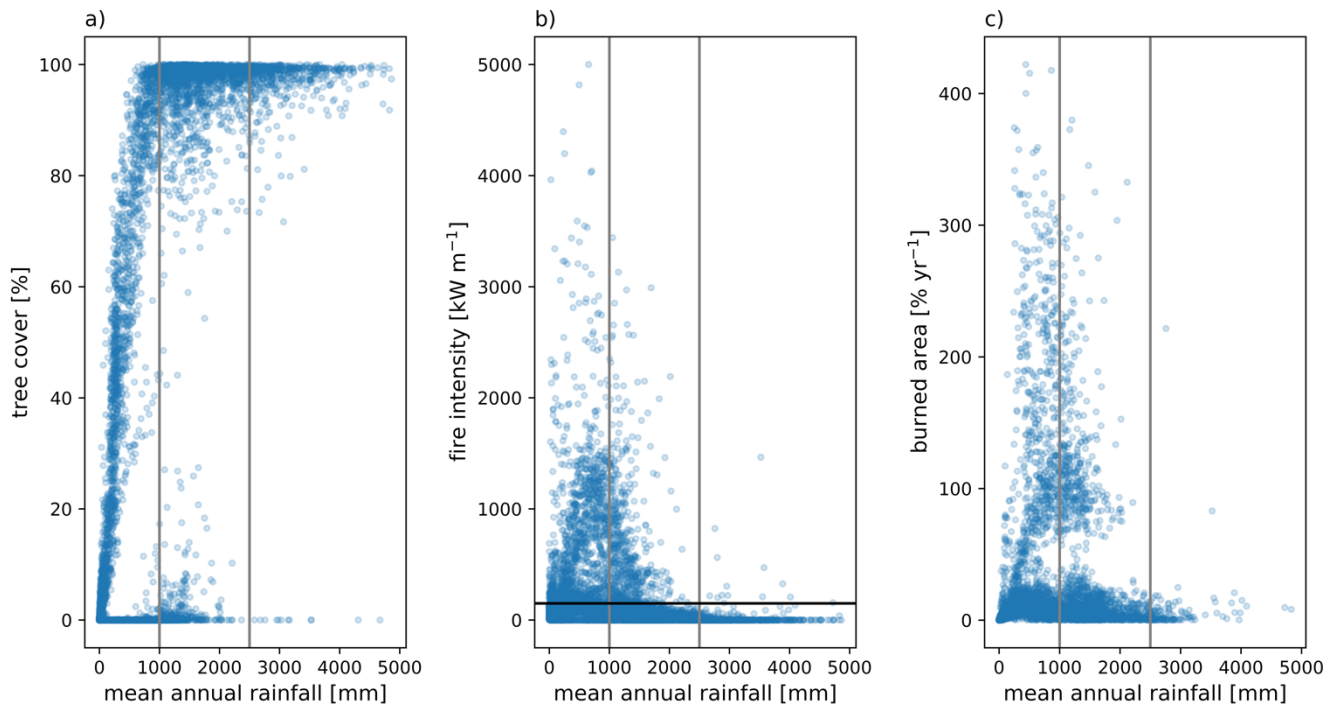
490 Figure 13. Simulated mean (a) tree cover, (b) fire intensity, and (c) burned area as a function of mean annual rainfall (MAR) (mm yr -1 ) from the final ten years of a 275 year CLM-FATES simulation across the tropics with active fire disturbance and a medium fuel drying parameterization. Grey vertical lines indicate 1000 and 2500 MAR. Horizontal black line in (b) indicates a fire intensity of 150 kW m -1 .
