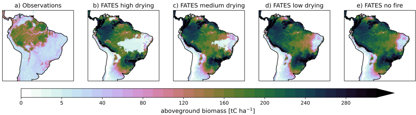
430 Figure 6. Aboveground biomass for (a) observations (Saatchi et al 2011), and for CLM-FATES using parameterizations with (b) high, (c) medium or (d) low fuel drying, and (e) without fire disturbance for the final ten years of 300 year simulations.
