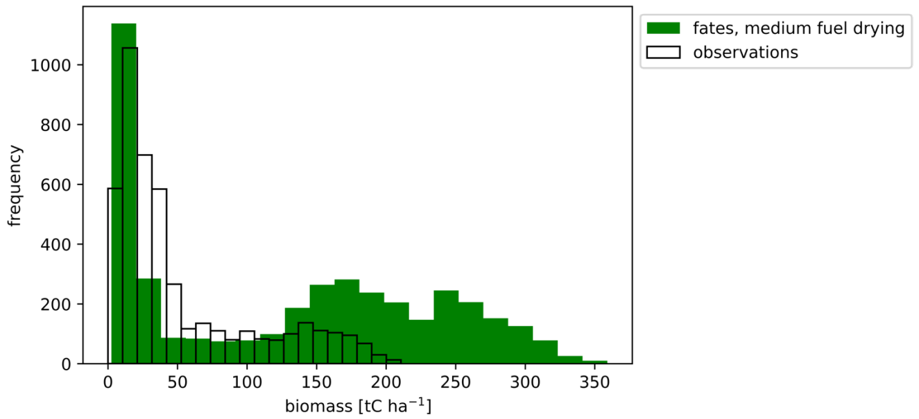
480 Figure 11. Mean aboveground biomass (tC ha -1 ) for the pan-tropics from observations (Saatchi et al 2011) (clear) and CLM-FATES (green) for the final ten years of a 275 year simulation with parameterizations for a medium fuel drying ratio.
