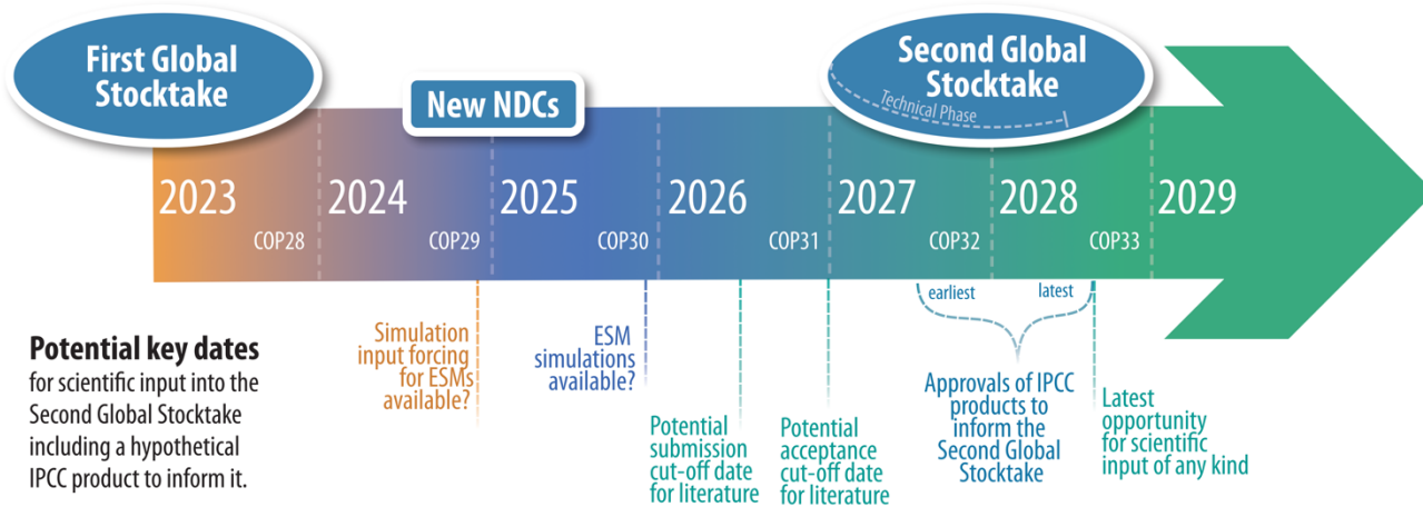
855 Figure 3 – A stylised timeline for scientific information and IPCC to inform the 2 nd Global Stocktake. Key dates are derived based on the global stocktake cycle and its modalities, including a technical phase for scientific input. The stylised timeline for IPCC products allows the establishment of a schedule for the design and execution of a new generation of ESMs simulations aimed at informing the relevant IPCC products. Note that cut-off dates are indicated relative to the earliest IPCC product approval timing and would move accordingly backwards for a later approval date.
