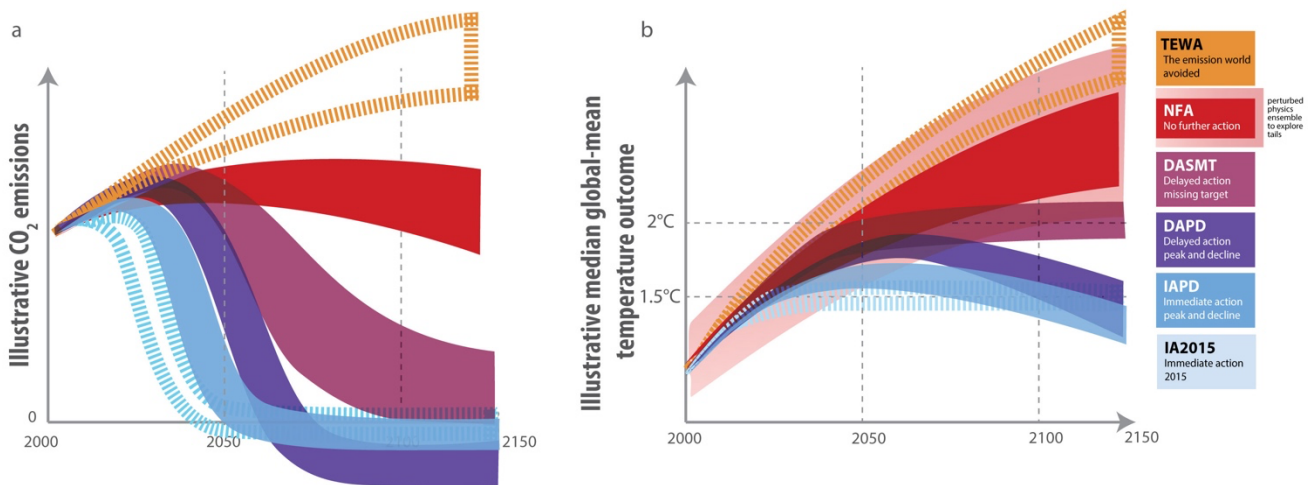
Figure 2 - Sketch overview of framing pathway categories for ESM simulations. Illustrative CO 2 emission trajectory ranges and corresponding global-mean temperature outcomes are shown in panel a and b, respectively. The temperature outcomes are approximate
