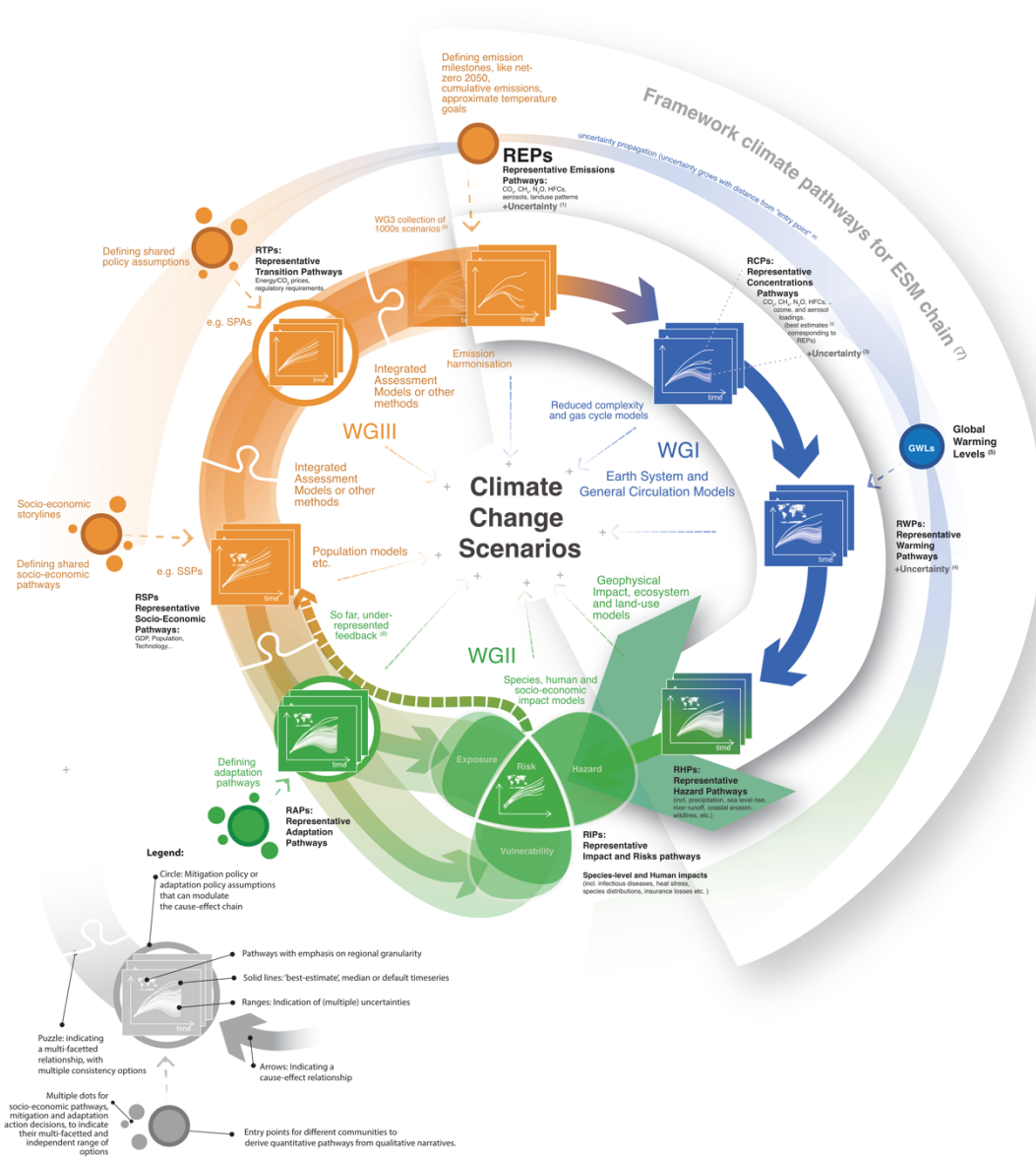
290 Figure 1 – Our conceptual overview of climate change scenarios, representative emission pathways (REPs) and the framework climate pathways. Scenarios are constructed from socio-economic, emission, concentration and impact pathways that are internally consistent with each other ('+' in middle). We propose anchoring the input for ESMs around 'Representative Emission Pathways' (REPs) ('1'), in contrast to anchoring around RCPs as was done in IPCC AR5 and IPCC AR6. However, the intention is to flexibly allow different 295 starting points for different communities. For the gas-cycles that are not represented in some ESMs, reduced complexity models can translate emission pathways to concentration pathways. The 'best-estimate' ('2') concentration projections in line with REPs can be labelled RCPs, although the 'representative pathways' across different subdomains (emissions, concentrations, socio-economic) do not necessarily have to be consistent. Furthermore, different models and approaches would translate emissions to concentrations differently, spanning an uncertainty range ('3'). 'Representative Warming Pathways' (RWPs) can provide another entry point into scenario design, closely aligned by a consideration of 'Global Warming Levels' (GWLs) ('5'). If derived from REPs, the range of derived warming pathways would represent 300 both gas-cycle and climate feedback uncertainties ('4'). Biogeophysical hazard models, ecosystem and land-use could then be driven by the
