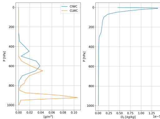
570 Figure 3. Graphical output of Listing 3, showing atmospheric profiles from ERA5 reanalysis for the nearest grid point to a location in Southern Italy (longitude 16.04°; latitude 39.44°) on 16 May 2023 at 18:00 UTC. Left: Cloud liquid water content (CLWC) and cloud ice water content (CIWC). Right: ozone mass mixing ratio.
