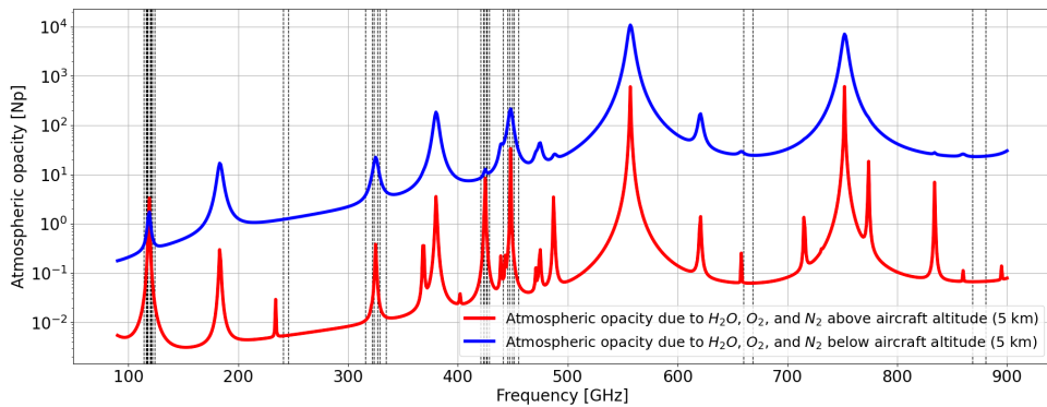
Figure 6. Top: downwelling and upwelling T_B simulating aircraft observations at respectively zenith and nadir from 5 km altitude (gas absorption model: R22; surface emissivity equal to 1). Bottom: Atmospheric opacity ( \tau ) corresponding to dominant gases ( H_2O , O_2 , and N_2 ) computed for the uplooking and downlooking views. All the features correspond to H_2O absorption but the following, due to O_2 : 118, 368, 424, 487, 715, 773, 834 GHz. Input profile from the radiosonde launched from Camborne (UK) on 22 July 2021 at 12:00 UTC and retrieved from the Wyoming Upper Air Archive. Vertical black lines indicate the ISMAR channel frequencies.
