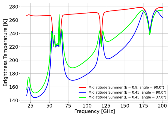
Figure 5. Graphical output of Listing 5, showing upwelling T_B spectra computed for a predefined climatological profile (Midlatitude Summer) at 90^\circ and 37^\circ elevation angles with constant surface emissivity values of 0.9 and 0.45.
