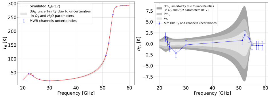
825 Figure 11. Left: Zenith downwelling T_B spectrum (red line) computed from one radiosonde launched from the ARM mobile facility during TCAP, Cape Cod, MA, USA (2012-08-26 16:58 UTC). Blue points and bars indicate the nearly simultaneous measurements from the colocated MWRP at 12 frequency channels and their calibration uncertainty. Right: Simulations minus observations at the 12 channels (blue points) with the instrumental calibration uncertainty (blue bars), together with the estimated uncertainty for zenith downwelling T_B ( \sigma(T_B) ) due to the uncertainty in absorption model spectroscopic parameters 830 (at 1-, 2-, and 3-sigma levels).
