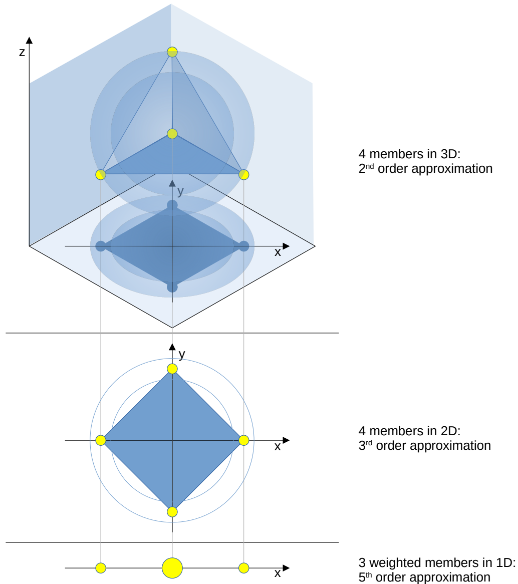
Figure 1. 4 tetrahedron-shaped ensemble members (yellow dots) in a 3-dimensional space (top) represent a second-order approximation of a standard normal distribution (with the spherical isosurfaces shown in shadow). The same 4 members form a square in 2 dimensions (middle), producing a third-order approximation. By projecting further into 1 dimension (bottom) and by assigning proper weights, a fifth-order approximation is obtained.
