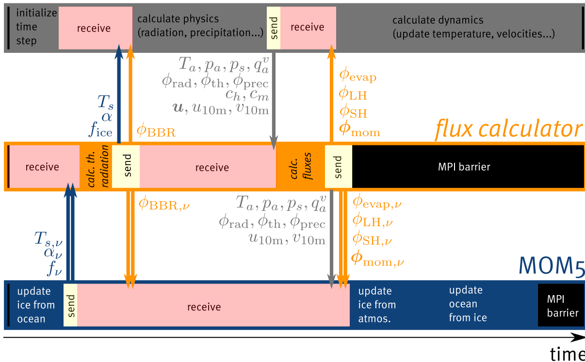
Figure 5. Schematic sequence diagram for one coupling time step. The two model components, MOM5 and CCLM, are visualized as the blue and grey blocks, respectively. The flux calculator is represented as the orange block. The calls of the coupling library routines are marked in light red for the blocking receiving function and in light yellow for the non-blocking send routine. Areas with the color corresponding to the particular model (blue and grey) mark the normal operation of the models. The simulation time is runs from left to right. The scaling of the time axis is just illustrative and not quantitatively true. Arrows illustrate the data exchange of the spelled out quantities explained in Tab. 1, where double arrows stand for surface-type dependent fields, i . Italic names denote fluxes that entirely calculated by e. one communicated field for each surface type. The colors of the flux calculator symbols represent the component from where they originate. For more description see the main text.
