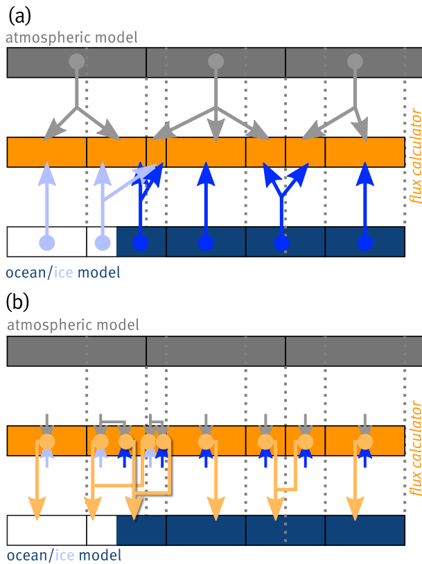
Figure 4. Coupling the models via the exchange grid and the flux calculator. Panel (a): State variables, calculated in the respective models (marked by the filled circles) , are communicated to the flux calculator (as visualized by the arrows) without averaging. Panel (b): Fluxes are calculated on the exchange grid and subsequently communicated to the bottom model.
