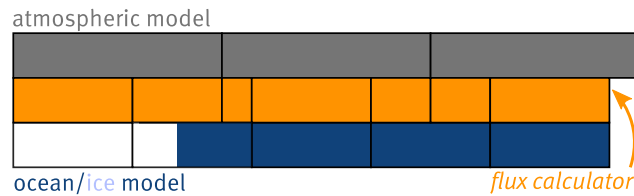
Figure 3. Introduction of the exchange grid ( orange boxes ) on which the flux-calculator flux calculator is acting.
