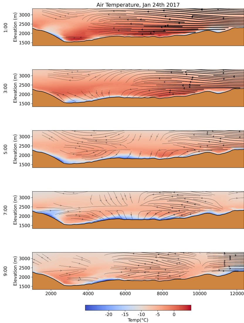
Figure 9. The development and diffusion of surface cooling for an alpine valley during dawn. The plot shows a small area of the 250m Swiss Alp domain introduced in section 3.5.3.4. The local time is indicated on the y-axis label. Wind vectors are plotted for wind directions along the transect. Thicker vectors indicate higher wind speeds, and winds below 0.2 m s -1 are not plotted.
