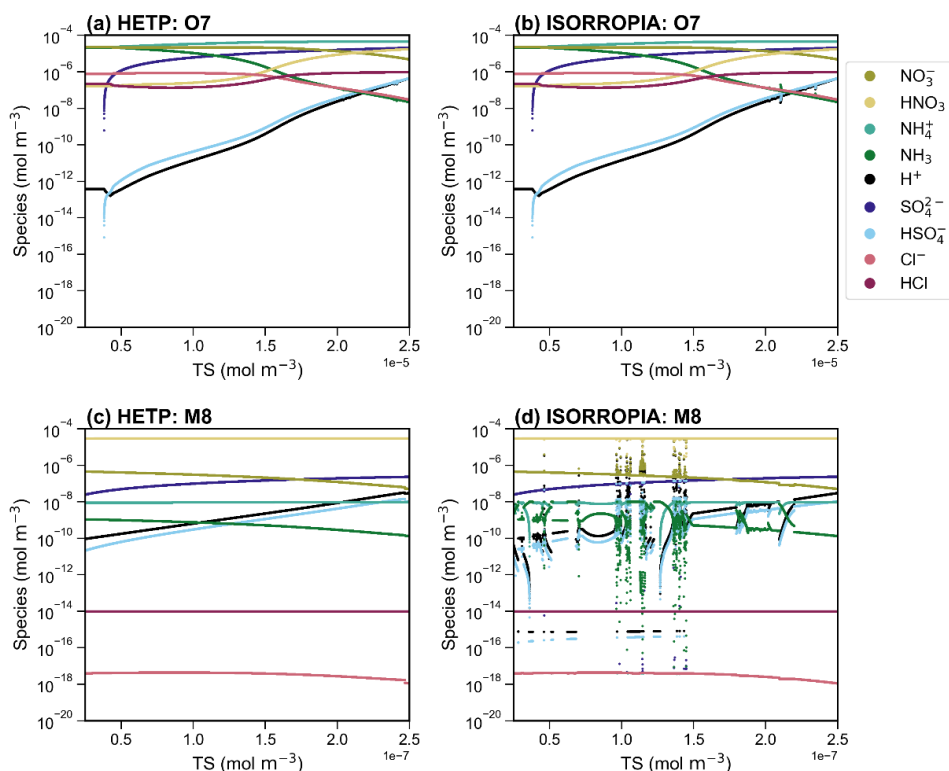
Figure 22: A side-by-side comparison of the output from HETP (left) and ISORROPIA (right), for the chemical subspace CALCO7 (a-b) and CALCM8 (c-d). All input species are held constant, except the total available sulfate (TS) which is varied over 10,000 sets of initial conditions. The air temperature and relative humidity are 306 K and 35% respectively, for all test cases in the figure. The convergence criteria are consistent between both solvers (see text).
