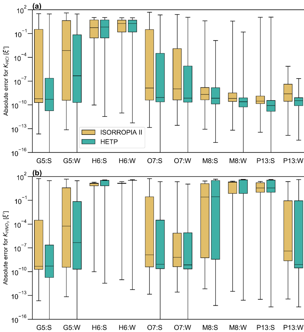
Figure 6: A box and whisker plot of the absolute error \xi' = |\log(K_{calc}) - \log(K_{true})| for (a) K_{HCl} and (b) K_{HNO_3} . The summer season is denoted by ‘:-S’ and the winter season is denoted by ‘:-W’ in the x-axis labels. \xi' is calculated from a set of 10,000 test cases in each season (obtained from the GEM-MACH air-quality model). \xi' shown in the figure for M8 and G5 correspond to the scatter plots shown in Fig. 5. The median \xi' is represented by the solid black line in the center of each box, and the 25 th and 75 th percentiles correspond to the bottom and top of each box respectively. The whiskers give the maximum (top) and minimum (bottom) of \xi' .
