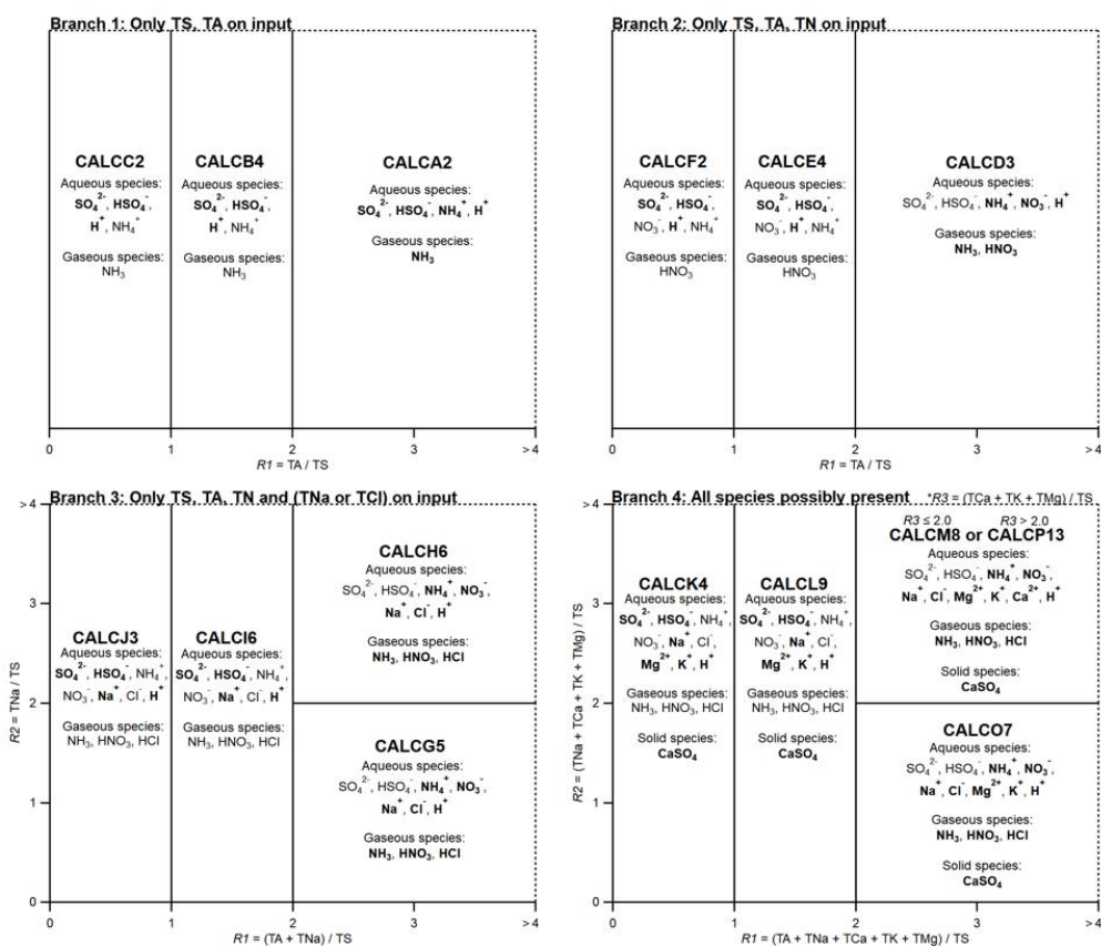
Figure 11: Domains of the systems of equations, based on ISORROPIA. For Branch 3, each of TS, TA and TN > tiny, as well as one (or both) of TNa and TCl. For Branch 4, each of TS, TA and TN > tiny, as well as one (or all) of TMg, TK and TCa – thus Branch 4 does not necessarily require TNa or TCl > tiny. However, it should be noted that for a solution to be possible, subcases CALCH6 , CALCG5 , CALCM8 , CALCO7 and CALCP13 do require TCl > tiny. The dashed lines in the figure implies that the domain extends infinitely in the direction of increasing R1 or R2 . For example, in Branch 1, 0 \leq R1 < \infty , but in the figure R1 only extends to 4, and subcase CALCA2 extends for all \text{TA}/\text{TS} > 2.
