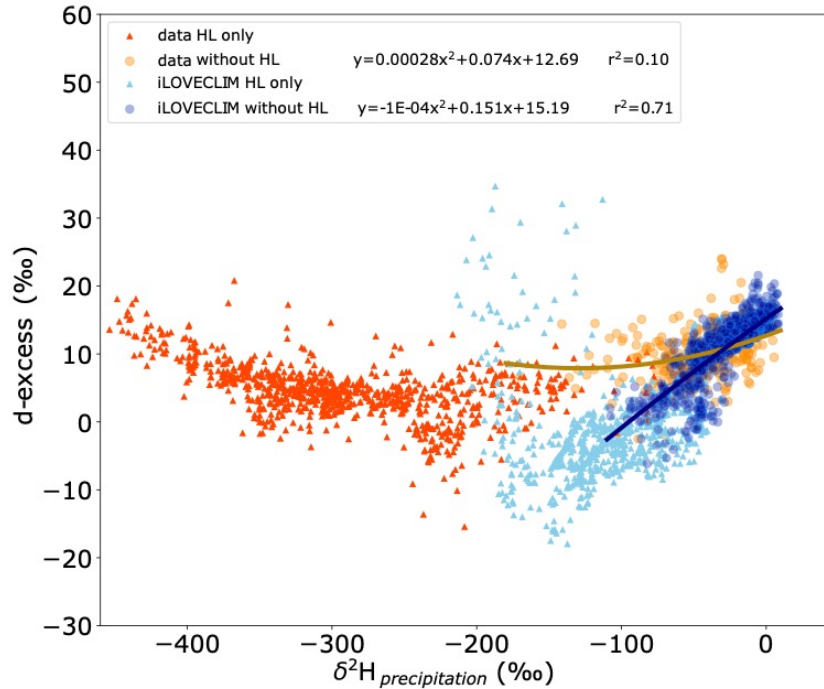
330 Figure 4: Global relationship between d-excess and \delta^2\text{H} in precipitation. High latitude values (above 60^\circ\text{N} and below 60^\circ\text{S} ) are presented with the red triangles for the data and with the light blue triangles for iLOVECLIM. Data for other regions are presented with the orange circles for the measurements and with the dark blue circles for the model. Regression curves for the data and the model, without high latitudes values, are also shown in orange and dark blue.
