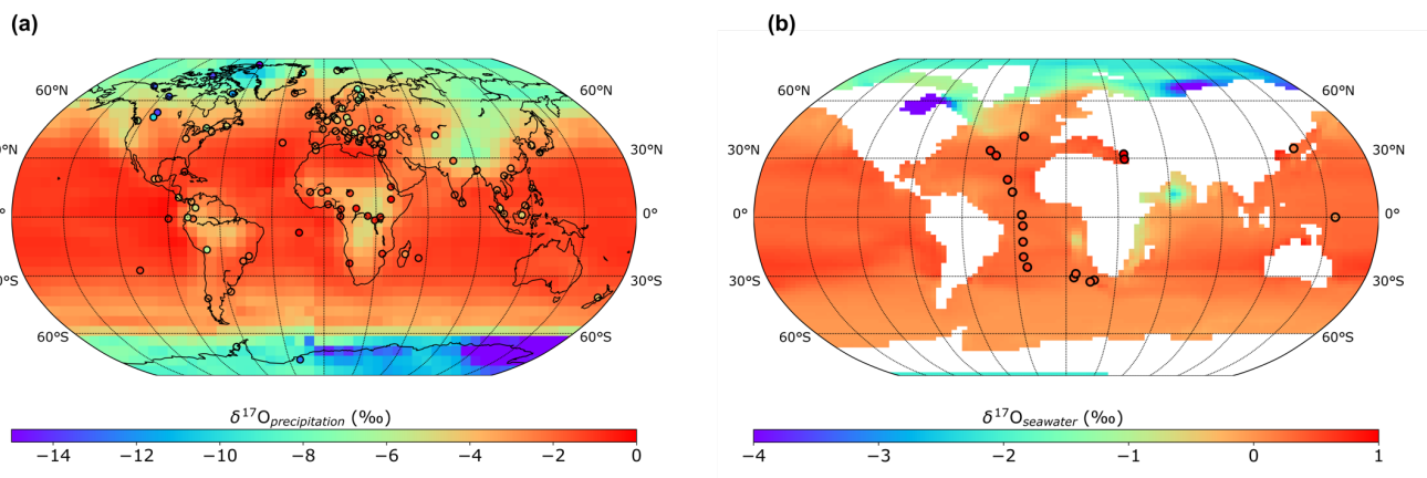
620 Figure A1: Mean annual spatial distribution of the iLOVECLIM modelled (a) \delta^{17}\text{O}_{\text{precipitation}} and (b) \delta^{17}\text{O} of ocean surface. Model results are compared to observations (in circles).
