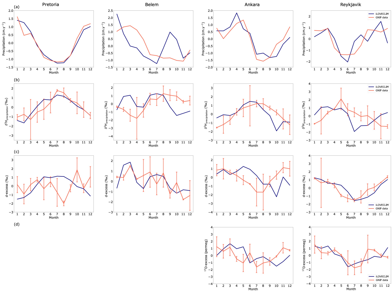
390 Figure 7: Monthly evolution of (a) precipitation, (b) \delta^2\text{H}_{\text{precipitation}} , (c) d-excess and (d) ^{17}\text{O} -excess at several stations (different columns for Pretoria, Belem, Ankara and Reykjavik). The red line is the GNP data measured at the station and the blue line is the iLOVECLIM model result at the corresponding location. The data and model results have been normalized. The error bars for the data are also shown at 2\sigma .
