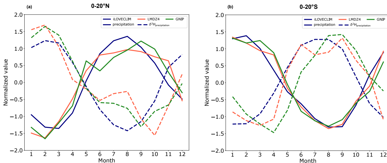
Figure 8: Seasonal variations of the mean precipitation and \delta^2\text{H}_{\text{precipitation}} in the tropics, from 0-20°N for (a) and from 0-20°S for (b). The values have been normalized, the solid lines represent the precipitation and the dashed lines the \delta^2\text{H}_{\text{precipitation}} . The blue curve presents the iLOVECLIM values, the red curve is for LMDZ4 and the green curve corresponds to the GNP data.
