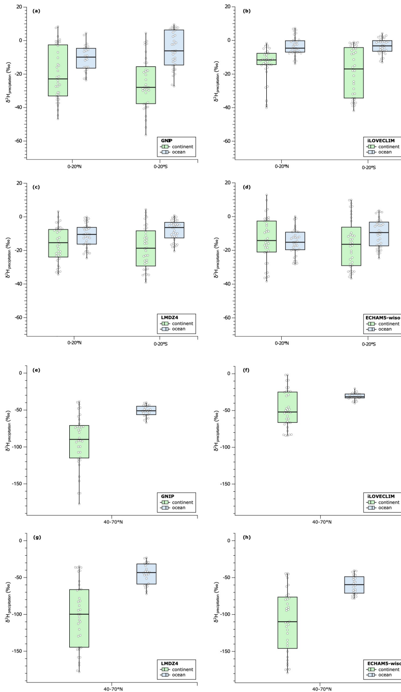
Figure 11: Box plots of the \delta^2\text{H}_{\text{precipitation}} over the continents (in green) and oceans (in blue). The panels (a) to (d) present values between 0-20°N and 0-20°S for (a) GNIP data, (b) iLOVECLIM, (c) LMDZ4 and (d) ECHAM5-wiso. The panels (e) to (g) present values between 40-70°N for (e) GNIP data, (f) iLOVECLIM, (g) LMDZ4 and (h) ECHAM5-wiso. The horizontal line in the box plots corresponds to the median value.
