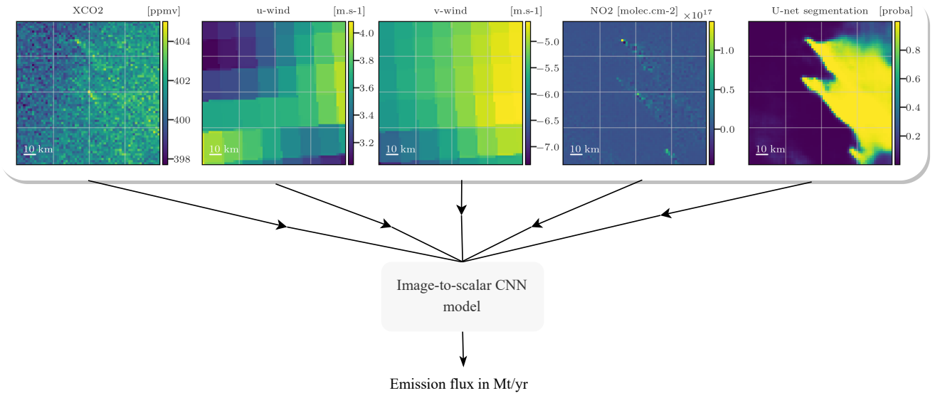
Figure 4. The XCO_2 -Various fields: XCO_2 , ancillary data winds, segmentation results and NO_2 , and emissions (of the central plume) emissions are used as inputs by a CNN that learns to estimate the emissions associated to the central plume concealed under the background. Note that the combination of NO_2 and segmentation results as inputs is never assessed in this manuscript.
