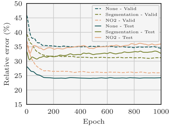
Figure 10. Evolution during training of the validation and test relative errors between the true emissions of Boxberg and the predictions of the CNNs. Specifically, for each epoch , the need of this experiment, new models being trained are trained and employed to predict the emissions corresponding to the validation and test fields at each epoch. Three models are considered: each is trained with the XCO 2 field and the winds as inputs. Two of the models additionally assimilate the NO 2 field or the predictions of the segmentation model. The validation error decreases monotonically with the number of epochs, while the test error does not, which suggests overfitting of the model.
