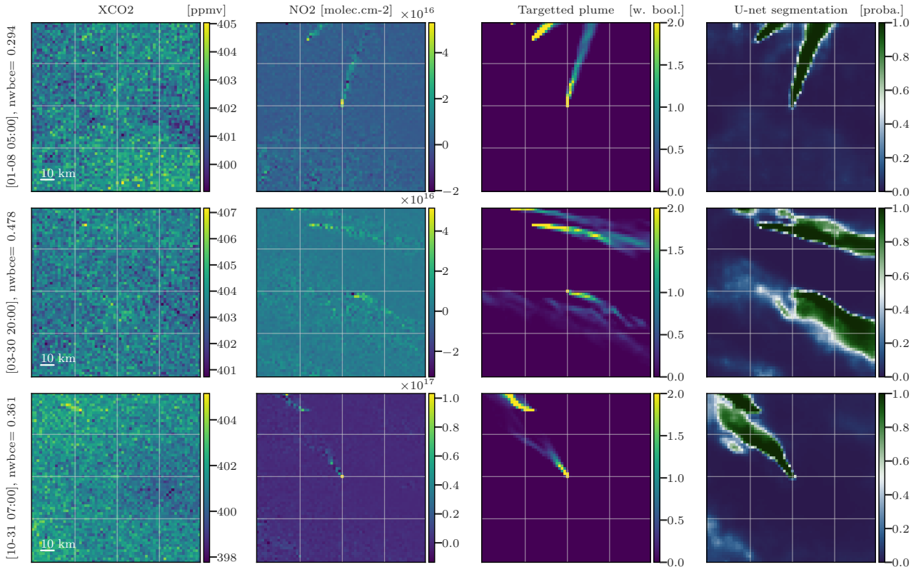
Figure 3. Examples of the U-net CNN model application on images centred at Turow. The first, second, third and fourth columns represent the XCO 2 images, NO 2 images, weighted Boolean plumes and U-net predictions as probability maps, respectively. All times are in UTC.
