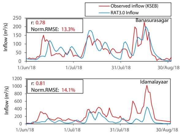
705 Figure 11: RAT hydrographs comparing observed inflow at Banasurasagar and Idamalayaar dam (red) against hydrologic model inflow by RAT using VIC (blue) during the 2018 Kerala floods. After Suresh et al. (2023). See Fig 12 for a map of Banasurasagar and Idamalayaar dam in Kerala.
