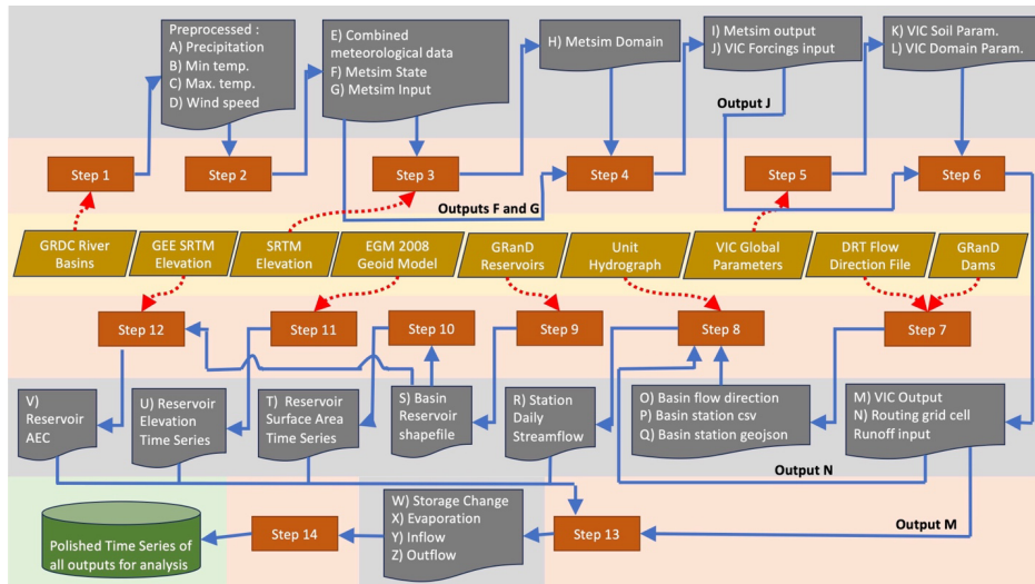
Figure 4: Workflow of RAT 3.0 with all the different steps listed in Table 1. The yellow layer shows the user inputs, the orange layer shows the flow of different steps or processes, and the grey and green layers show the intermediate and final outputs produced by RAT 3.0, respectively.
