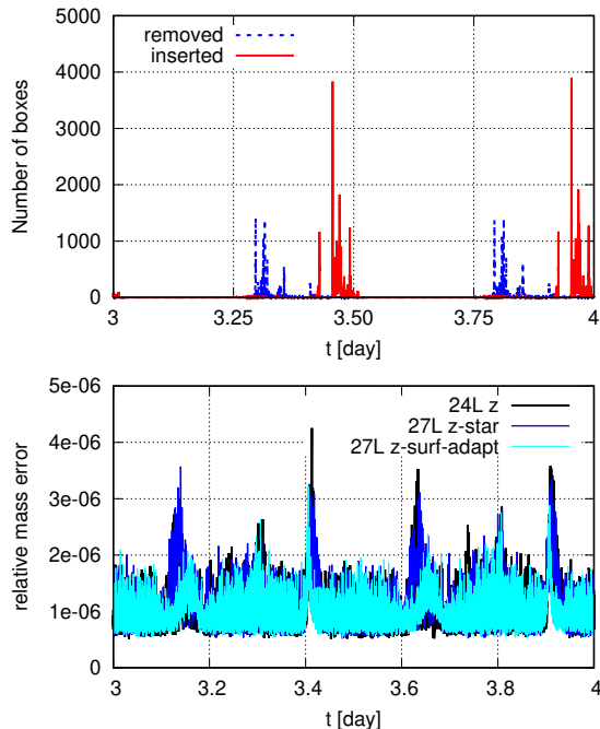
Figure 14. Po river. Top left: time evolution of the total number of layers inserted and removed per time step for the 24L z -surf-adapt simulation. Bottom left: relative mass conservation error for the dual cell. Right: relative tracer constancy error after 4 days.
