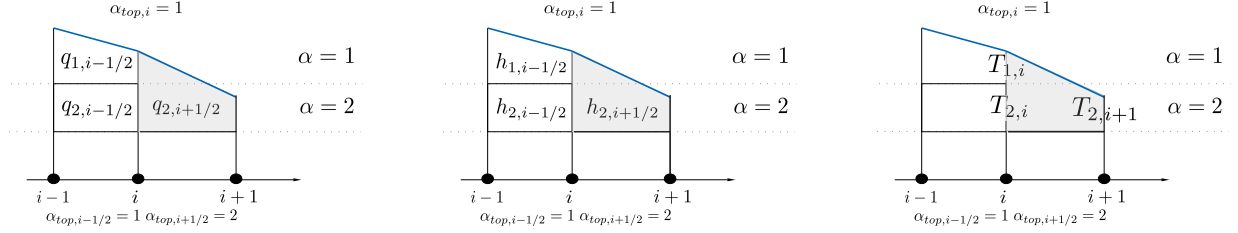
Figure 7. Non-conformal box for the one-dimensional case. The non-conformal box is in grey. Discharges, layer thickness and tracers are shown.
