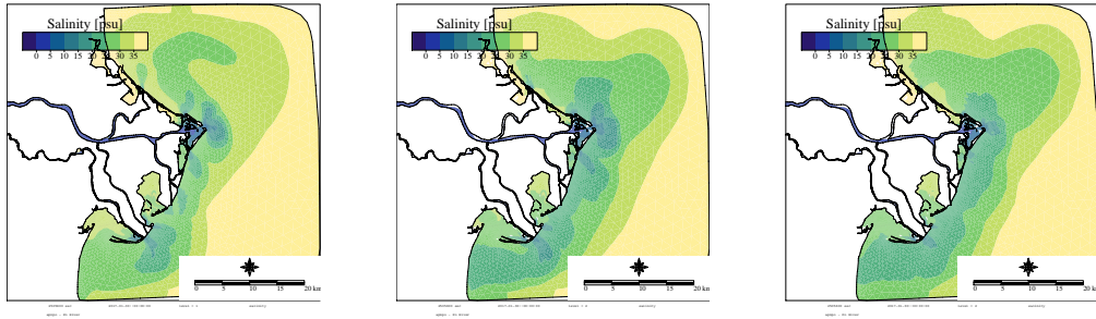
Figure 15. Po river. Minimum of the surface salinity (for the 24-layer grid the minimum is computed at the first layer, for the 27-layer grid at the second layer). Left: 24L z . Middle: 27L z —surf-adapt. Right: 27L z —star.
