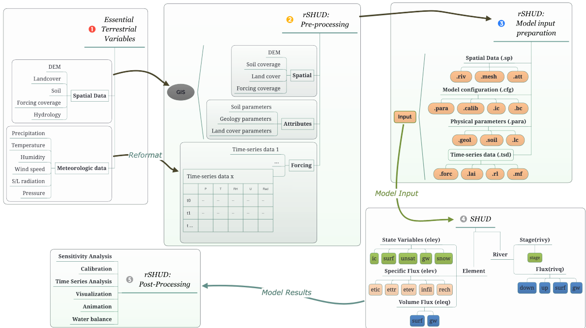
Figure 2. The general workflow of hydrological modeling and implementation of SHUD modeling system, which includes five steps: raw data accessing, pre-processing, building model
