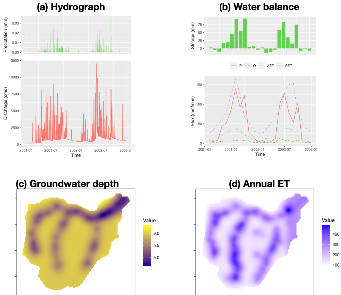
Figure 8. The result analysis of modeling Waerma Watershed; (a) hydrograph, (b) watershed scale water balance, (c) ground water depth [m], and (d) annual evaporation rate [mm/year].
